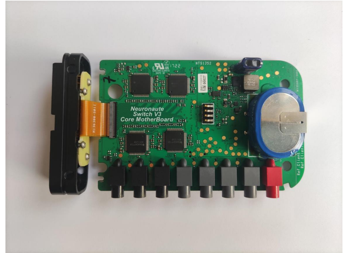
Bottom View
