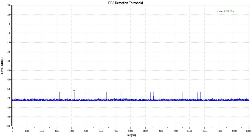
11AC40SISO_5310_Type5
