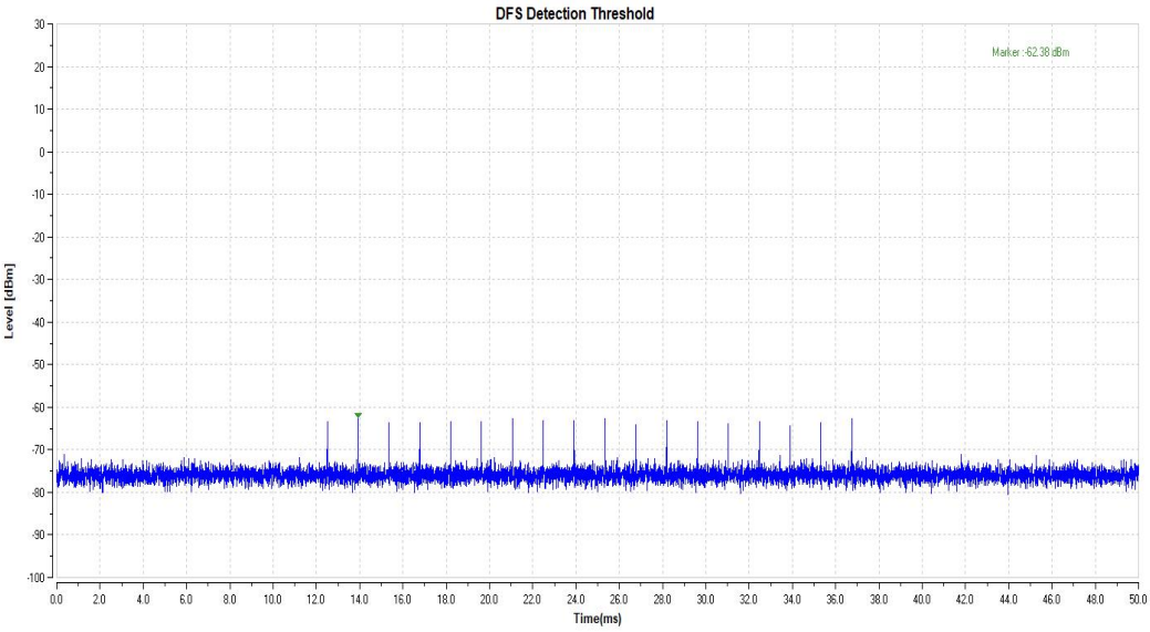
11AC40SISO_5310_Type0
