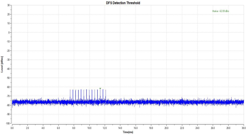
11AC20SISO_5320_Type4
