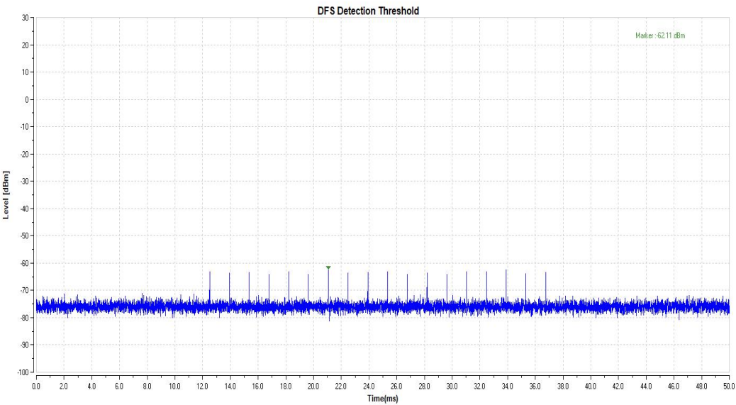
11AC20SISO_5500_Type1
