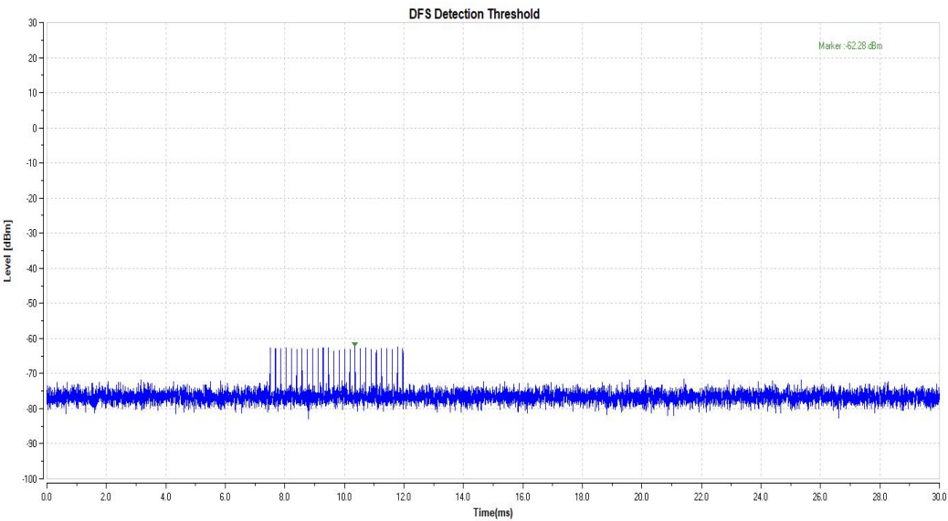
11AC20SISO_5320_Type3
