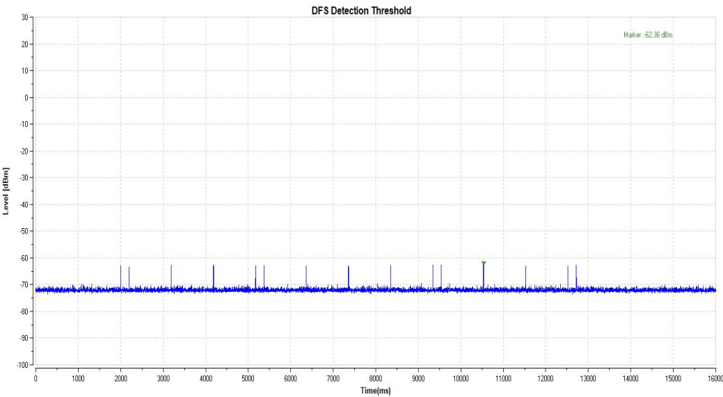
11AC20SISO_5500_Type6
