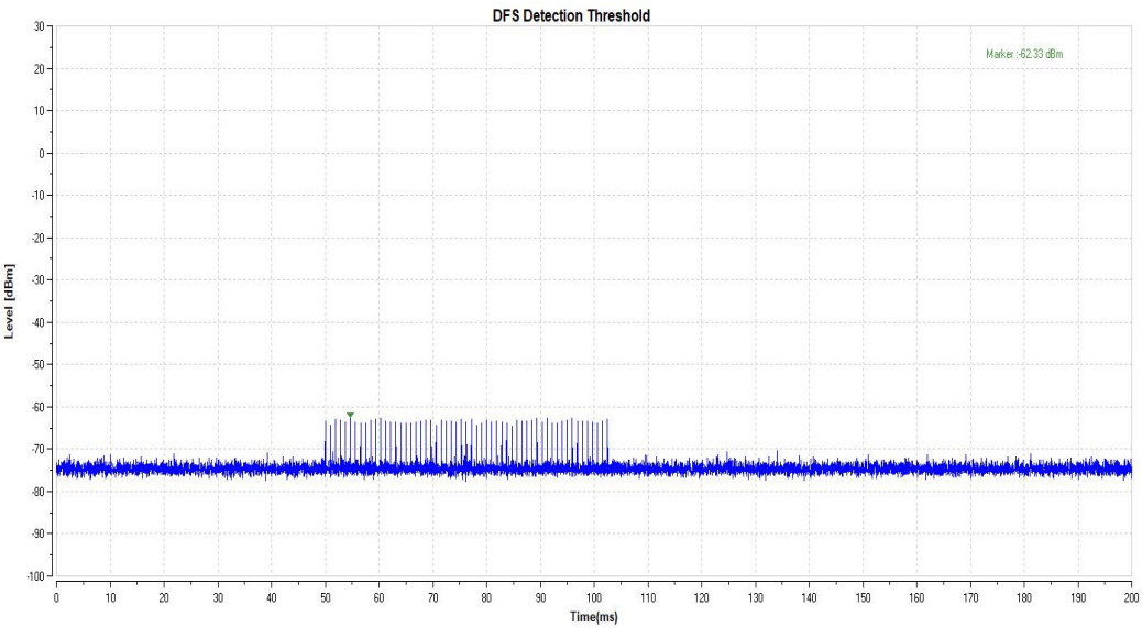
11AC20SISO_5500_Type2
