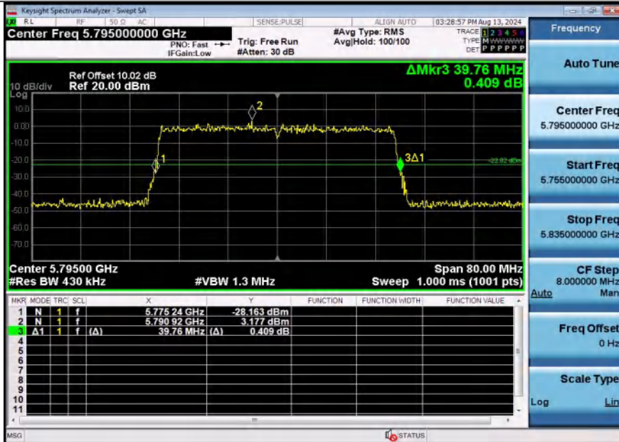
11AX40SISO-Ant2-5795
