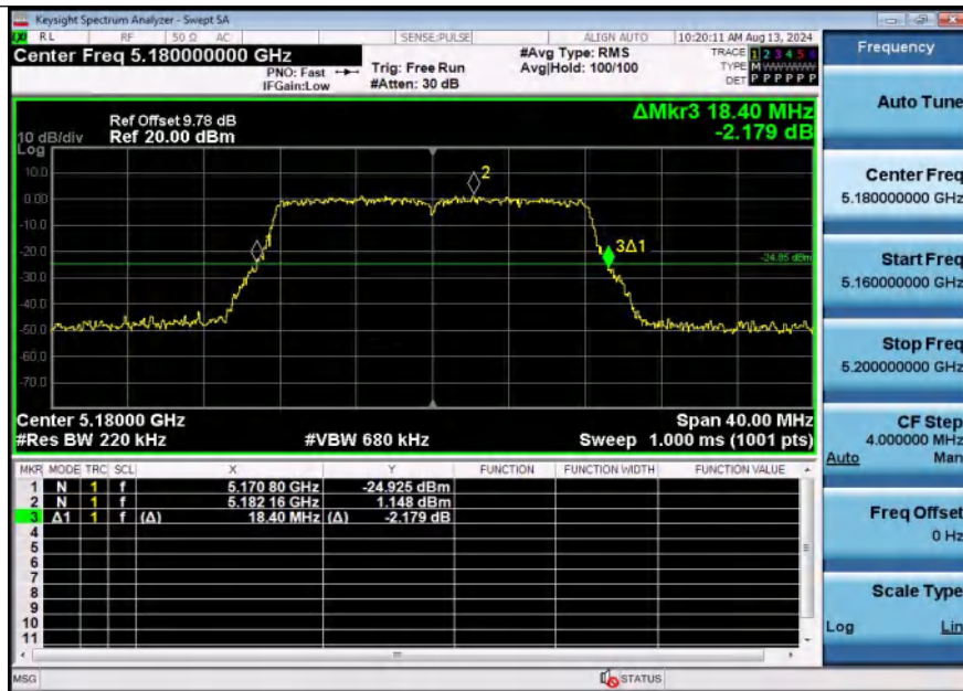
11A-Ant2-5180
