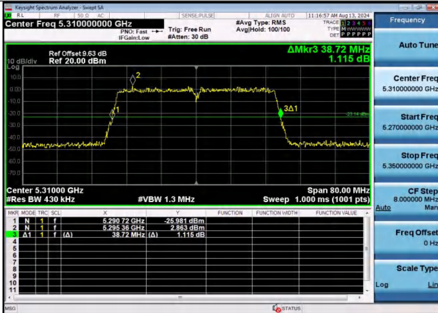
11N40SISO-Ant2-5310
