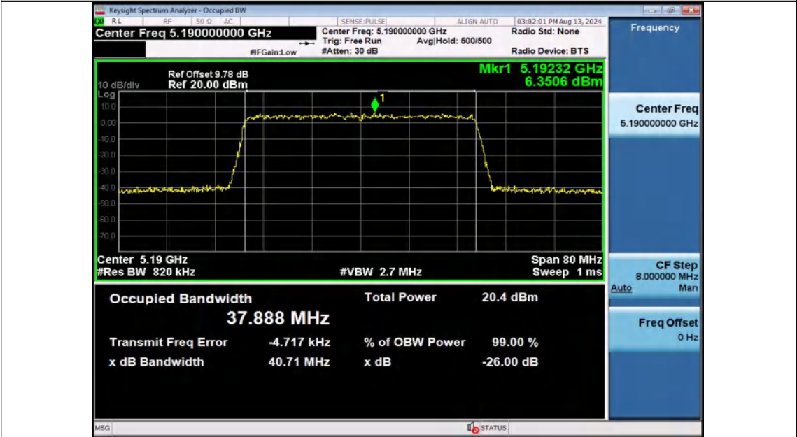
11AX40SISO-Ant2-5190
