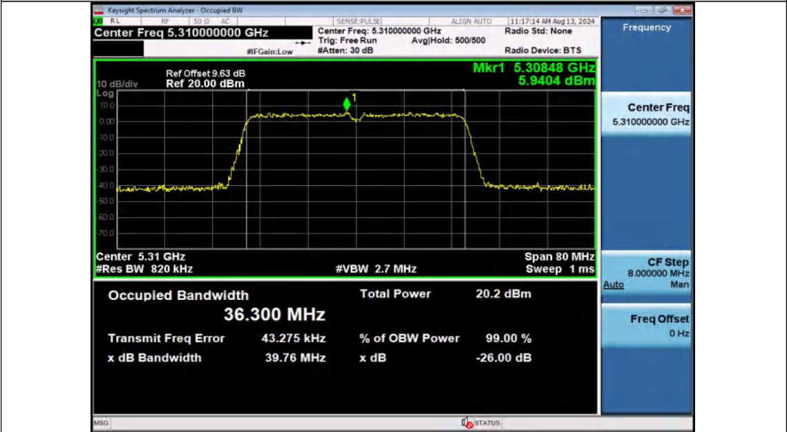
11N40SISO-Ant2-5310
