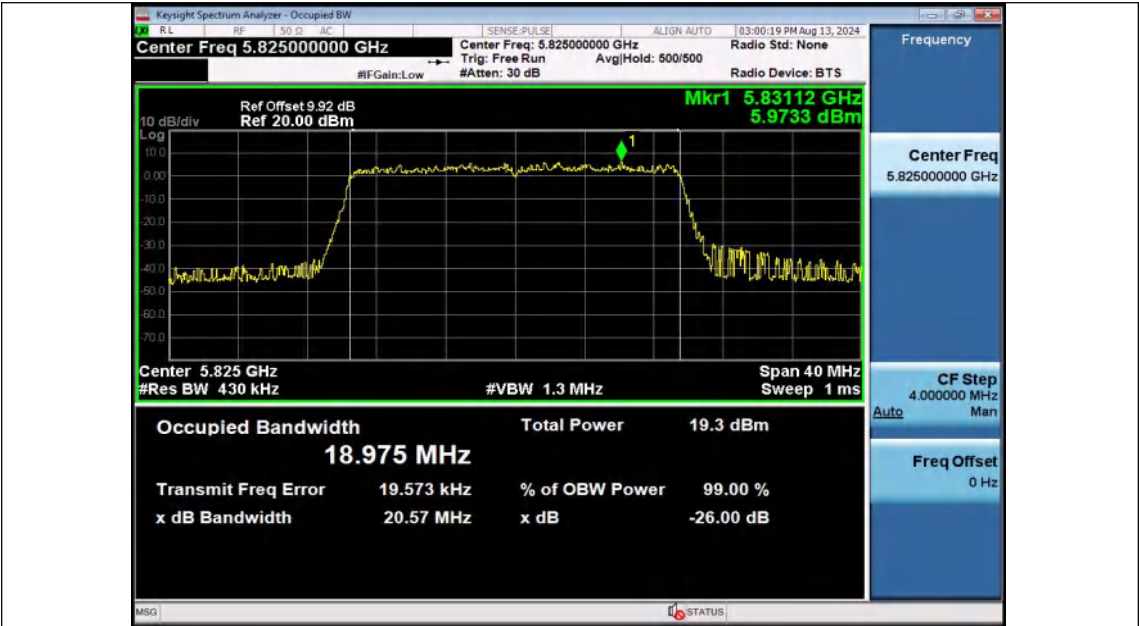
11AX20SISO-Ant2-5825
