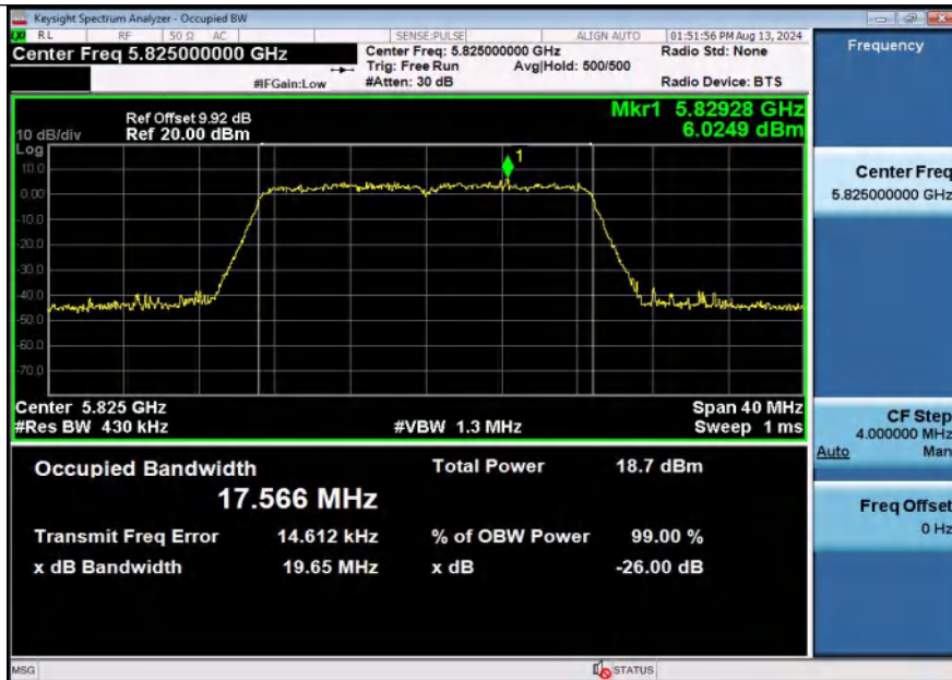
11AC20SISO-Ant2-5825
