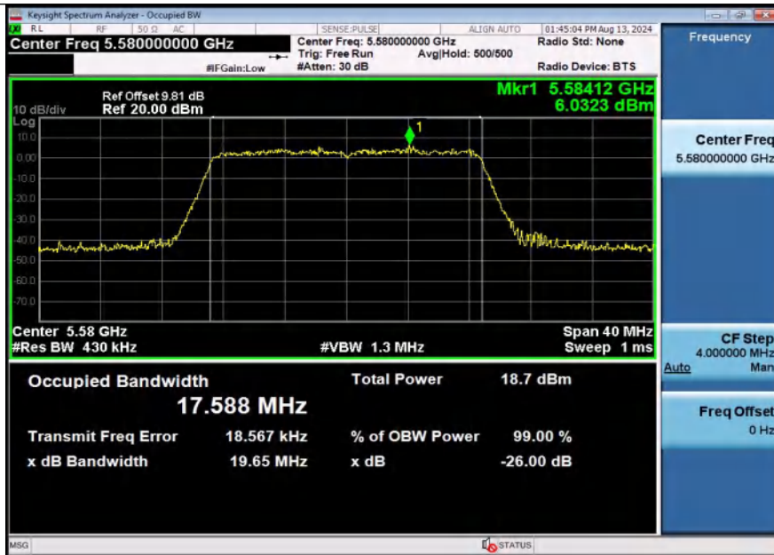
11AC20SISO-Ant2-5580
