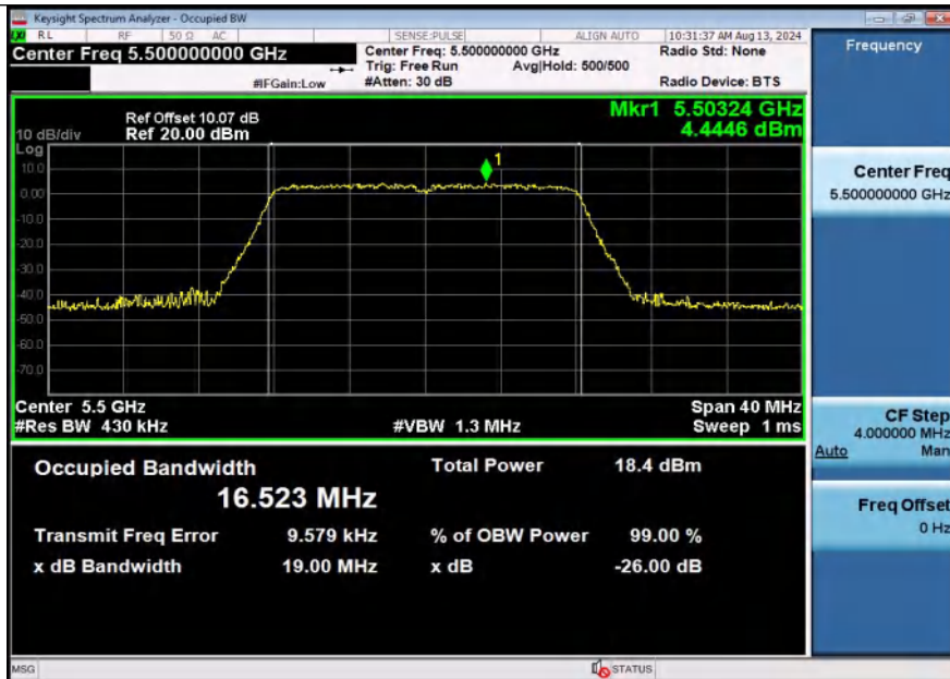
11A-Ant2-5500
