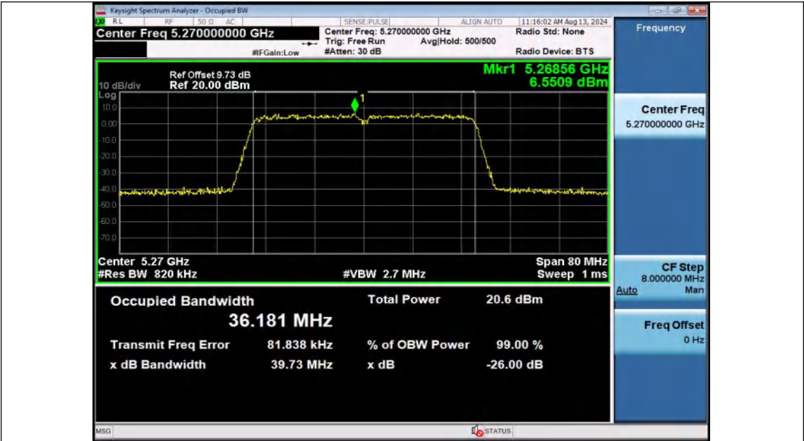
11N40SISO-Ant2-5270
