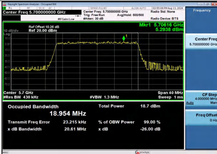
11AX20SISO-Ant2-5700
