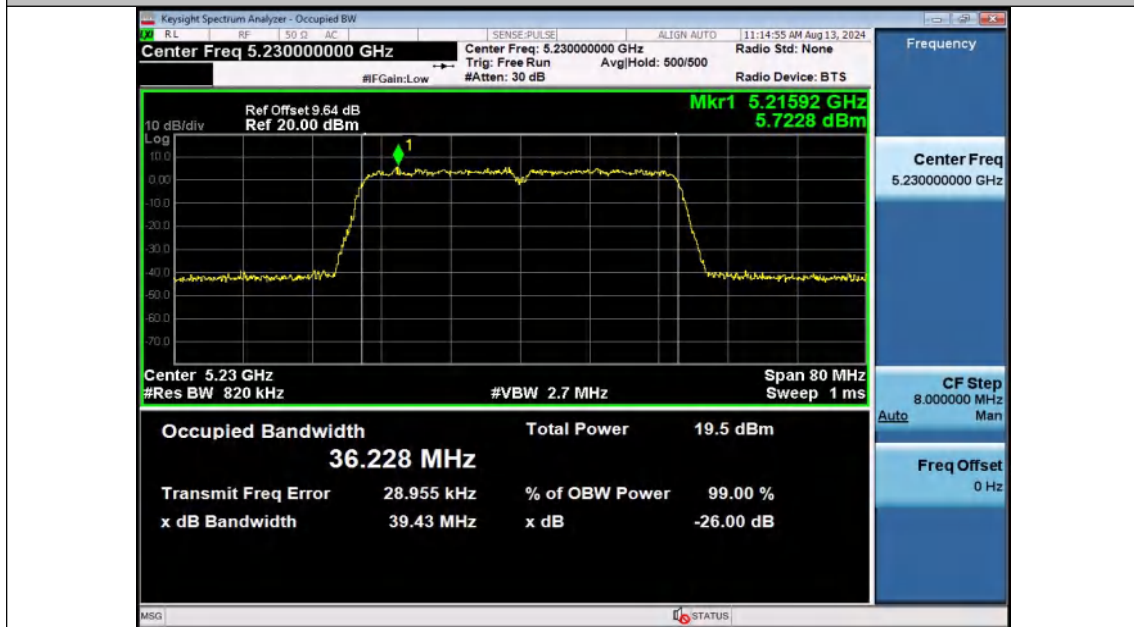
11N40SISO-Ant2-5230
