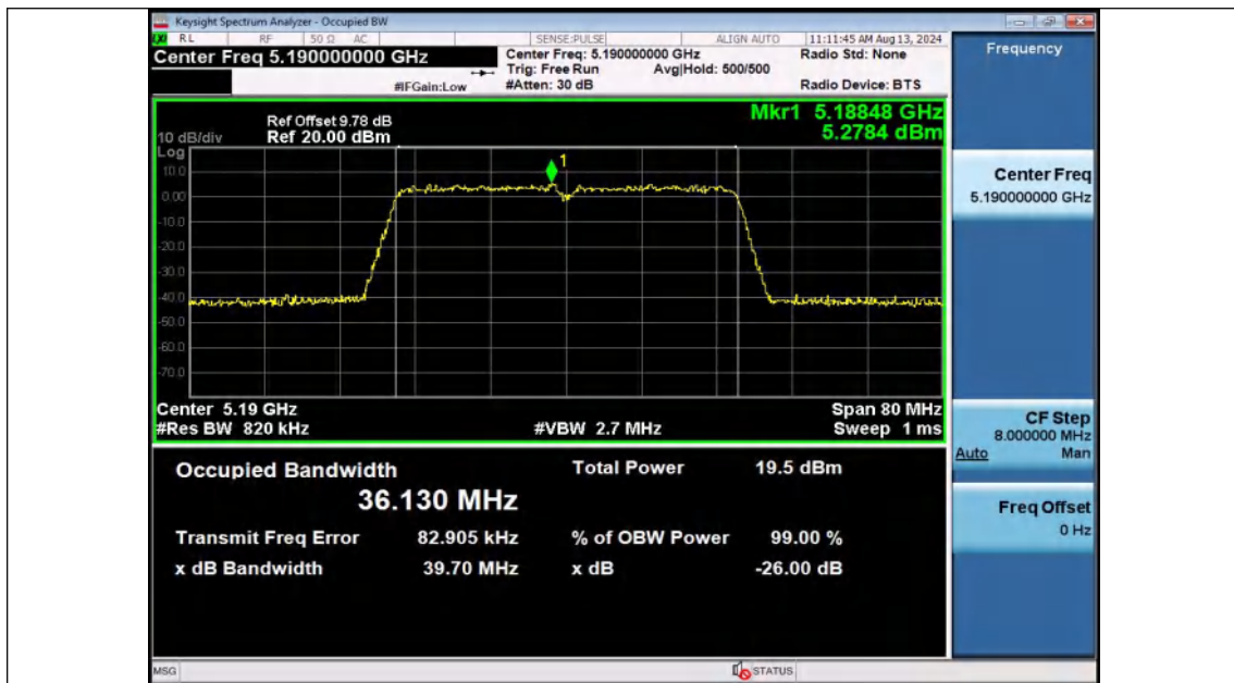
11N40SISO-Ant2-5190
