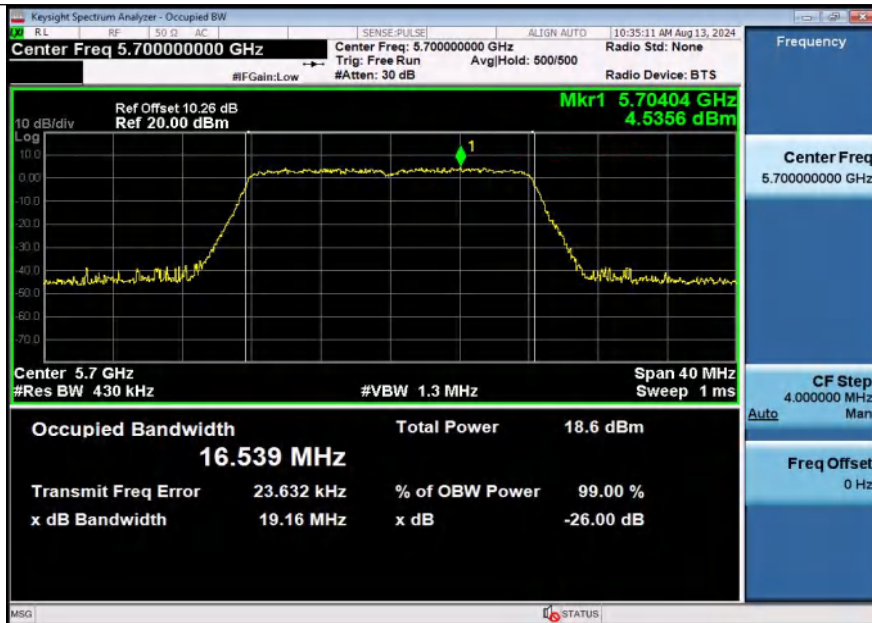
11A-Ant2-5700
