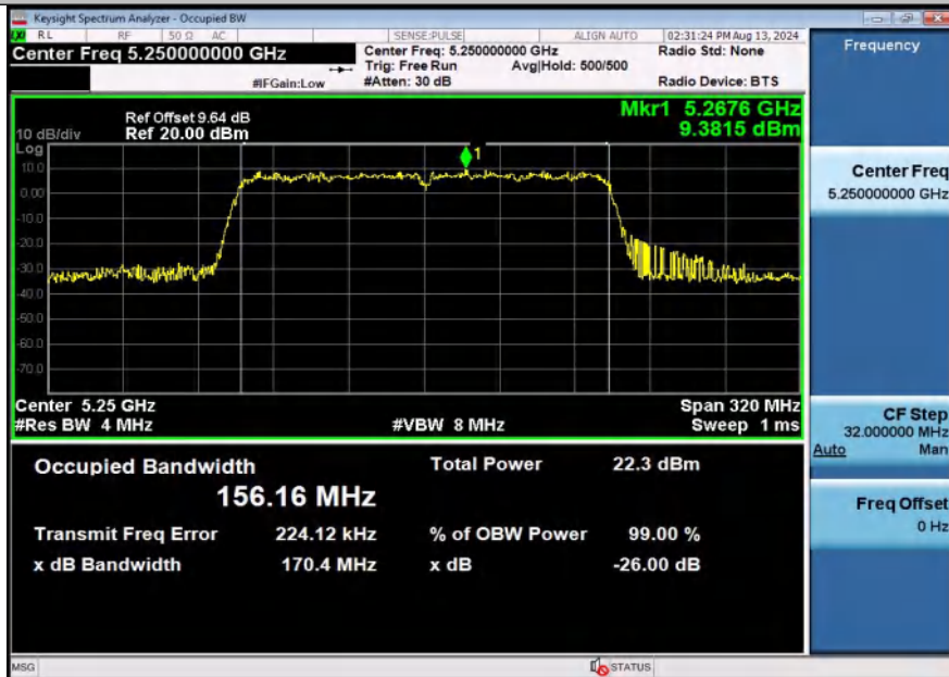
11AC160SISO-Ant2-5250
