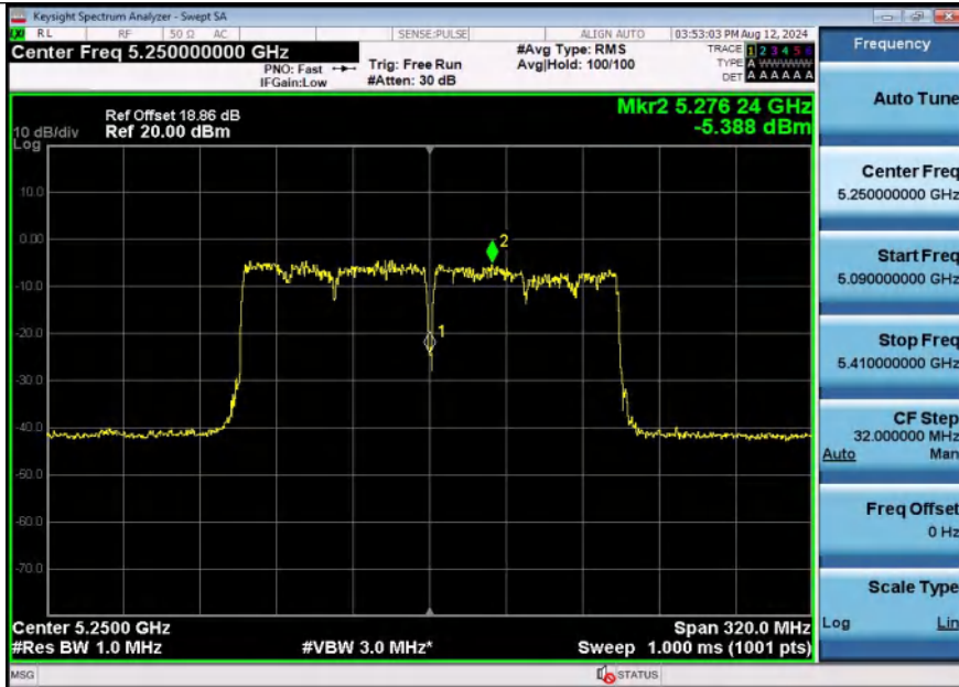
11AC160SISO-Ant1-5250_UNII-2A-PASS
