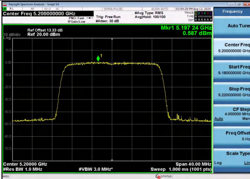
11AX20SISO-Ant1-5200-PASS
