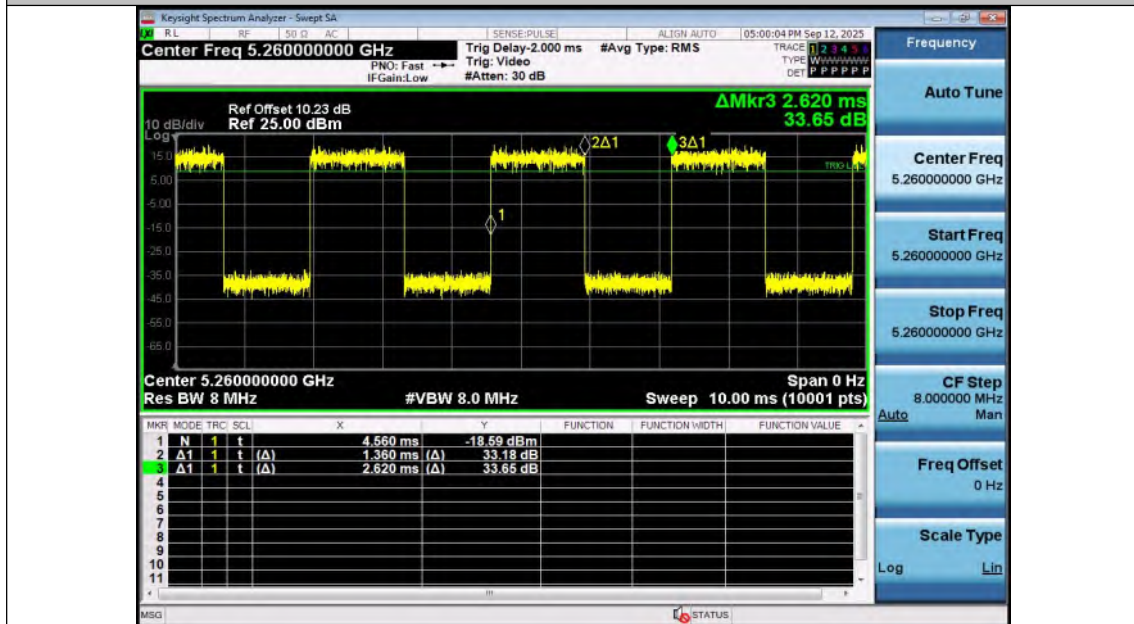
NTNV-11A-Ant2-5260
