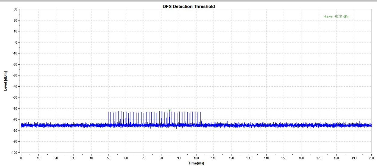
11AX80-5290-Type1-PASS
