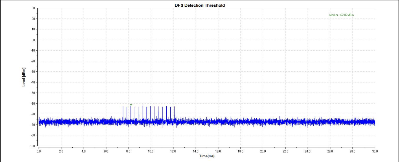
11AX40-5510-Type4-PASS
