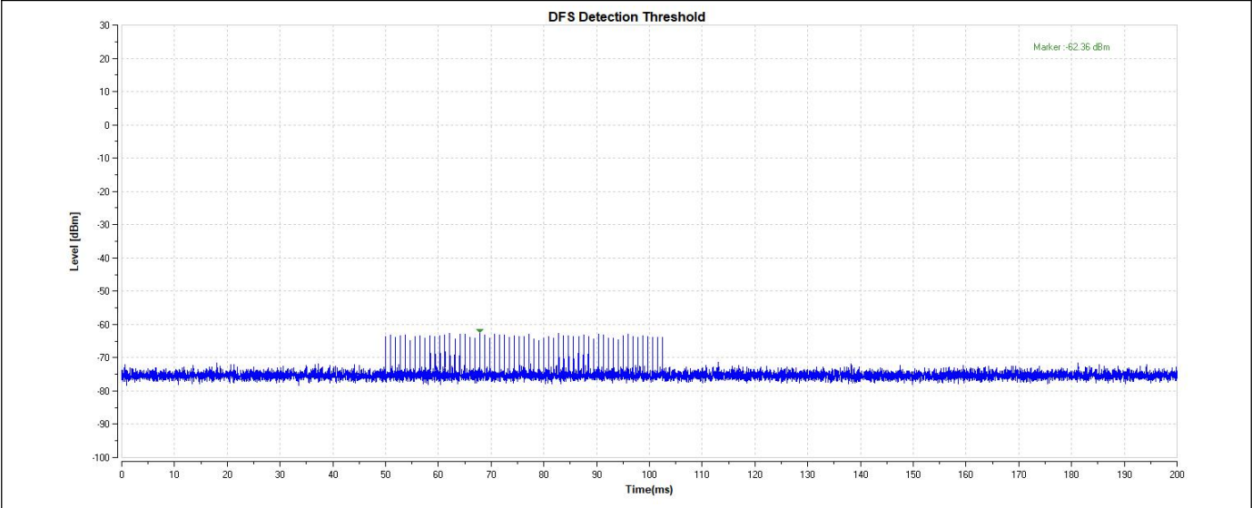
11AX160-5250-Type1-PASS
