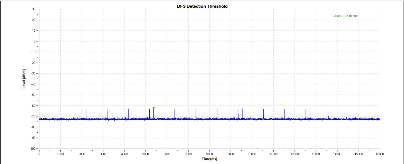
11AX80-5290-Type5-PASS
