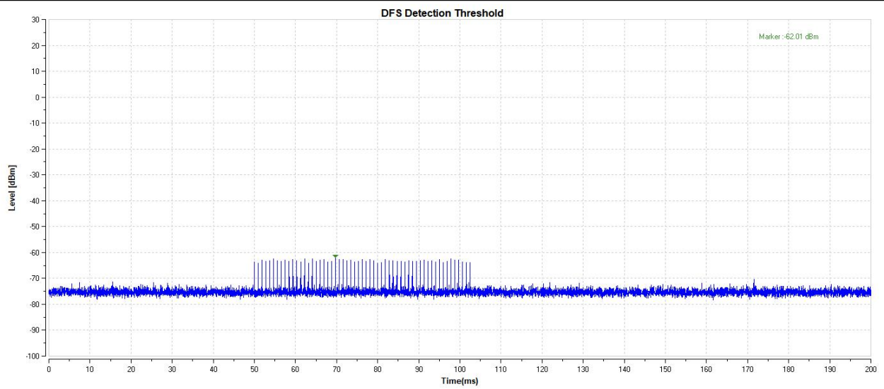
11AX40-5510-Type1-PASS
