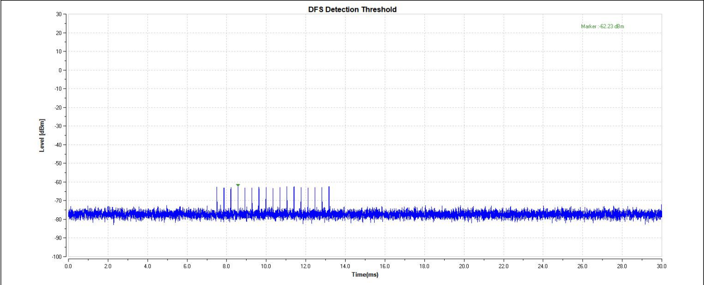
11AX20-5500-Type3-PASS
