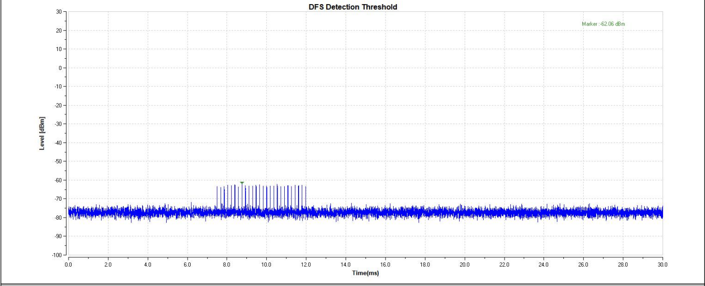
11AX20-5260-Type2-PASS
