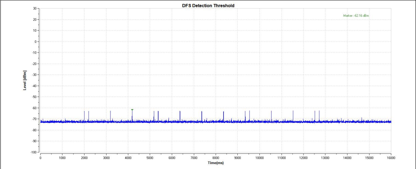
11AX80-5530-Type5-PASS
