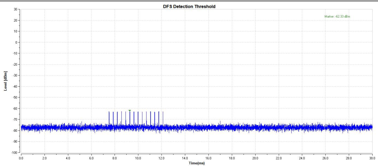
11AX80-5290-Type4-PASS
