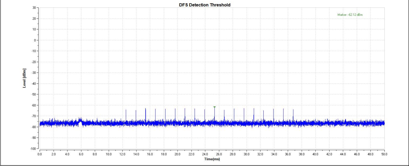
11AX80-5530-Type0-PASS
