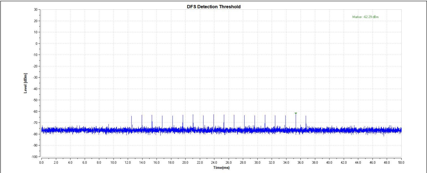
11AX160-5250-Type0-PASS
