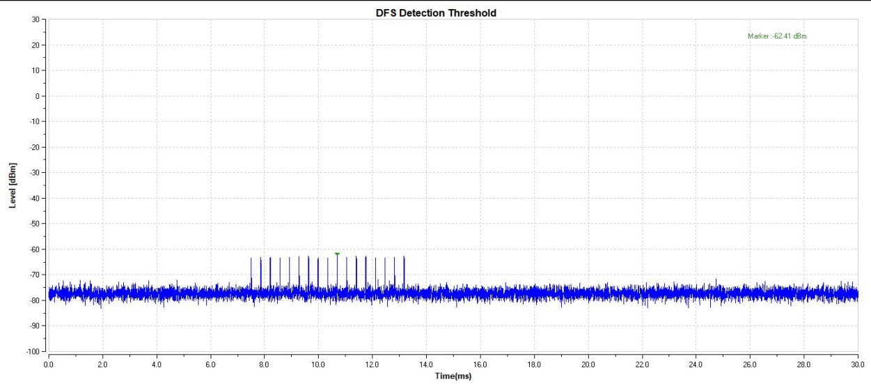
11AX80-5290-Type3-PASS
