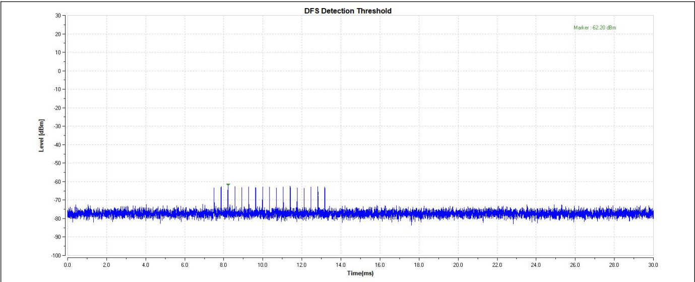
11AX160-5250-Type3-PASS
