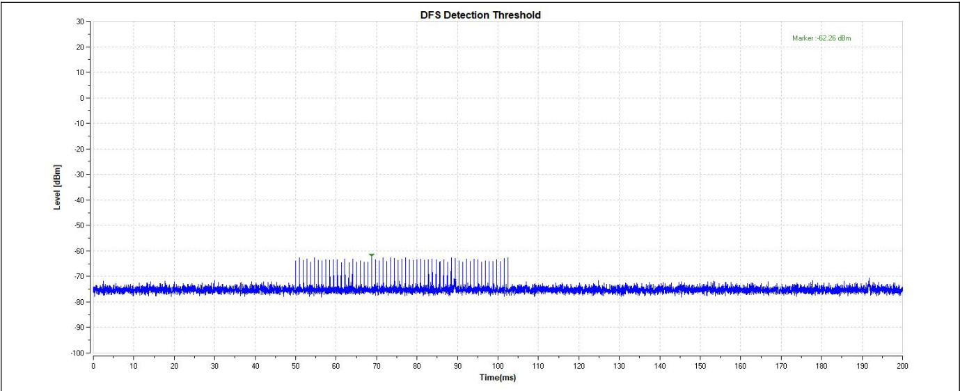
11AX80-5530-Type1-PASS
