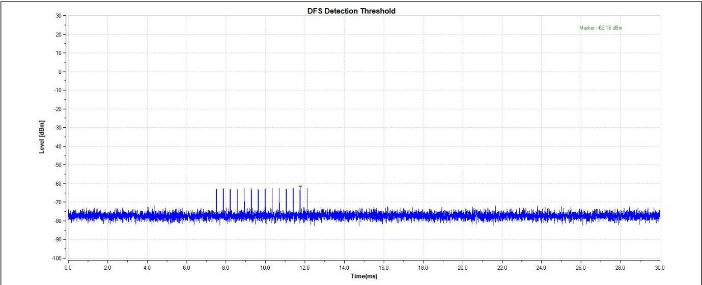
11AX80-5530-Type4-PASS
