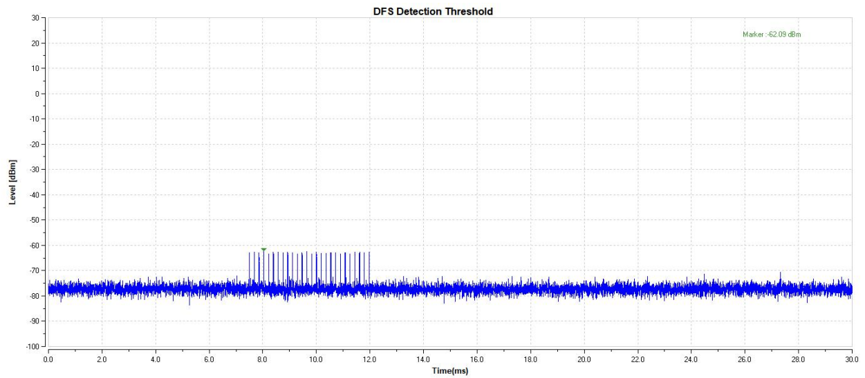
11AX80-5290-Type2-PASS
