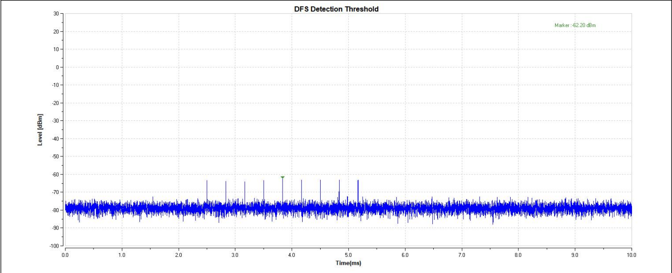
11AX80-5290-Type6-PASS
