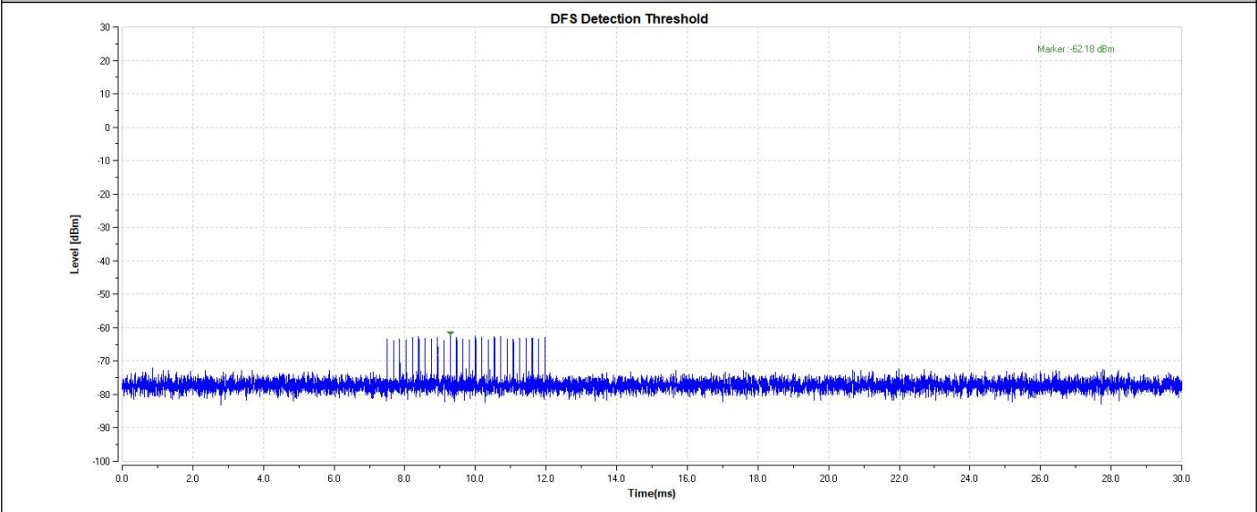
11AX80-5530-Type2-PASS
