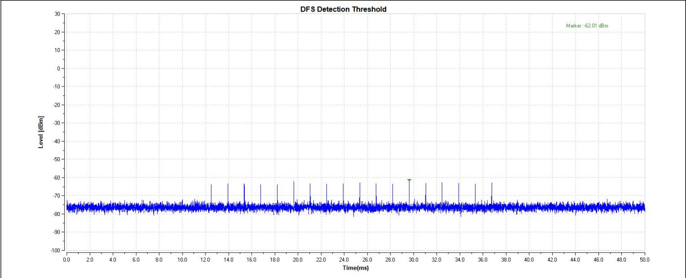
11AX160-5570-Type0-PASS
