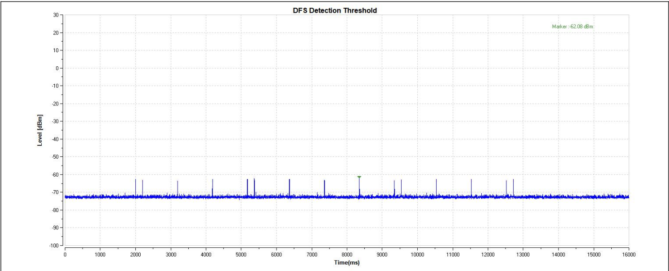
11AX20-5500-Type5-PASS
