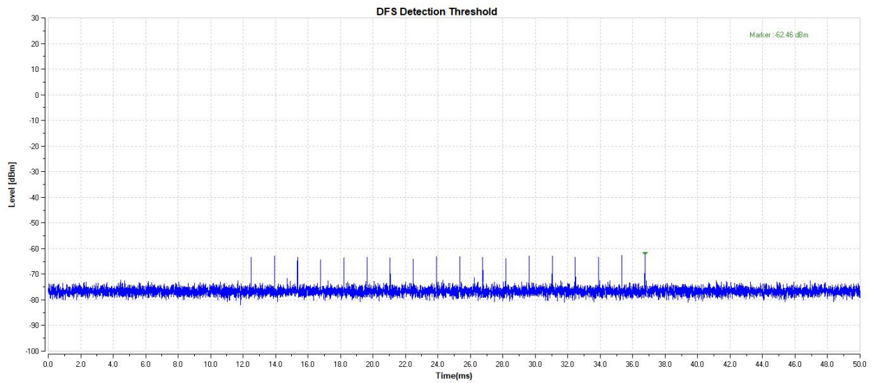
11AX40-5510-Type0-PASS
