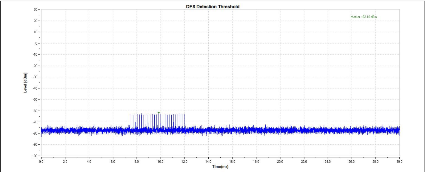
11AX20-5500-Type2-PASS
