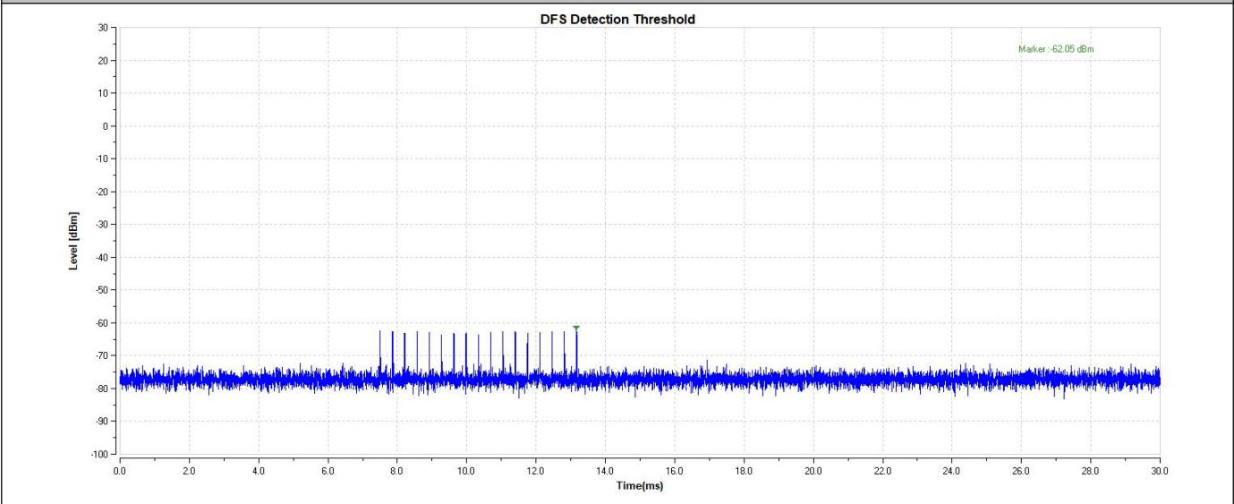
11AX80-5530-Type3-PASS
