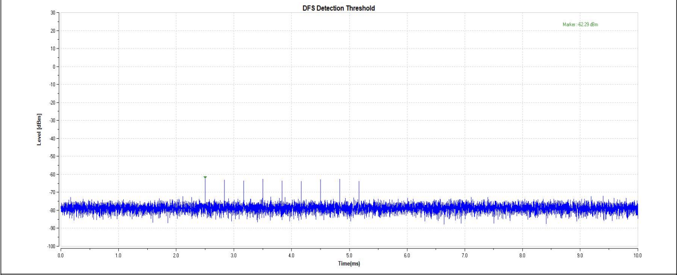
11AX80-5530-Type6-PASS
