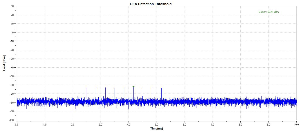
11AX40-5510-Type6-PASS
