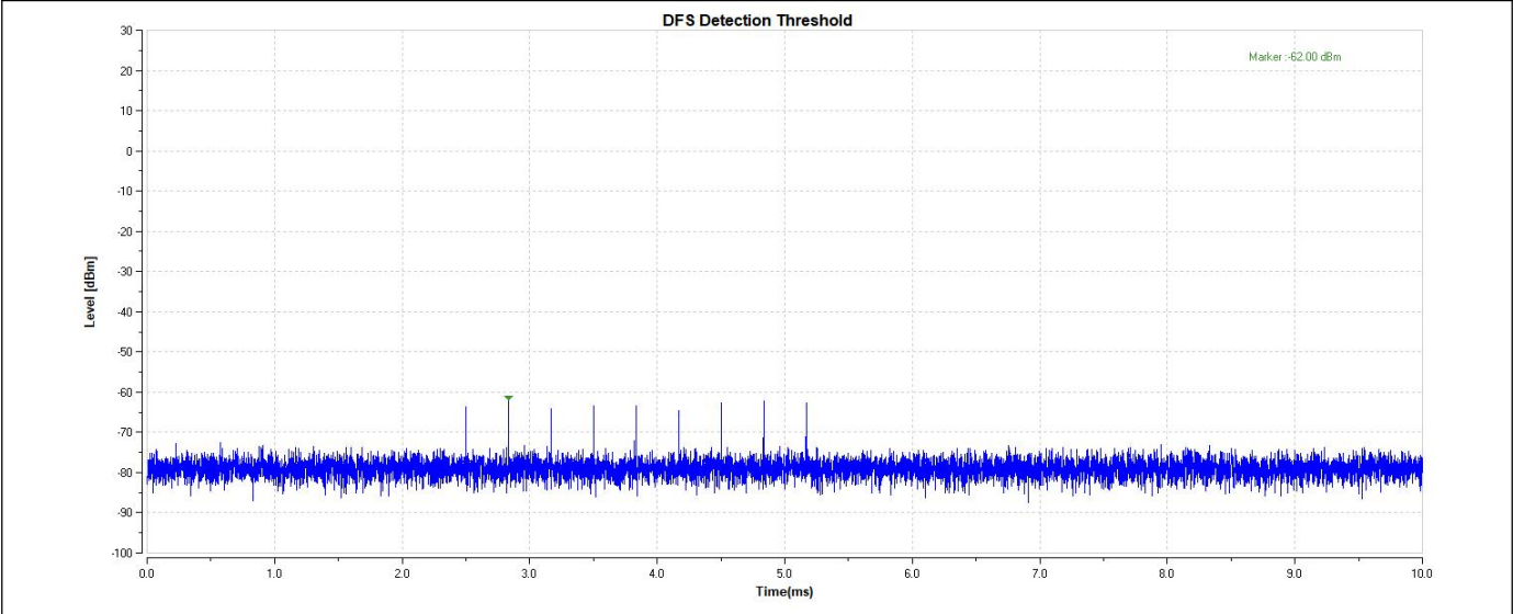
11AX20-5500-Type6-PASS
