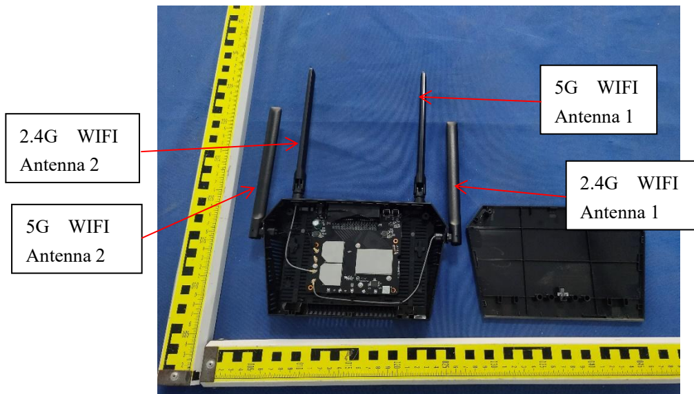
Enclosure 2
