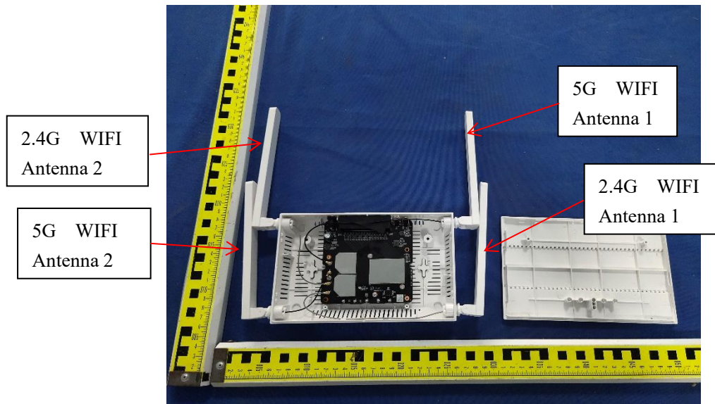
Enclosure 1
