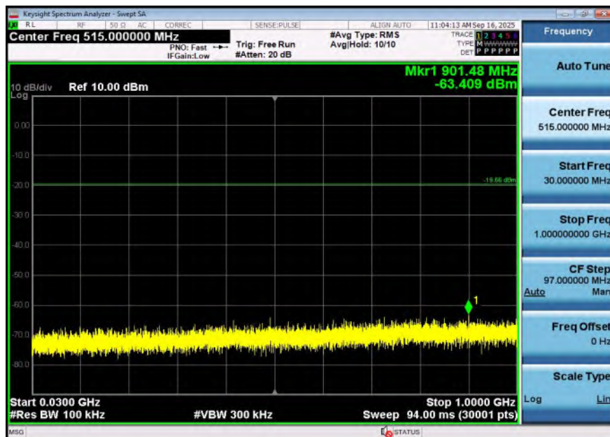
11B-Ant2-2412-30~1000-PASS
