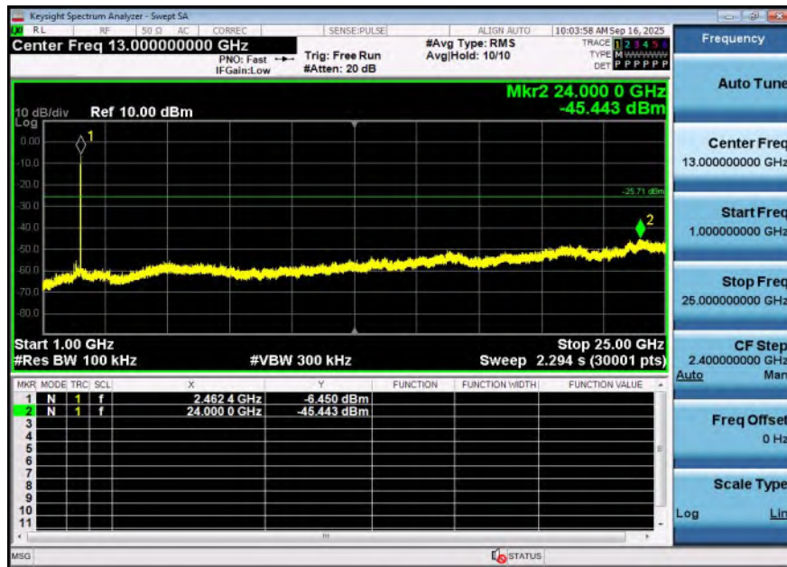
11AX20SISO-Ant1-2462-1000~25000-PASS
