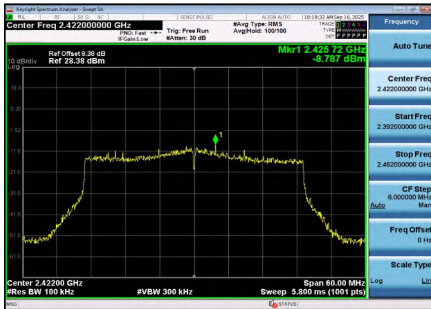
11AX40SISO-Ant1-2422-0~Reference-PASS
