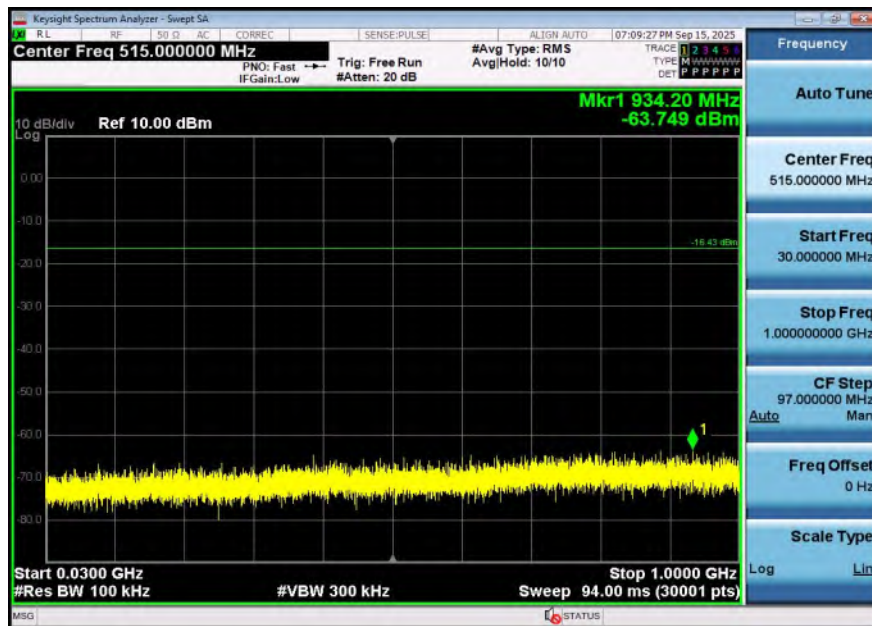
11B-Ant1-2462-30~1000-PASS
