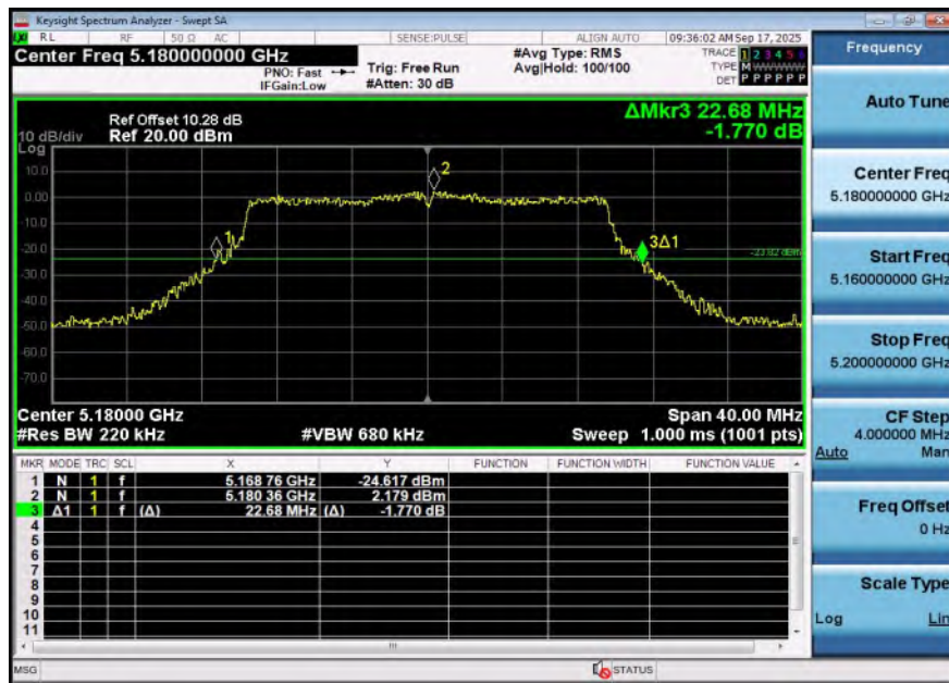
11AX20SISO-Ant1-5180
