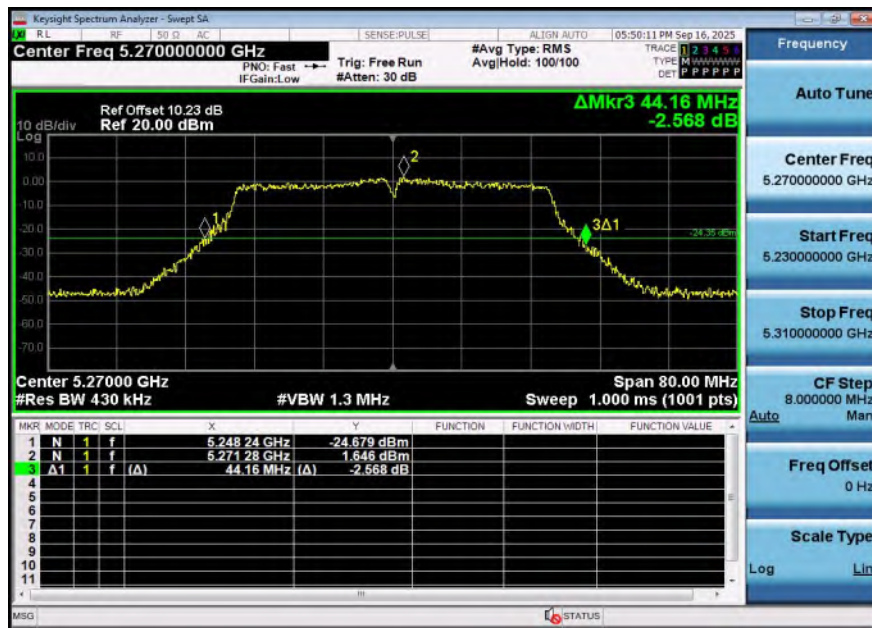
11AC40SISO-Ant1-5270
