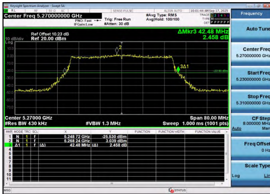
11AX40SISO-Ant1-5270
