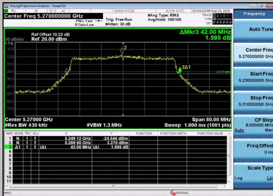
11BE40SISO-Ant1-5270
