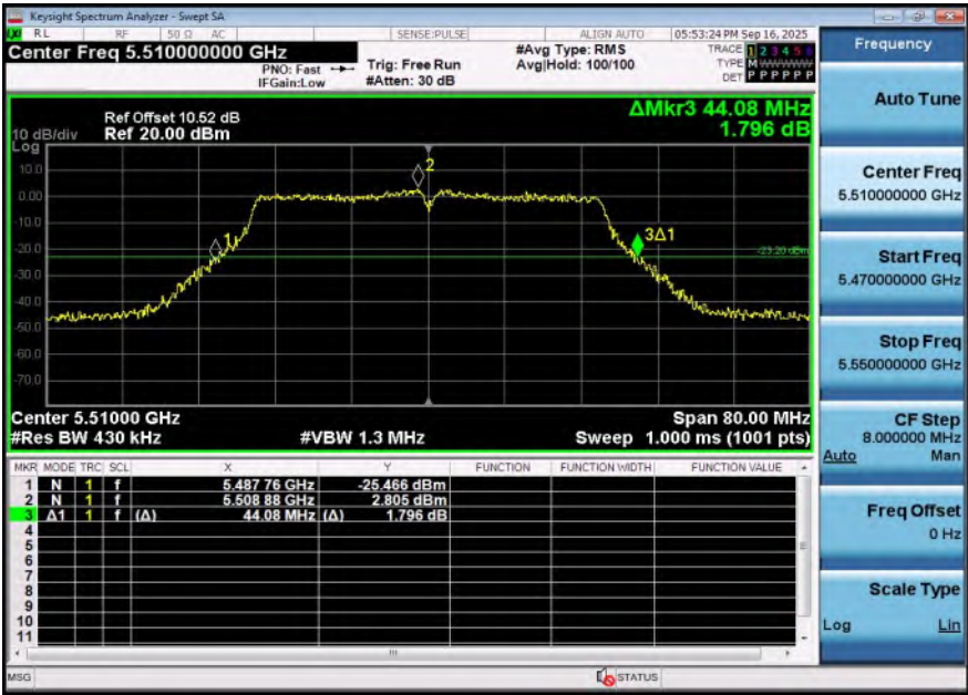
11AC40SISO-Ant1-5510
