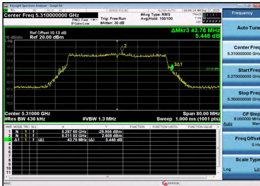
11AX40SISO-Ant1-5310
