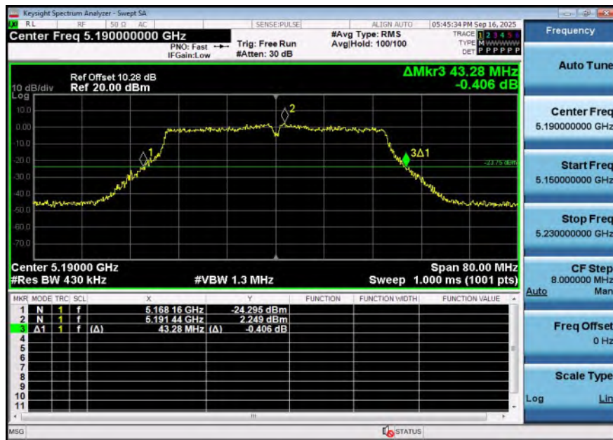
11AC40SISO-Ant1-5190
