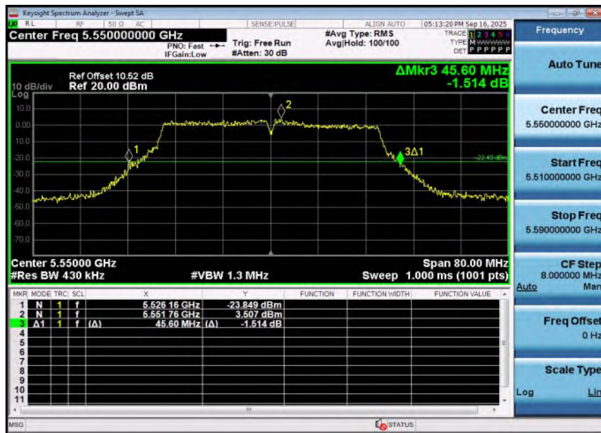
11N40SISO-Ant1-5550
