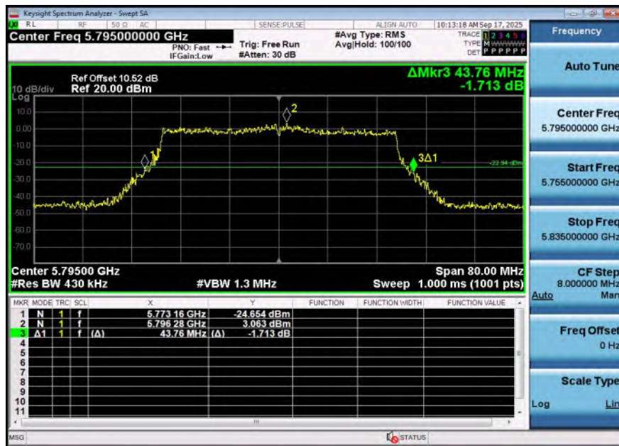
11AX40SISO-Ant1-5795
