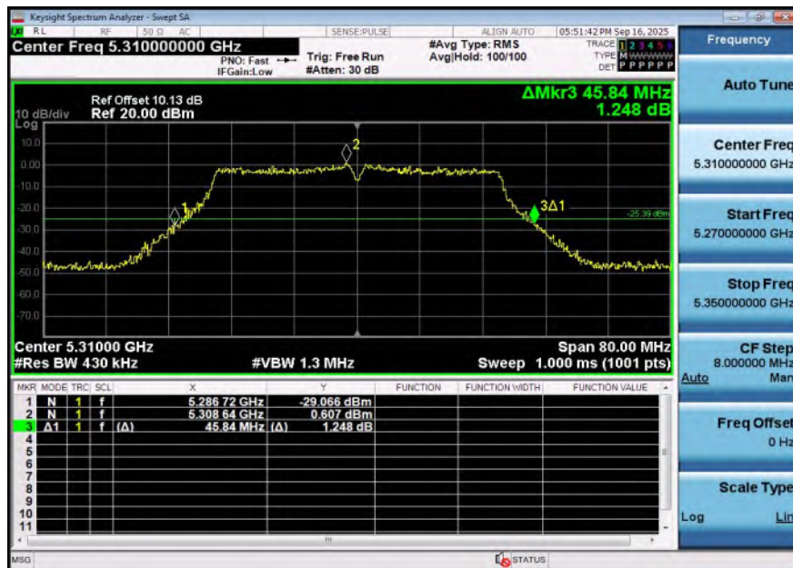
11AC40SISO-Ant1-5310
