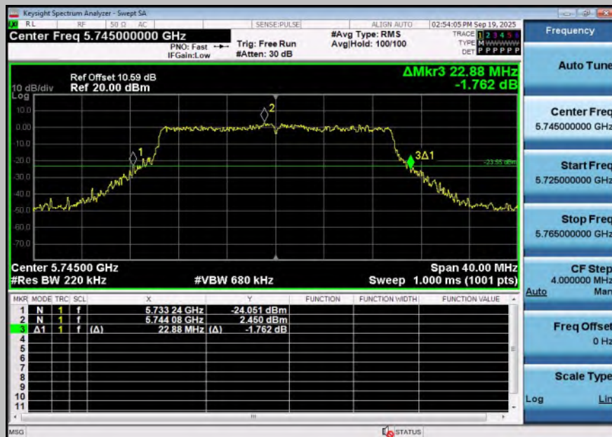
11BE20SISO-Ant1-5745
