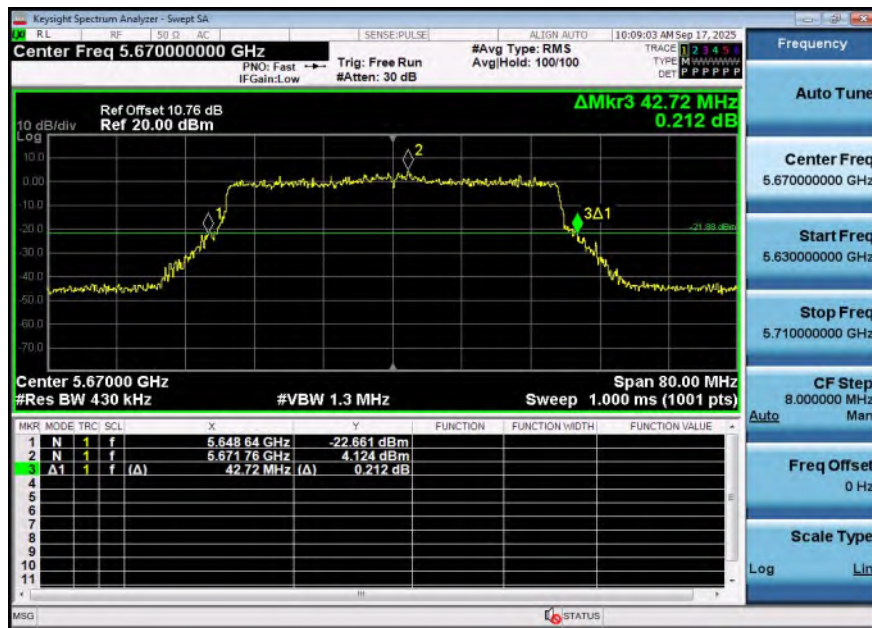
11AX40SISO-Ant1-5670
