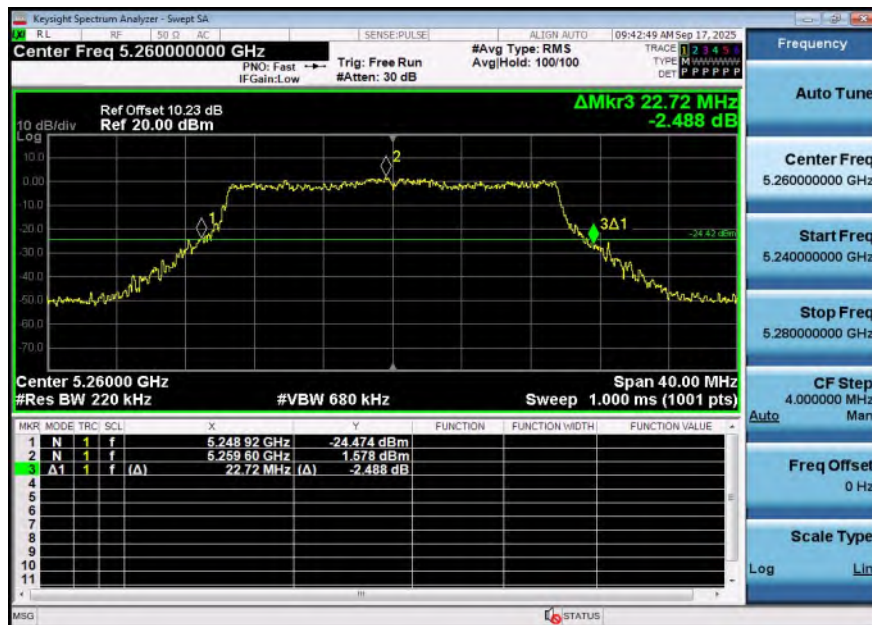
11AX20SISO-Ant1-5260
