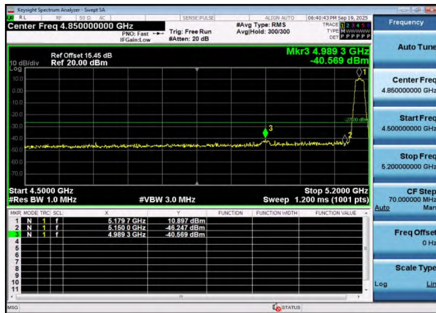
11AC20SISO-Ant2-5180-PASS
