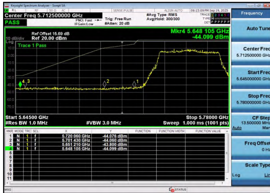
11AX40SISO-Ant1-5755-PASS
