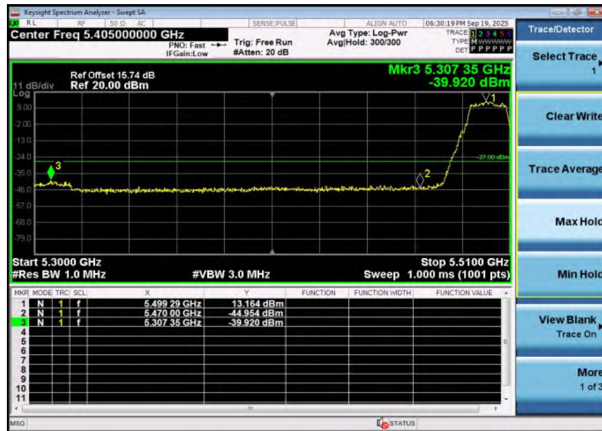
11A-Ant2-5500-PASS
