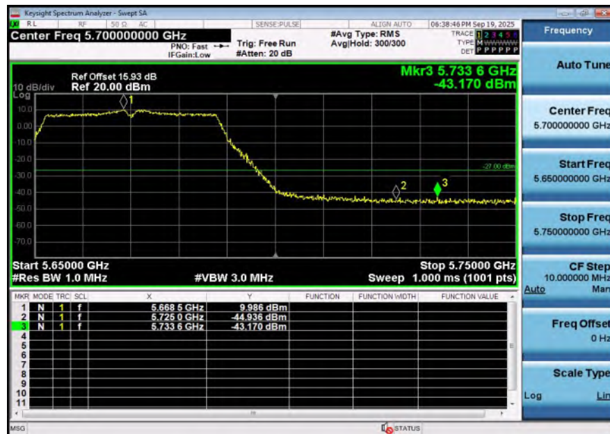
11N40SISO-Ant2-5670-PASS
