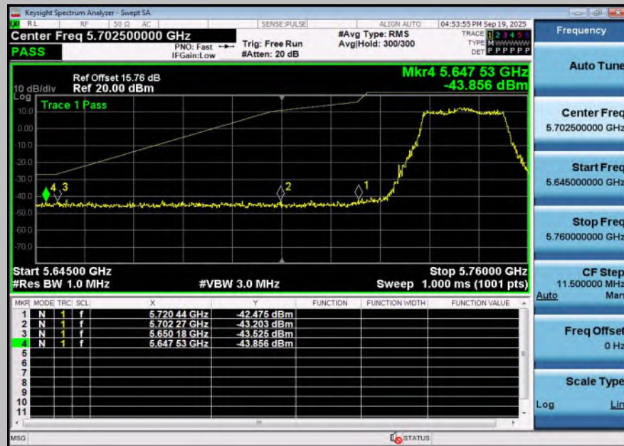
11BE20SISO-Ant1-5745-PASS
