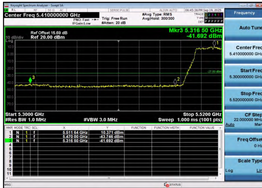
11AC40SISO-Ant2-5510-PASS
