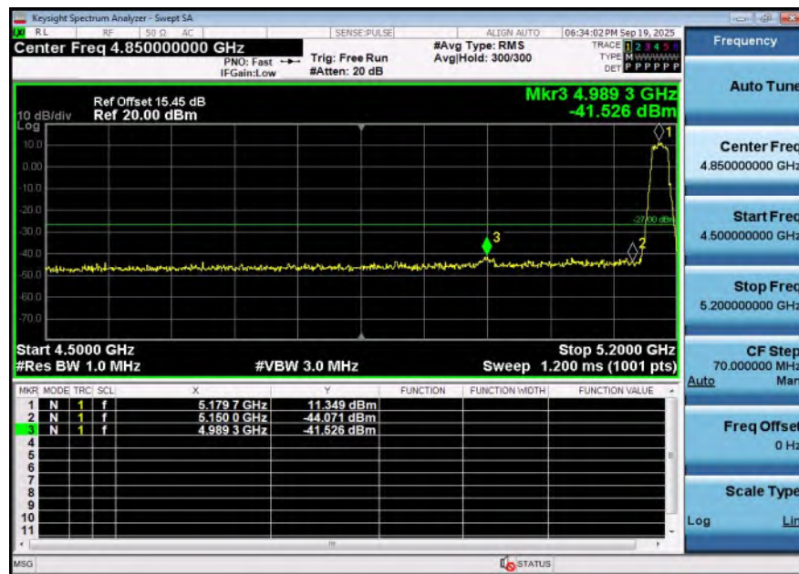
11N20SISO-Ant2-5180-PASS
