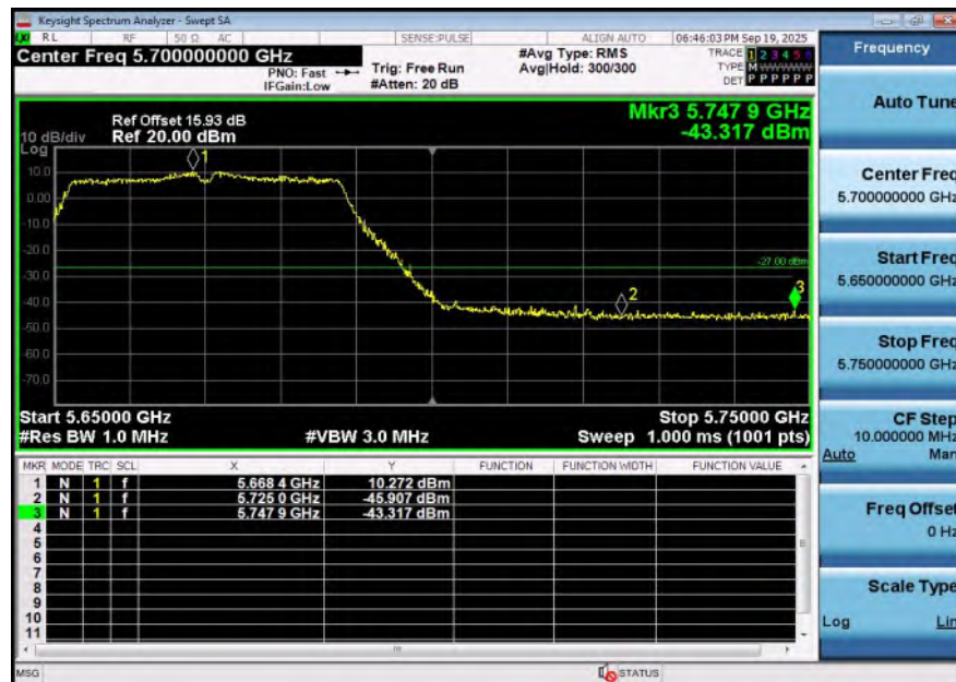
11AC40SISO-Ant2-5670-PASS
