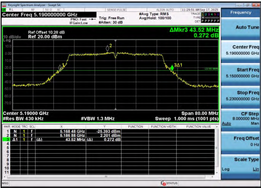
11N40SISO-Ant2-5190
