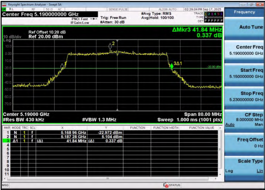
11AX40SISO-Ant2-5190
