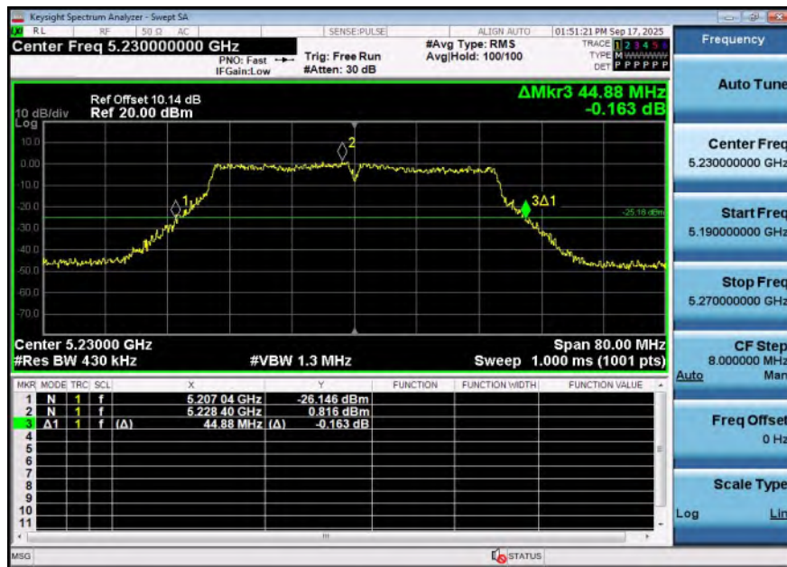
11AC40SISO-Ant2-5230
