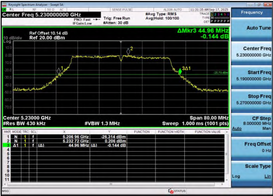
11N40SISO-Ant2-5230
