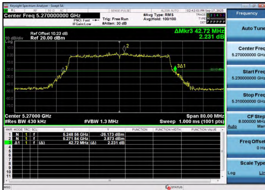
11AX40SISO-Ant2-5270
