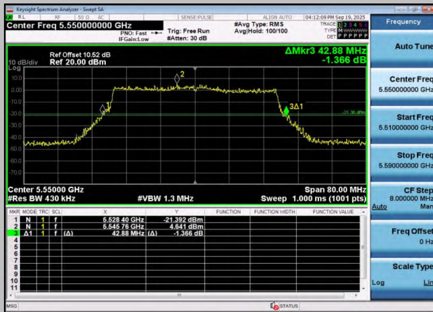
11BE40SISO-Ant2-5550
