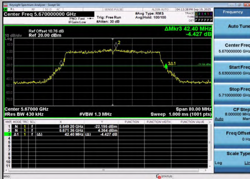
11BE40SISO-Ant2-5670
