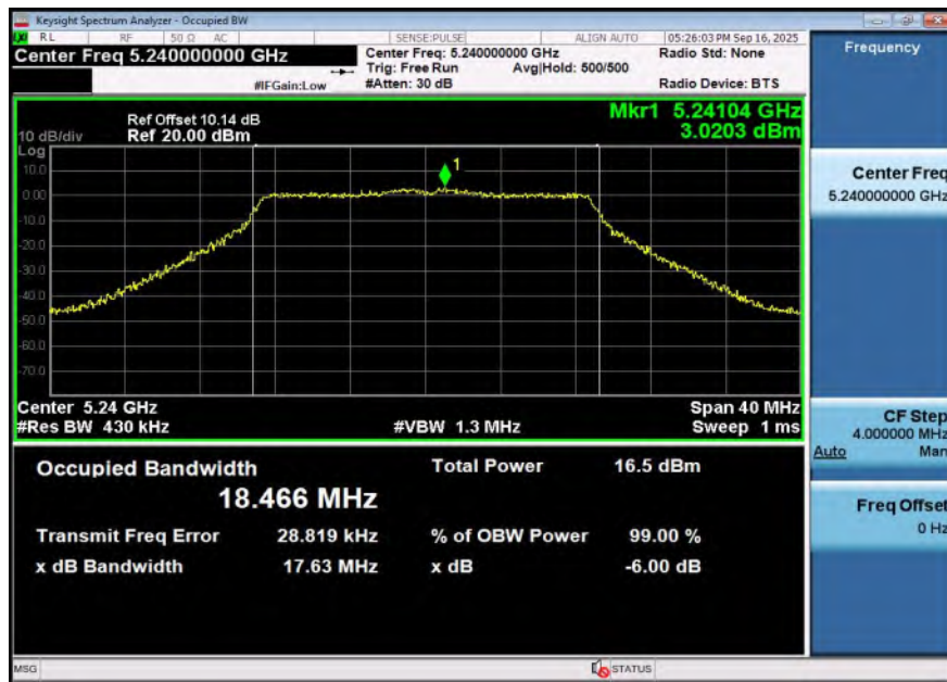
11AC20SISO-Ant1-5240
