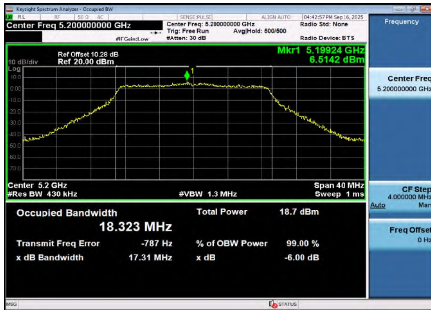
11N20SISO-Ant1-5200
