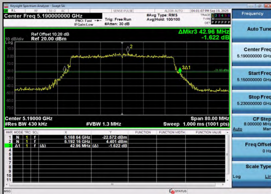
11BE40SISO-Ant2-5190
