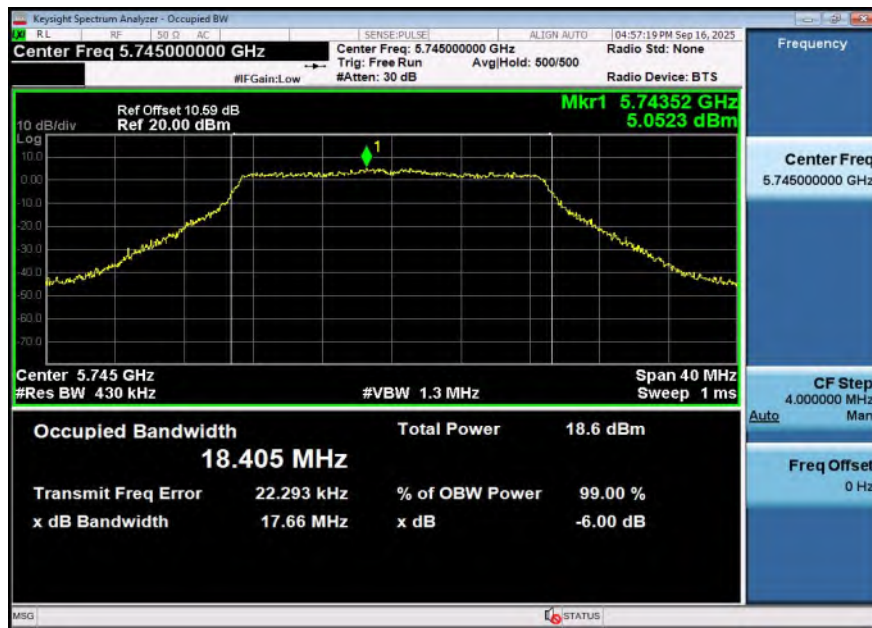
11N20SISO-Ant1-5745
