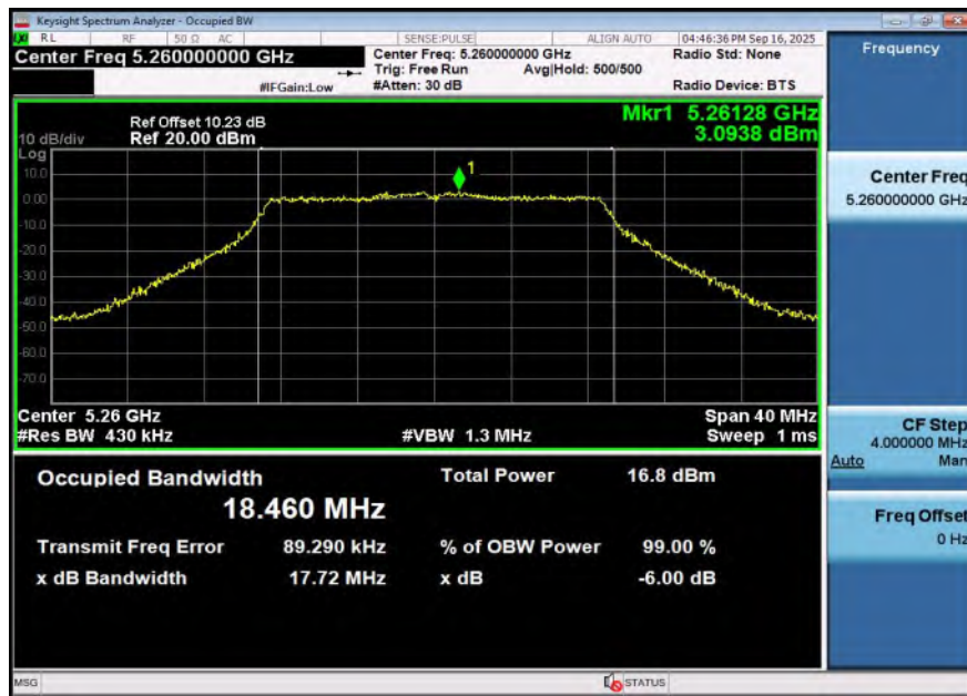
11N20SISO-Ant1-5260
