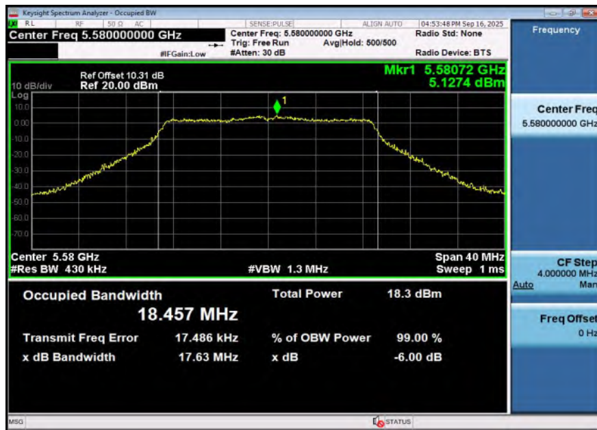
11N20SISO-Ant1-5580
