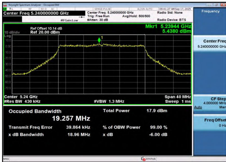
11AX20SISO-Ant1-5240
