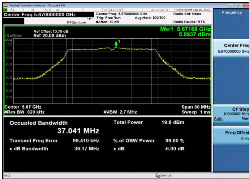
11AC40SISO-Ant1-5670
