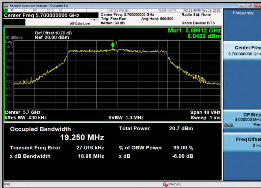
11BE20SISO-Ant1-5700
