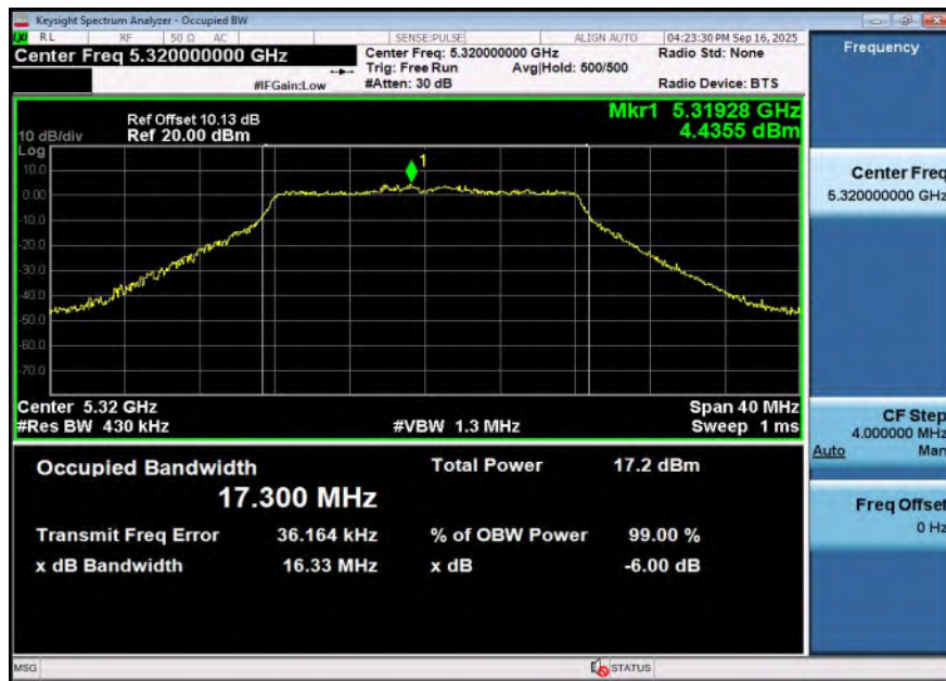
11A-Ant1-5320
