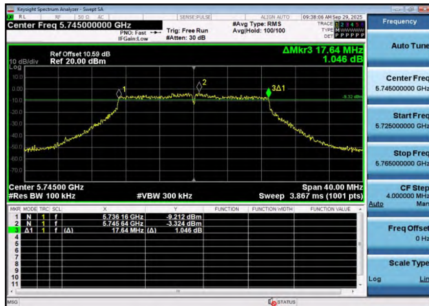
11N20SISO-Ant2-5745-PASS
