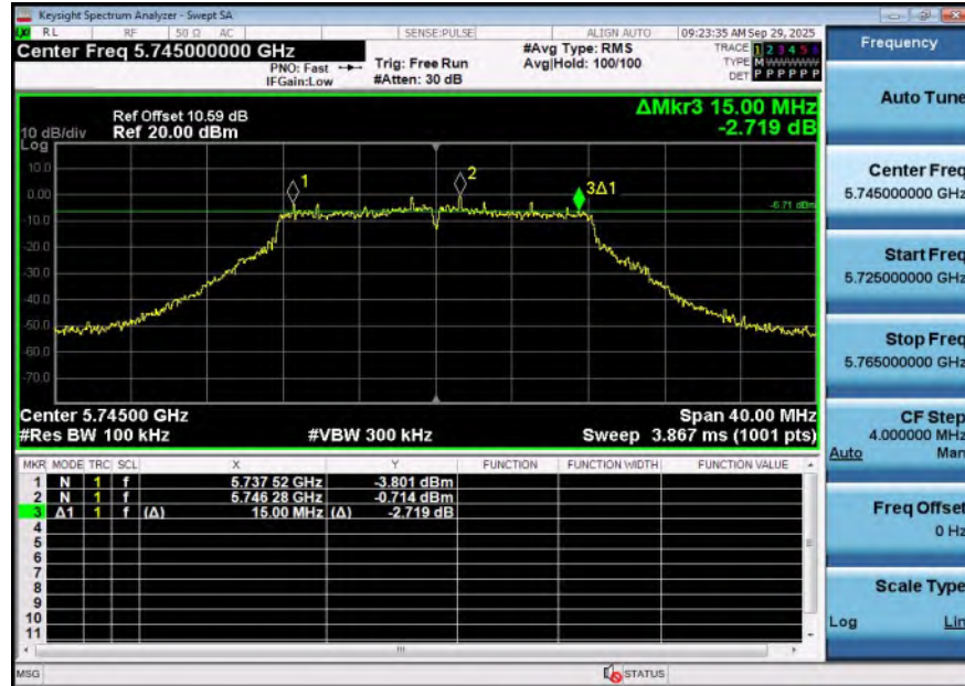
11A-Ant1-5745-PASS
