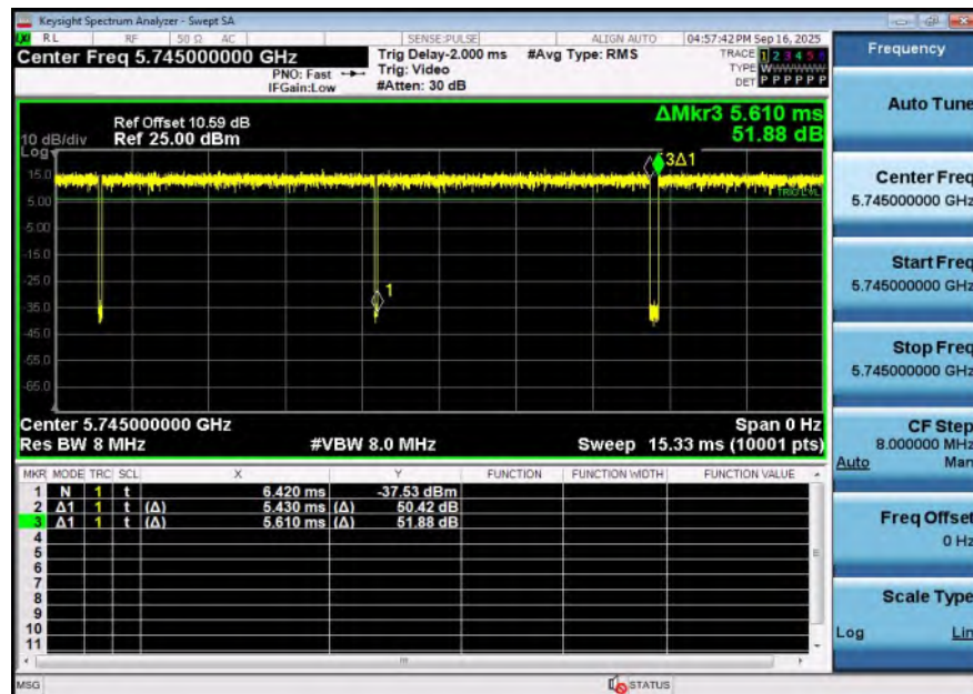
NTNV-11N20SISO-Ant1-5745
