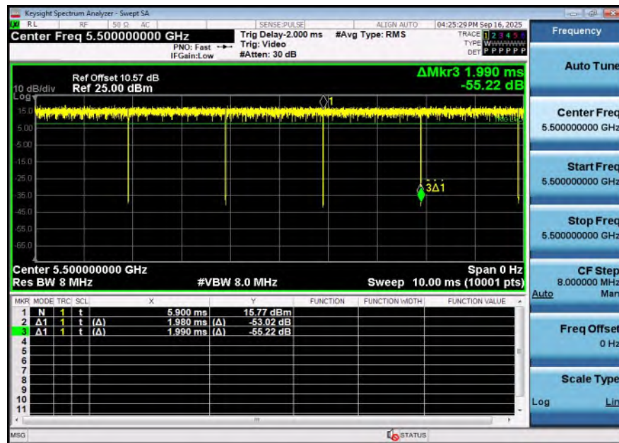
NTNV-11A-Ant1-5500
