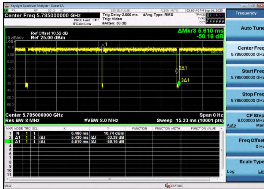
NTNV-11N20SISO-Ant1-5785
