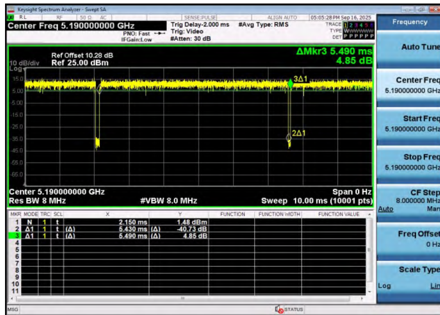
NTNV-11N40SISO-Ant1-5190
