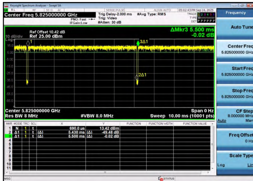
NTNV-11N20SISO-Ant1-5825
