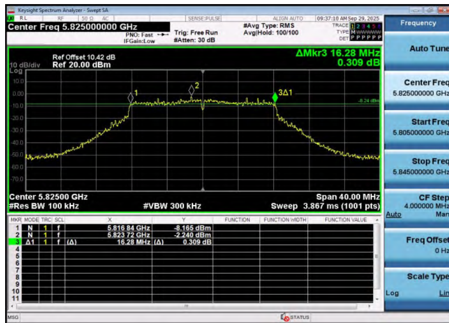
11A-Ant2-5825-PASS
