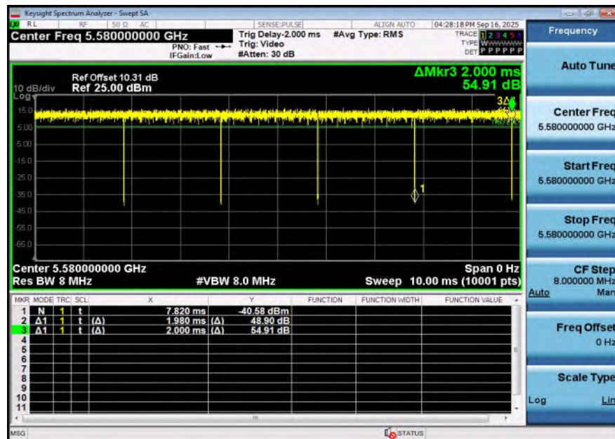
NTNV-11A-Ant1-5580
