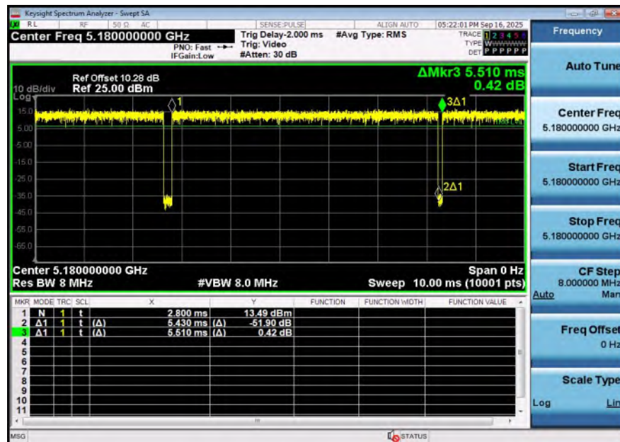
NTNV-11AC20SISO-Ant1-5180
