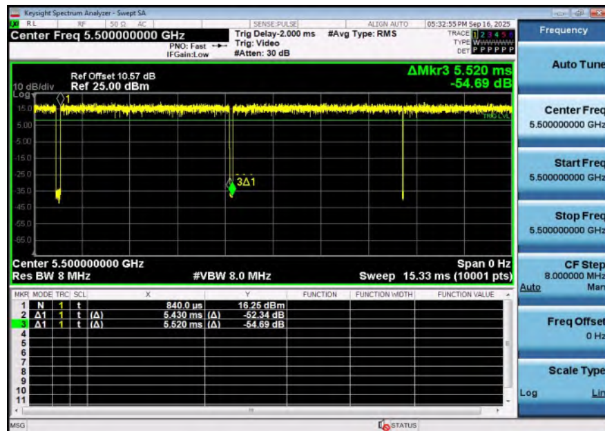
NTNV-11AC20SISO-Ant1-5500
