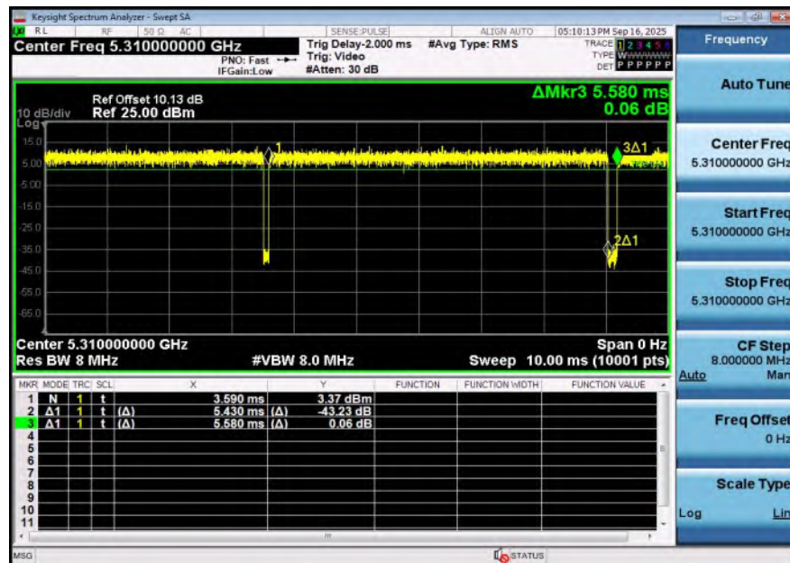
NTNV-11N40SISO-Ant1-5310
