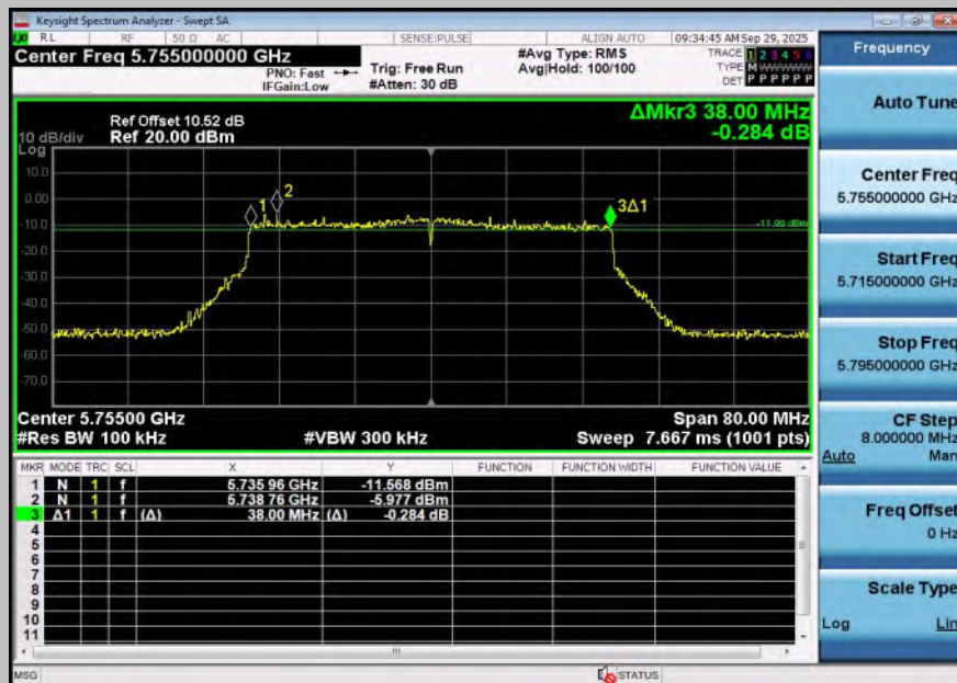
11BE40SISO-Ant1-5755-PASS
