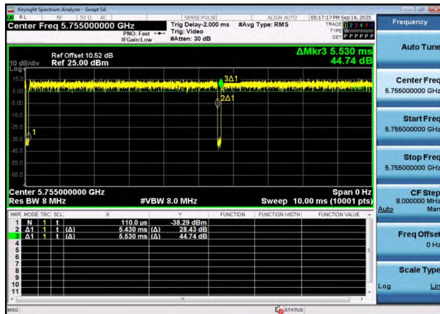
NTNV-11N40SISO-Ant1-5755
