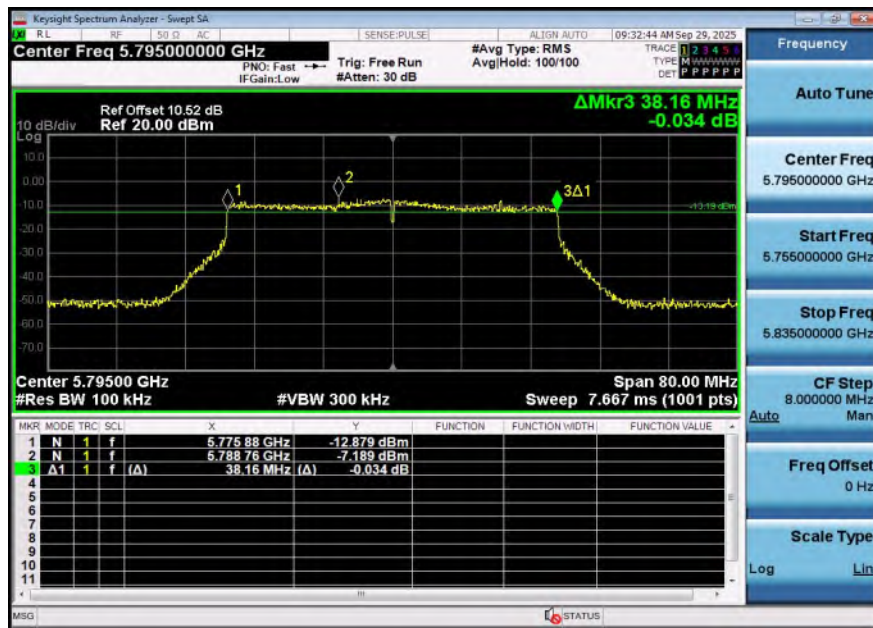
11AX40SISO-Ant1-5795-PASS
