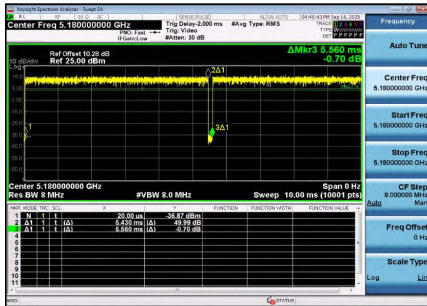
NTNV-11N20SISO-Ant1-5180
