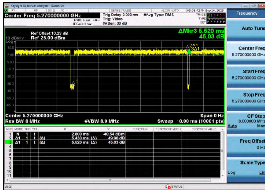
NTNV-11N40SISO-Ant1-5270
