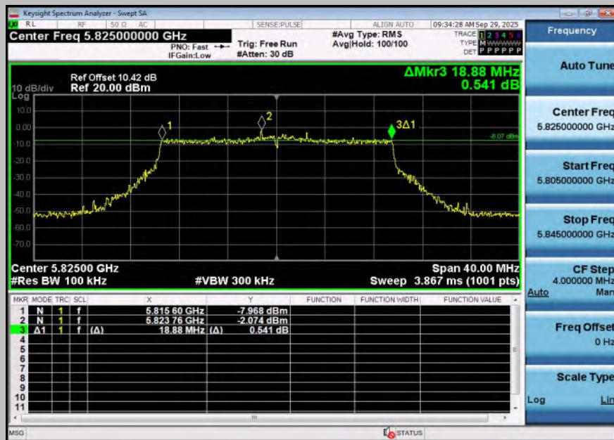
11BE20SISO-Ant1-5825-PASS
