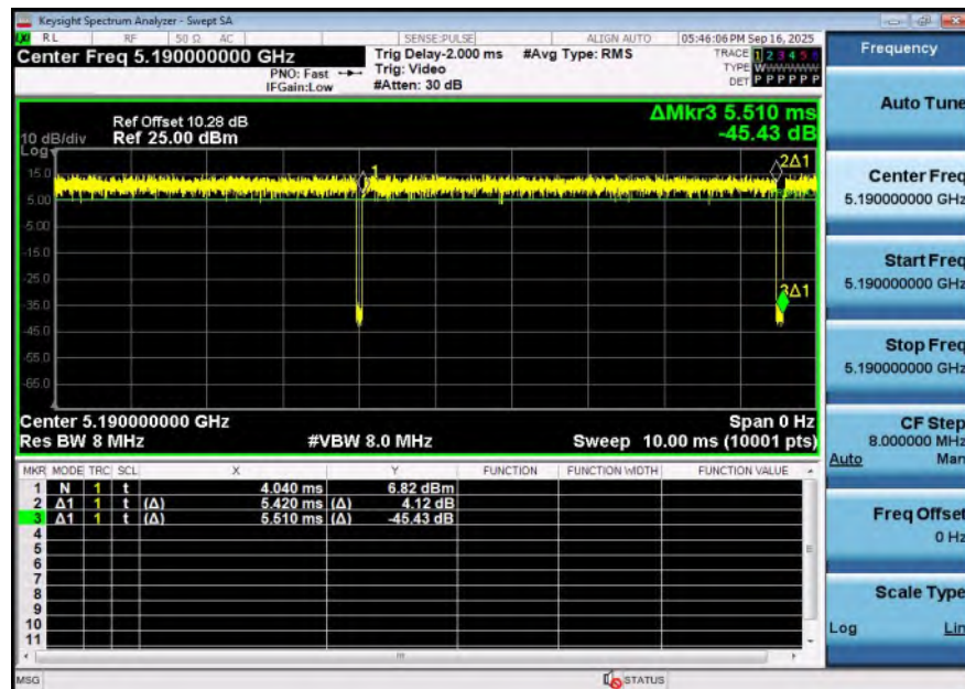
NTNV-11AC40SISO-Ant1-5190
