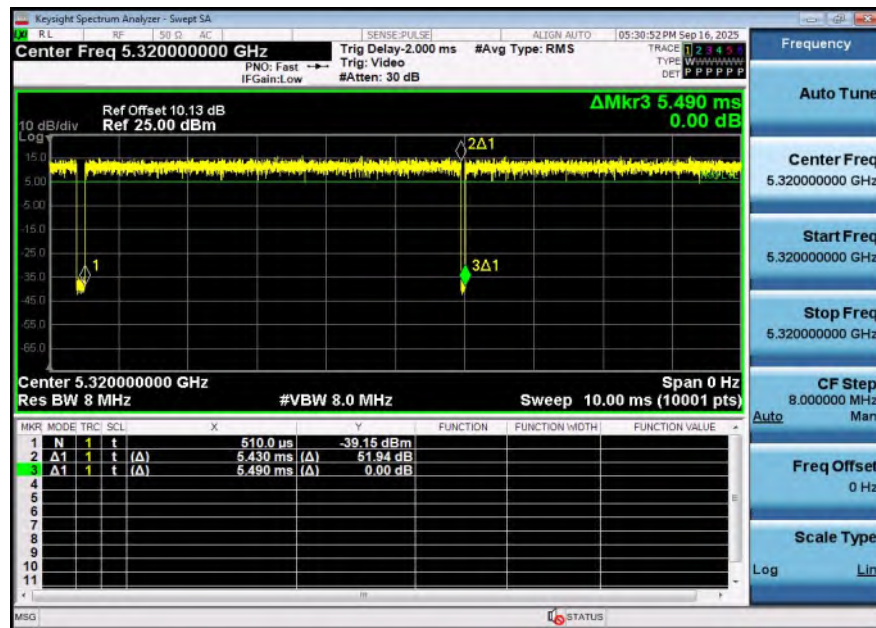
NTNV-11AC20SISO-Ant1-5320
