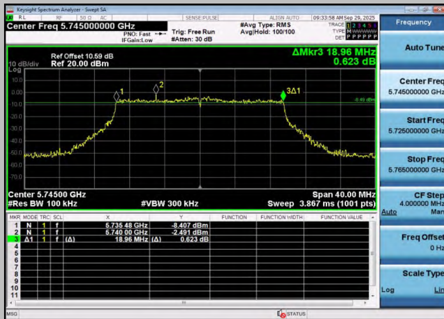
11BE20SISO-Ant1-5745-PASS
