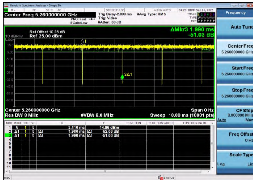
NTNV-11A-Ant1-5260
