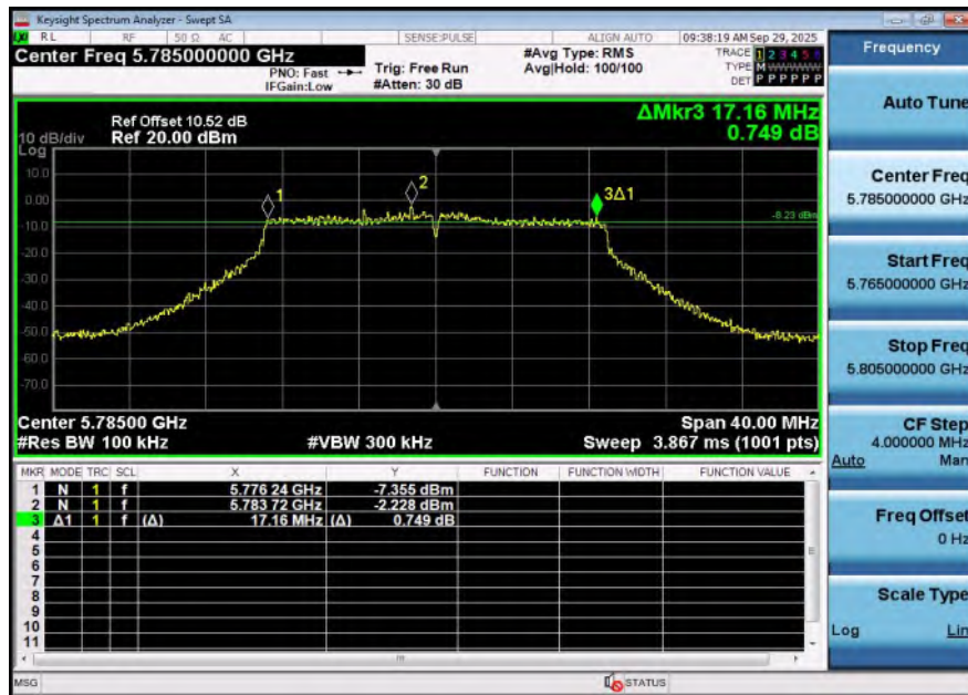
11N20SISO-Ant2-5785-PASS
