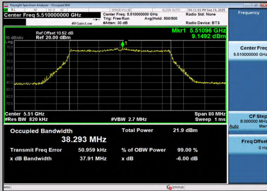
11BE40SISO-Ant2-5510
