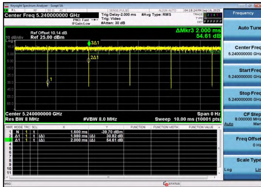
NTNV-11A-Ant1-5240
