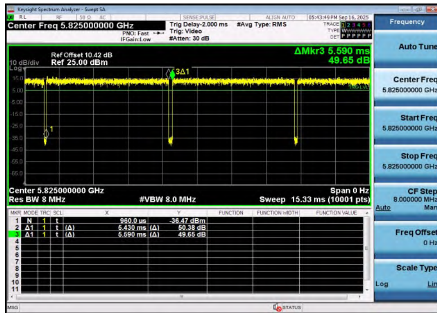
NTNV-11AC20SISO-Ant1-5825
