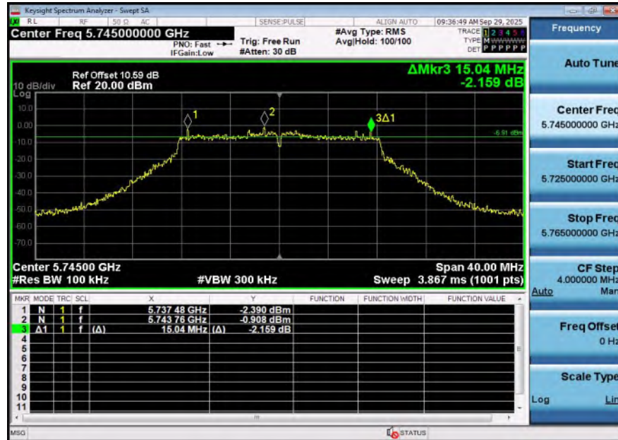
11A-Ant2-5745-PASS
