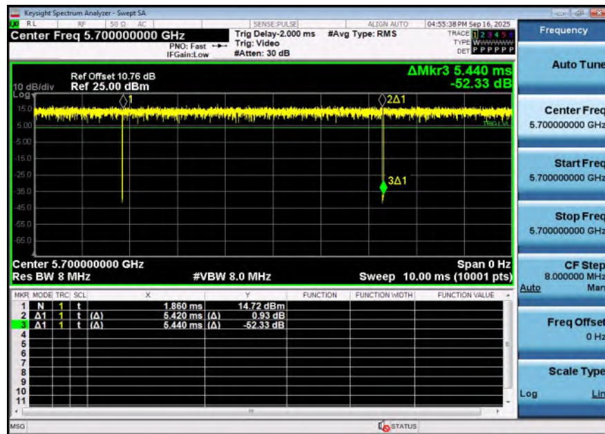
NTNV-11N20SISO-Ant1-5700
