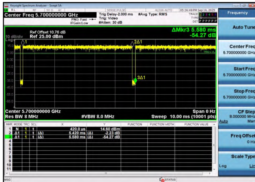
NTNV-11AC20SISO-Ant1-5700
