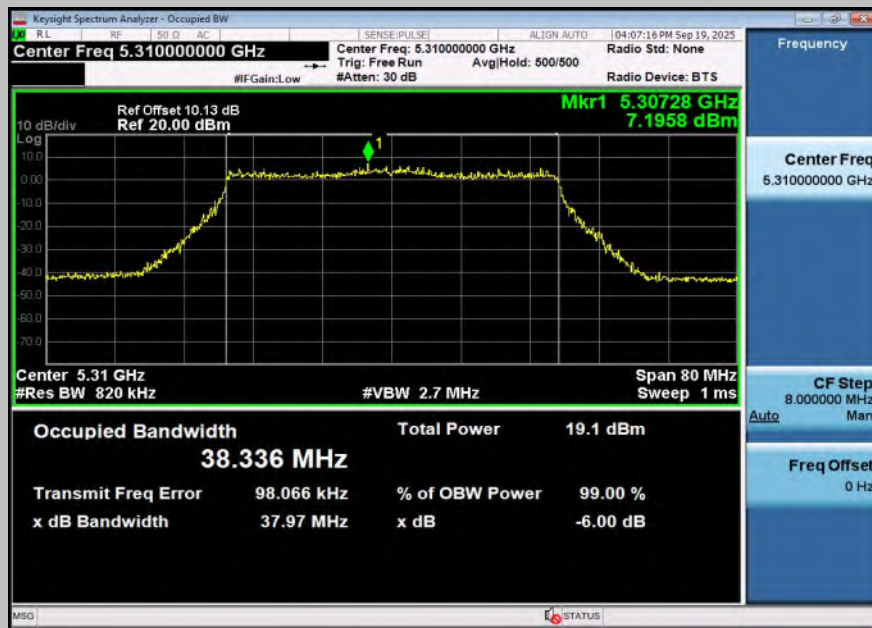
11BE40SISO-Ant2-5310
