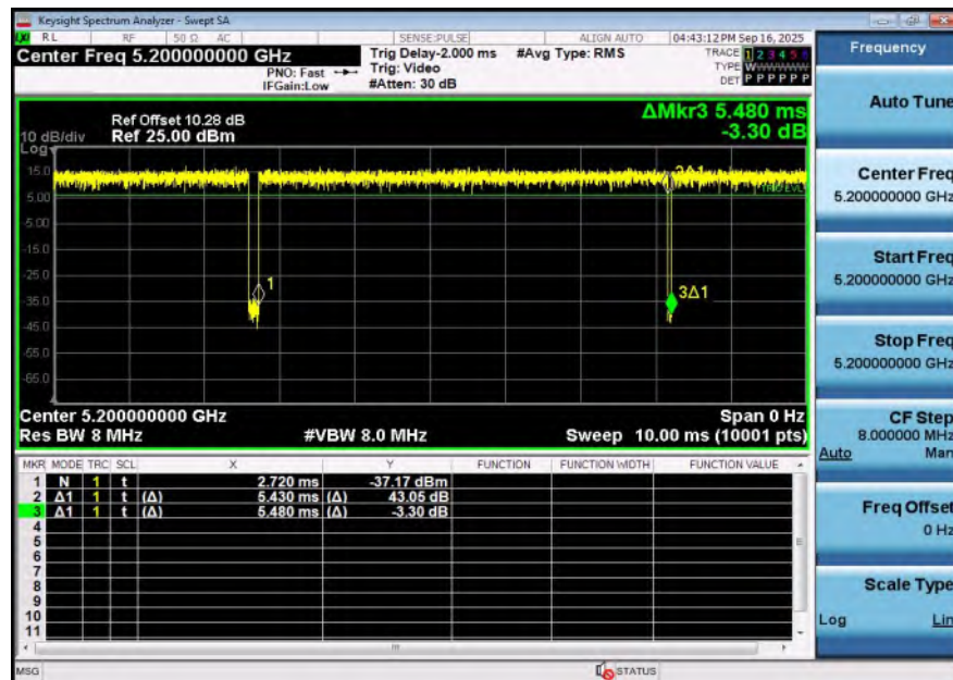
NTNV-11N20SISO-Ant1-5200
