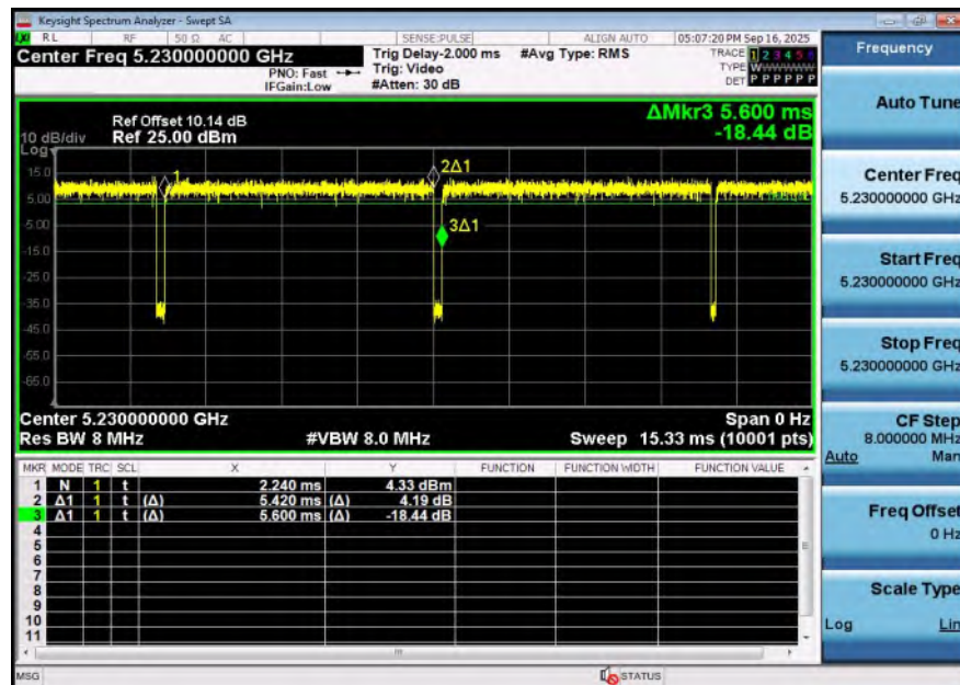
NTNV-11N40SISO-Ant1-5230
