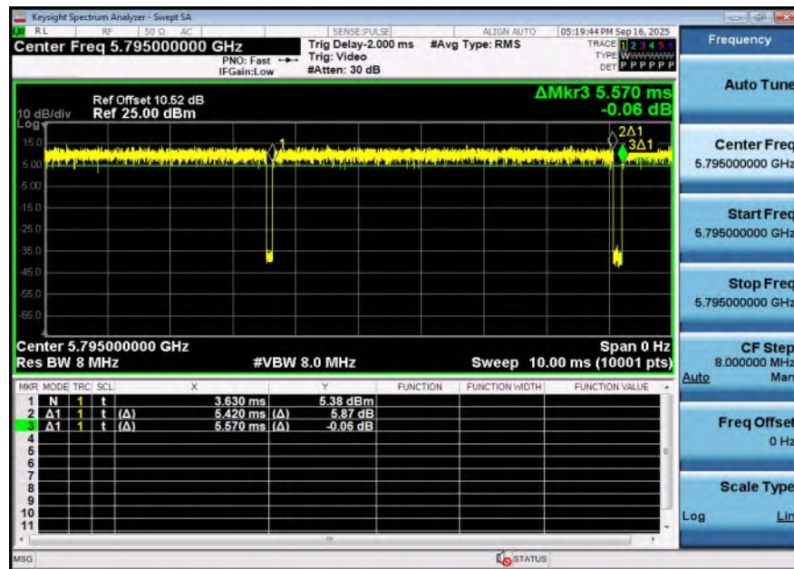
NTNV-11N40SISO-Ant1-5795
