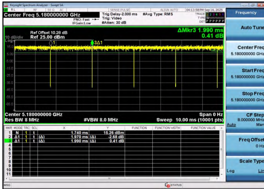
NTNV-11A-Ant1-5180
