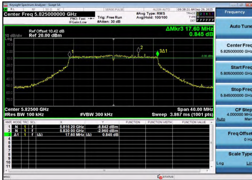
11N20SISO-Ant2-5825-PASS
