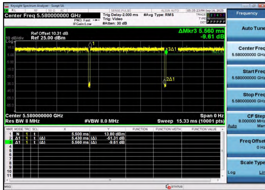
NTNV-11AC20SISO-Ant1-5580
