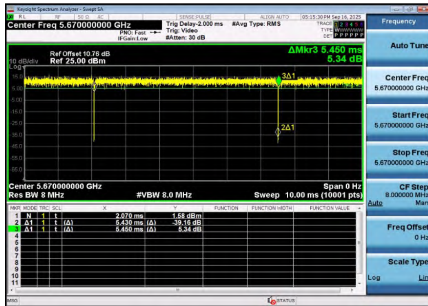
NTNV-11N40SISO-Ant1-5670
