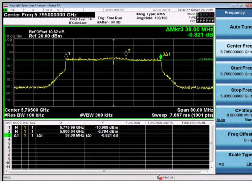
11BE40SISO-Ant1-5795-PASS
