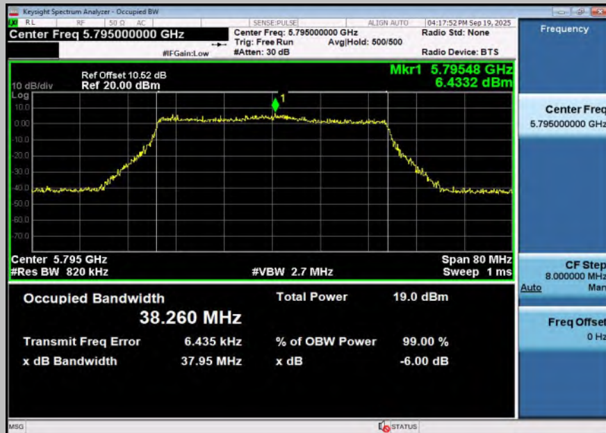
11BE40SISO-Ant2-5795
