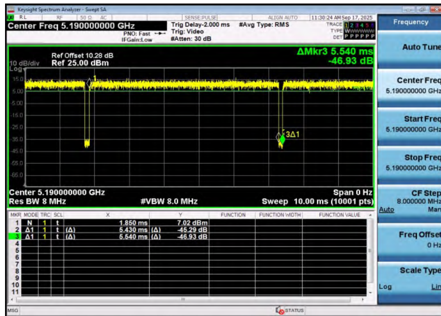
NTNV-11N40SISO-Ant2-5190
