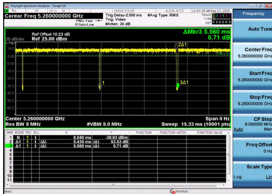
NTNV-11N20SISO-Ant2-5260
