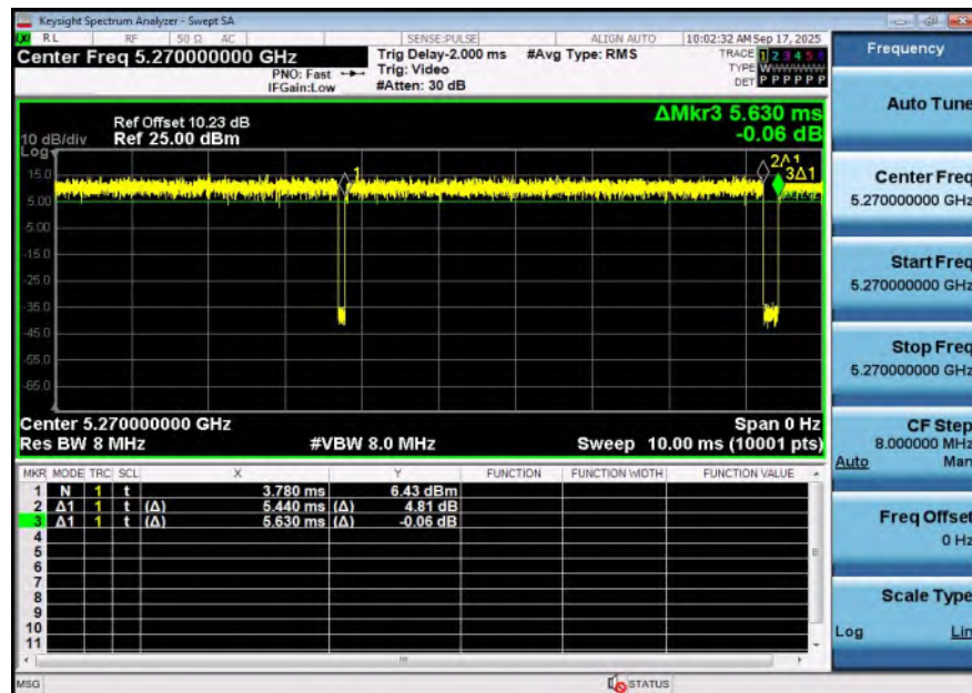
NTNV-11AX40SISO-Ant1-5270
