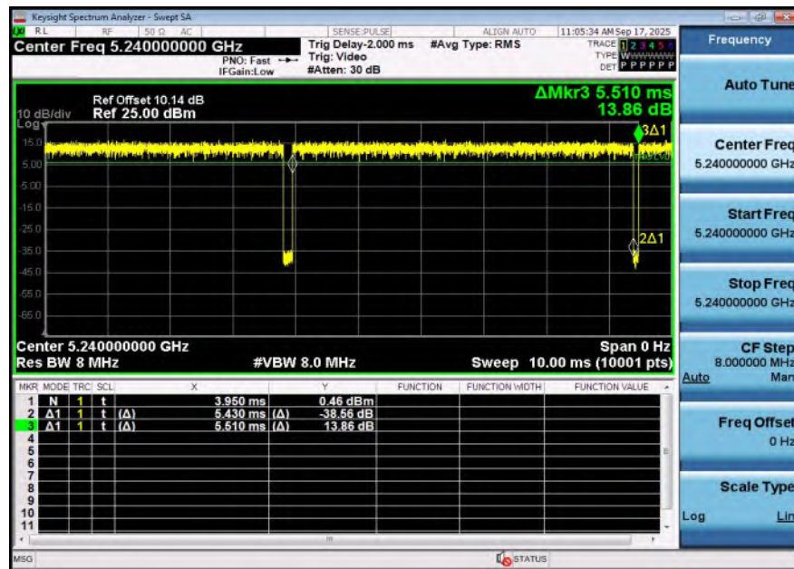
NTNV-11N20SISO-Ant2-5240
