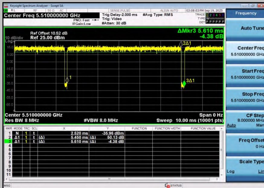
NTNV-11BE40SISO-Ant1-5510
