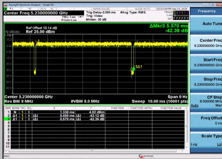
NTNV-11BE40SISO-Ant1-5230
