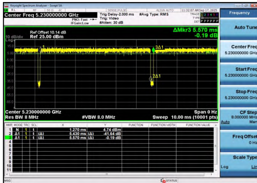
NTNV-11N40SISO-Ant2-5230
