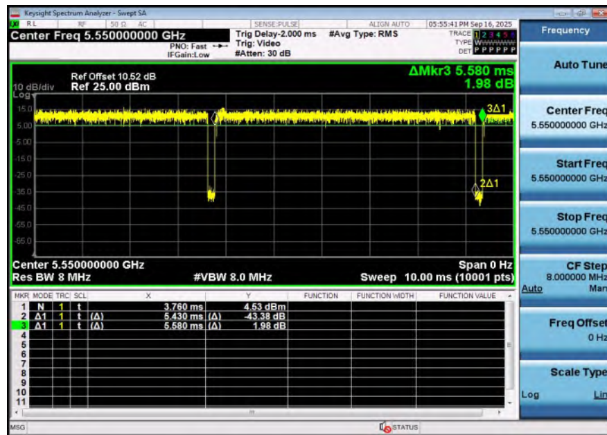
NTNV-11AC40SISO-Ant1-5550
