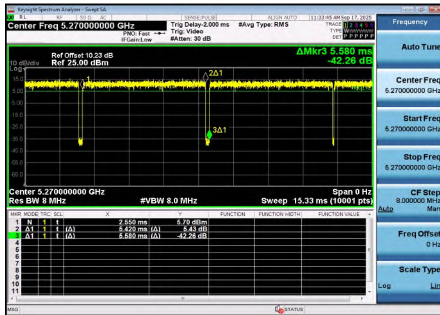
NTNV-11N40SISO-Ant2-5270
