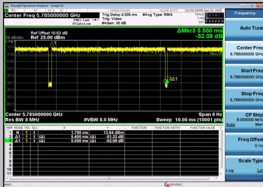
NTNV-11BE20SISO-Ant1-5785
