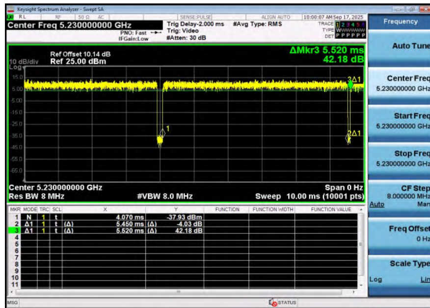
NTNV-11AX40SISO-Ant1-5230
