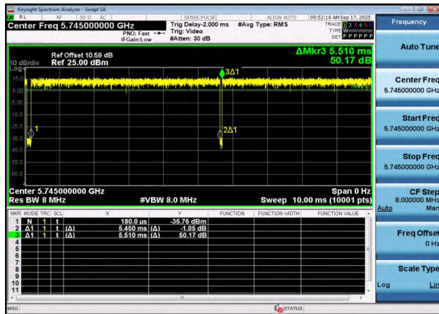
NTNV-11AX20SISO-Ant1-5745
