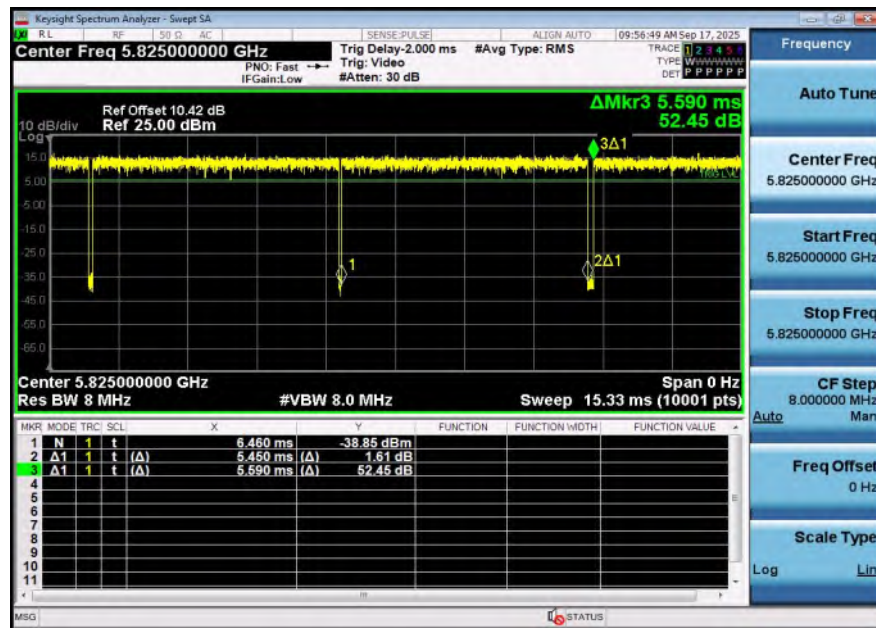
NTNV-11AX20SISO-Ant1-5825
