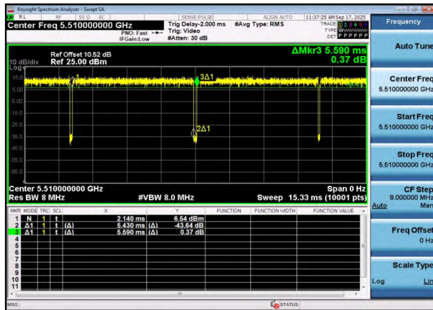
NTNV-11N40SISO-Ant2-5510
