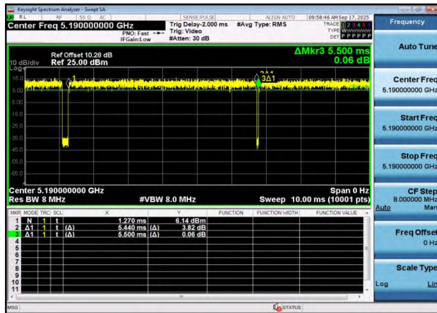
NTNV-11AX40SISO-Ant1-5190
