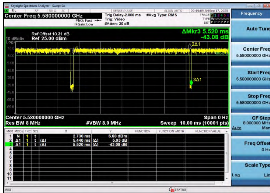
NTNV-11AX20SISO-Ant1-5580
