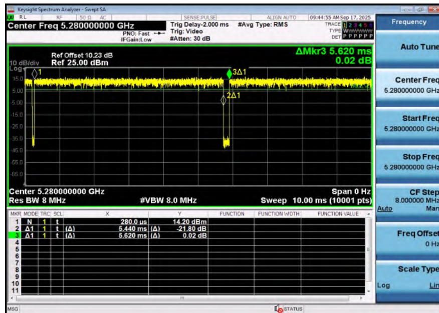
NTNV-11AX20SISO-Ant1-5280
