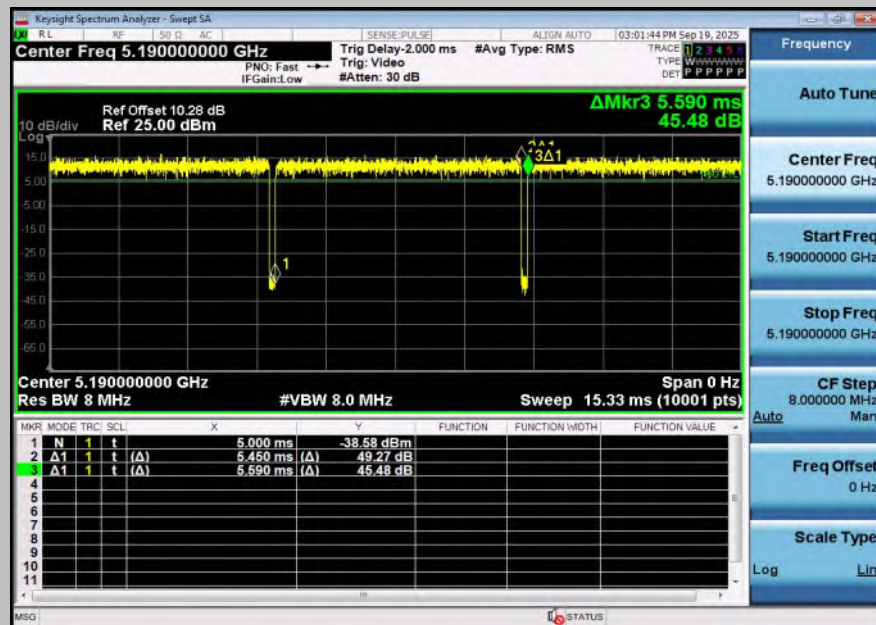
NTNV-11BE40SISO-Ant1-5190
