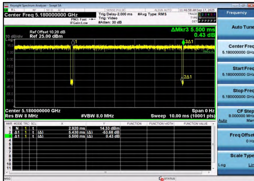
NTNV-11AC20SISO-Ant2-5180
