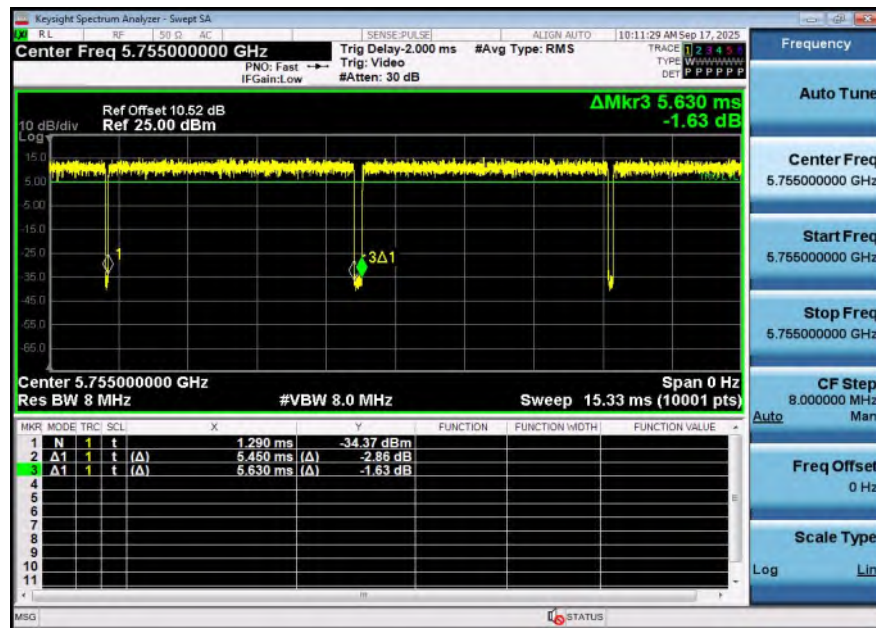
NTNV-11AX40SISO-Ant1-5755
