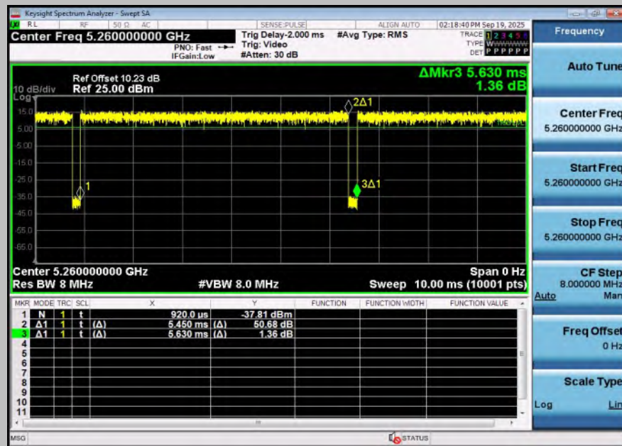
NTNV-11BE20SISO-Ant1-5260
