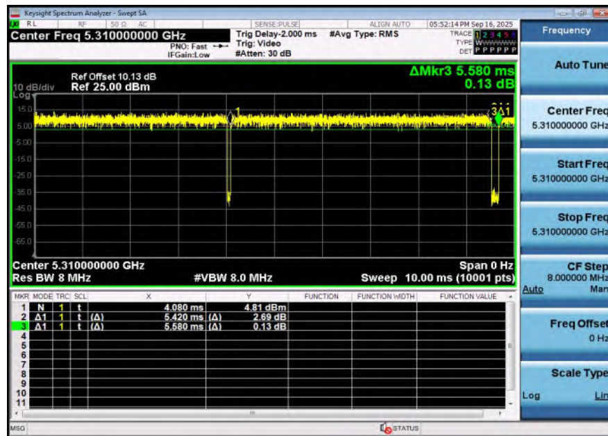
NTNV-11AC40SISO-Ant1-5310
