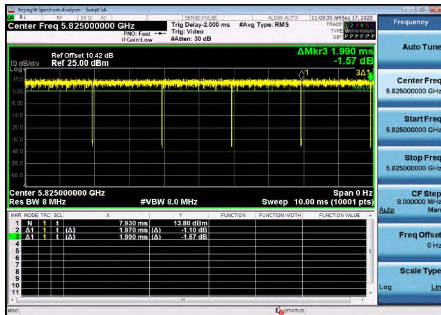
NTNV-11A-Ant2-5825
