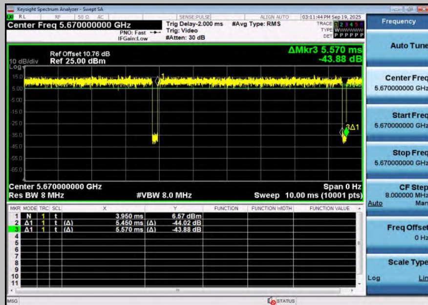
NTNV-11BE40SISO-Ant1-5670
