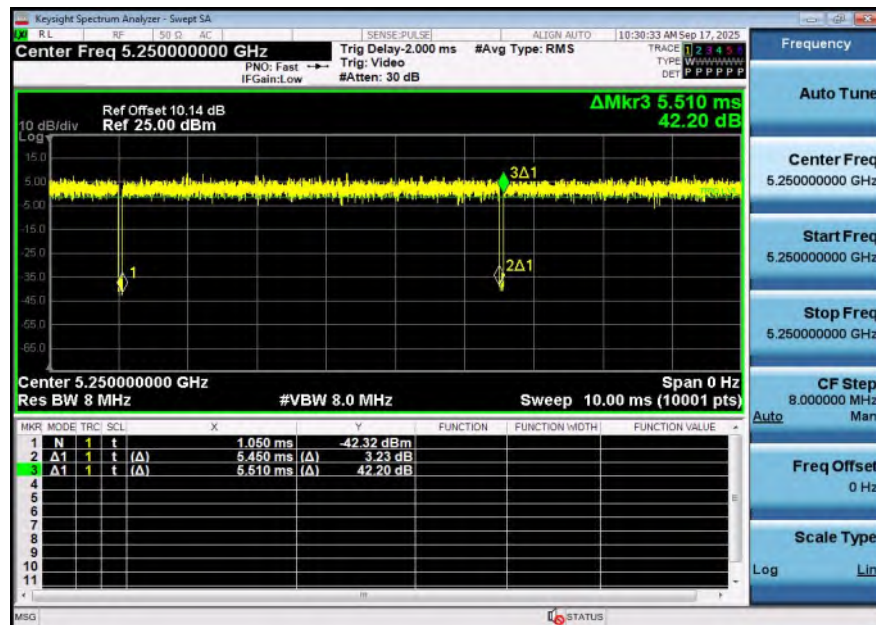
NTNV-11AX160SISO-Ant1-5250
