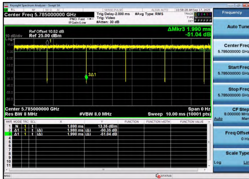
NTNV-11A-Ant2-5785
