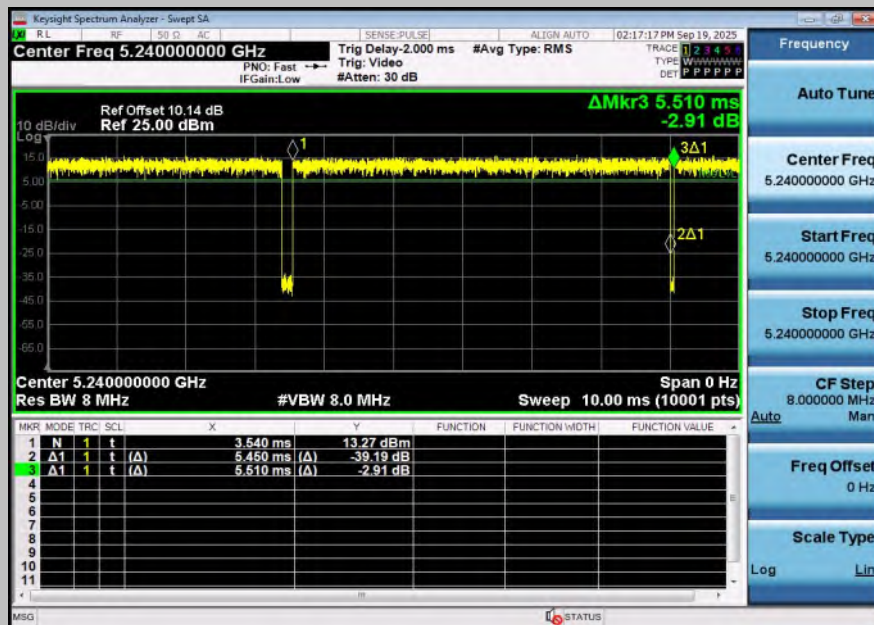
NTNV-11BE20SISO-Ant1-5240
