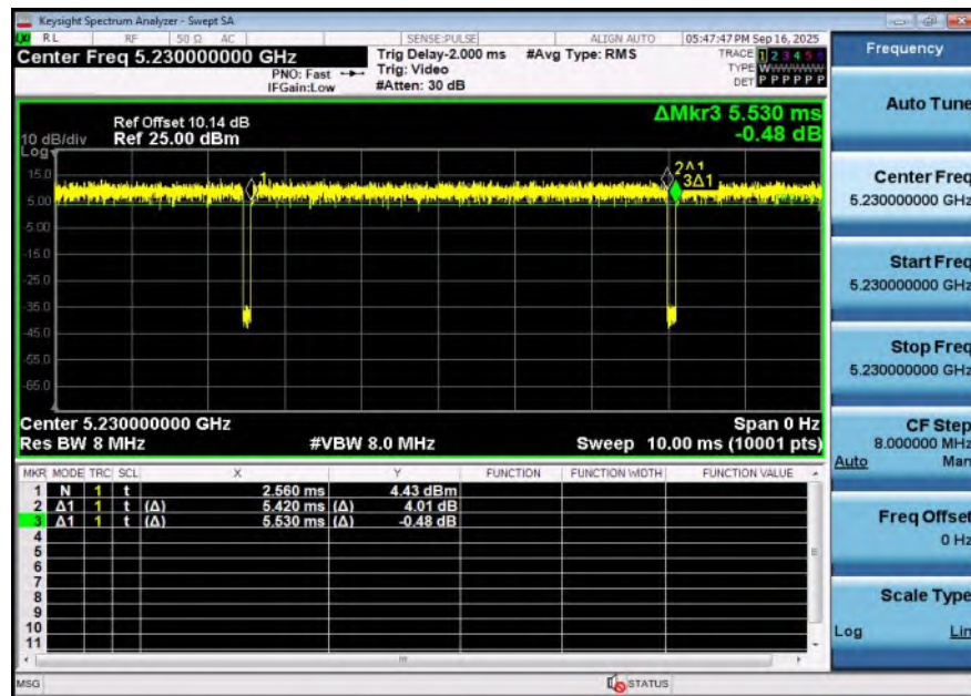
NTNV-11AC40SISO-Ant1-5230
