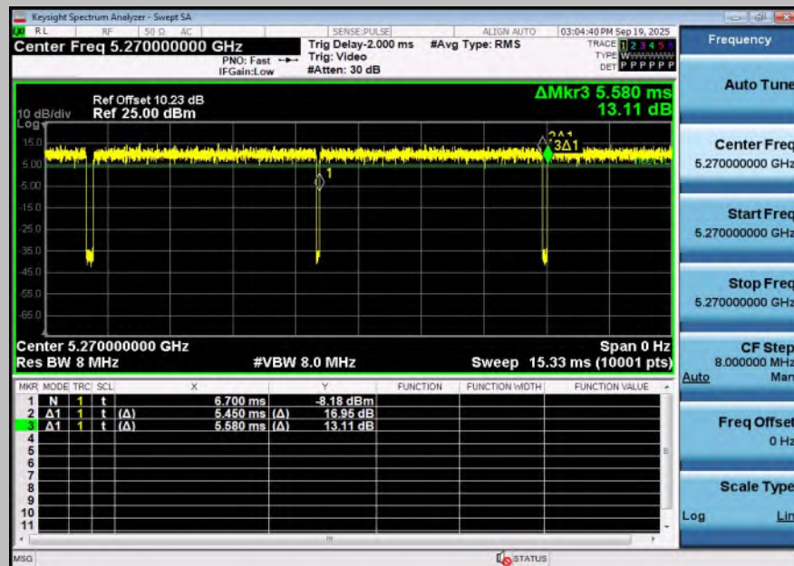
NTNV-11BE40SISO-Ant1-5270
