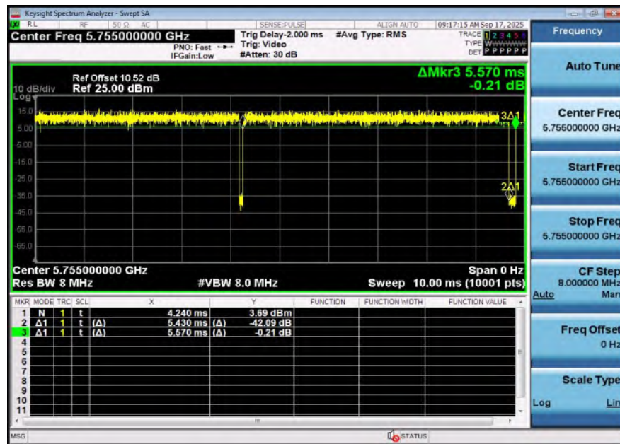
NTNV-11AC40SISO-Ant1-5755
