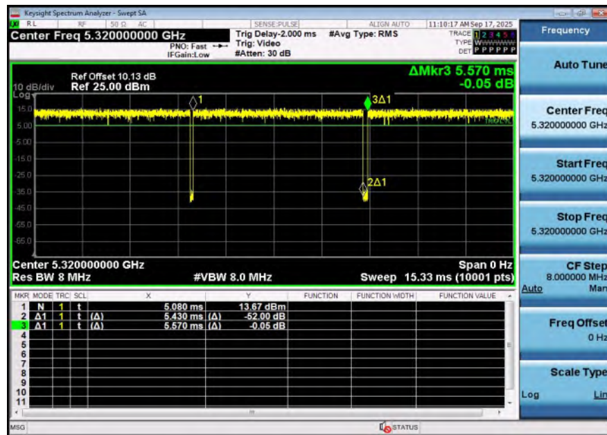
NTNV-11N20SISO-Ant2-5320
