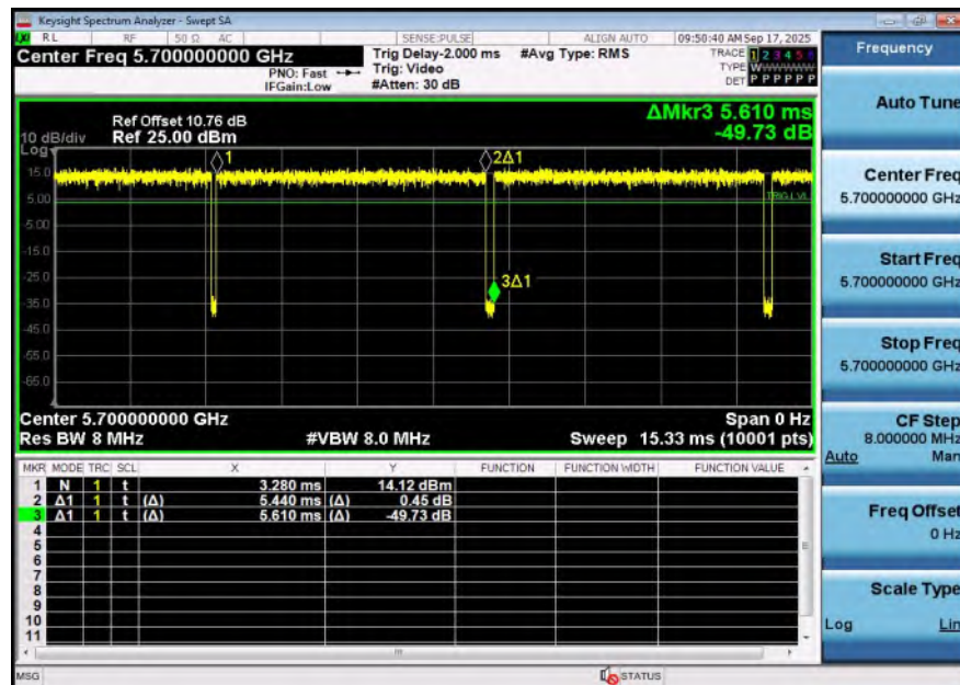
NTNV-11AX20SISO-Ant1-5700
