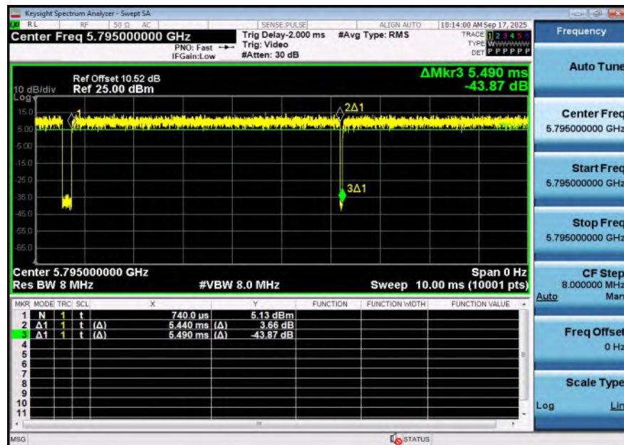
NTNV-11AX40SISO-Ant1-5795
