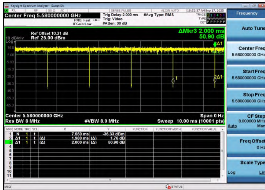
NTNV-11A-Ant2-5580
