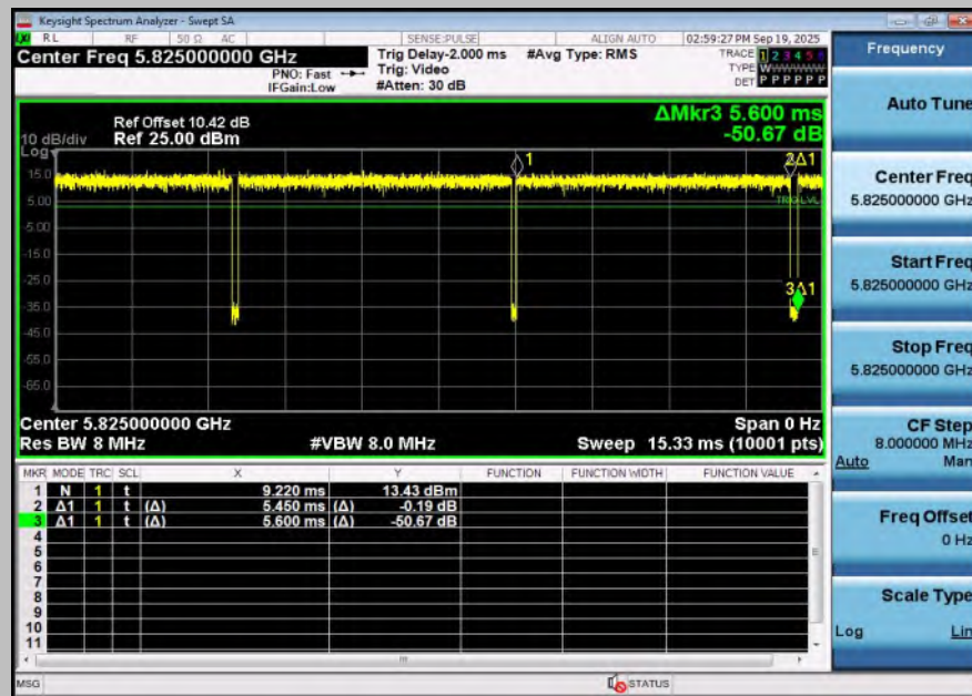
NTNV-11BE20SISO-Ant1-5825
