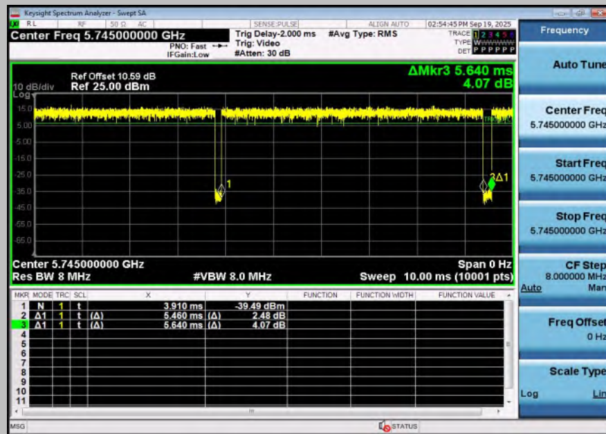
NTNV-11BE20SISO-Ant1-5745
