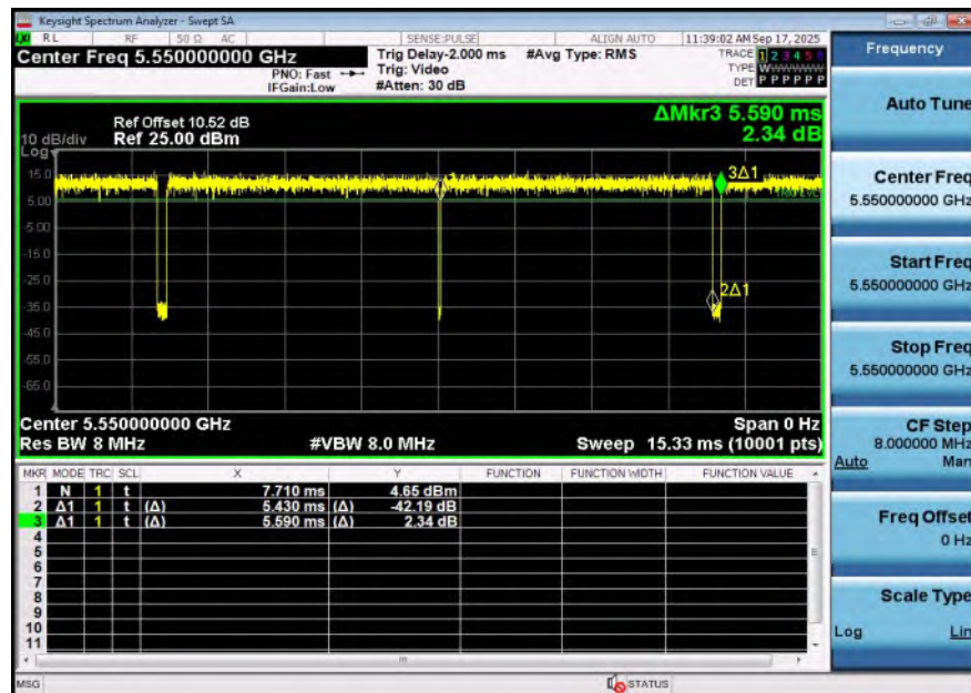
NTNV-11N40SISO-Ant2-5550
