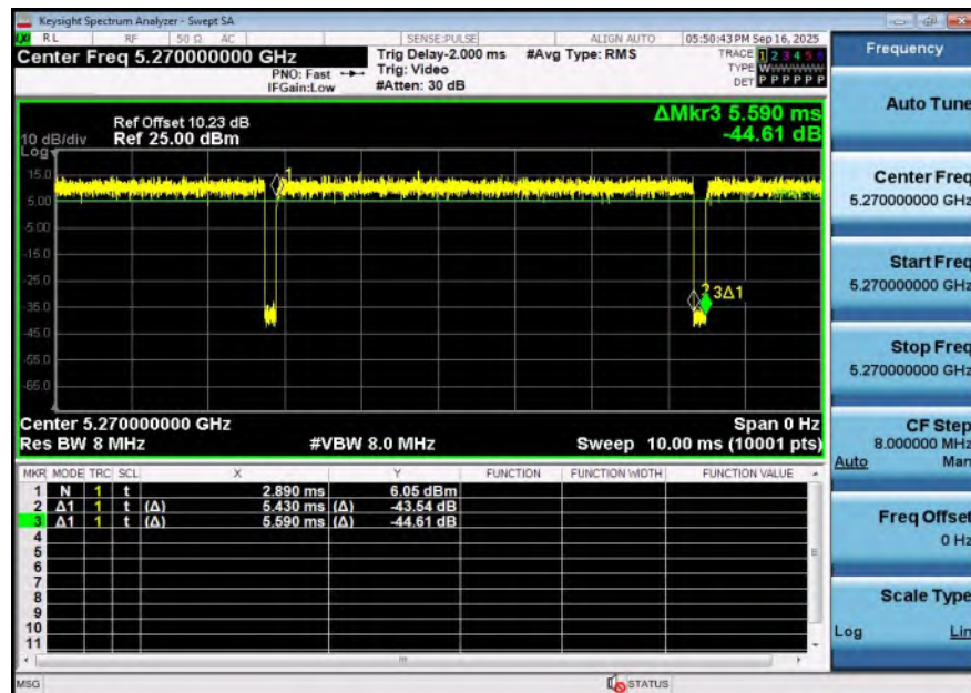
NTNV-11AC40SISO-Ant1-5270
