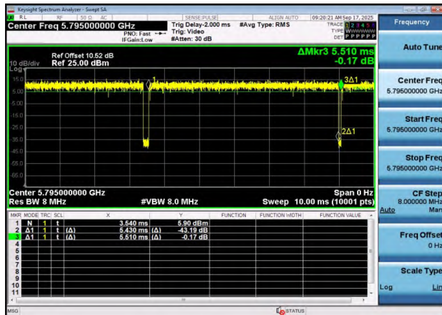
NTNV-11AC40SISO-Ant1-5795
