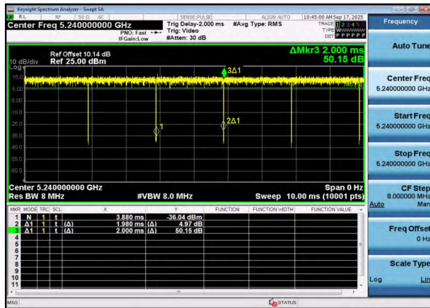
NTNV-11A-Ant2-5240
