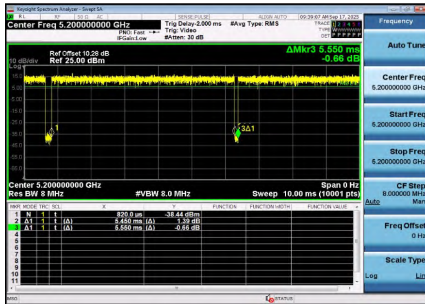
NTNV-11AX20SISO-Ant1-5200
