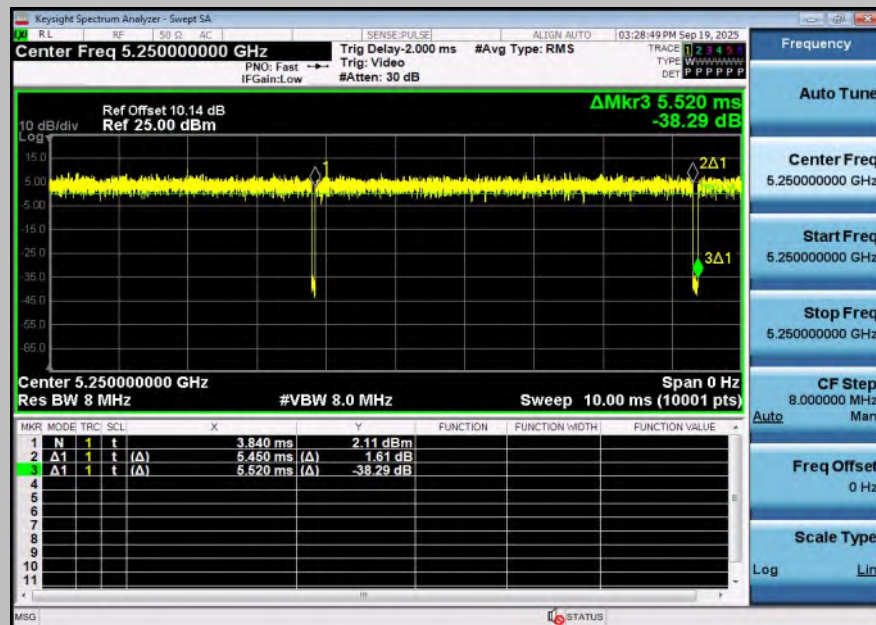
NTNV-11BE160SISO-Ant1-5250
