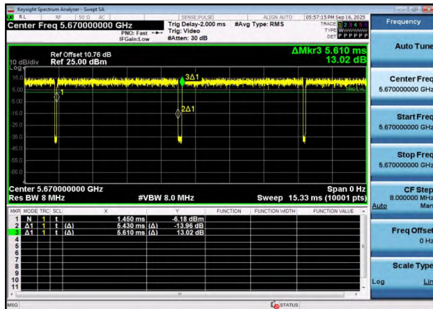
NTNV-11AC40SISO-Ant1-5670
