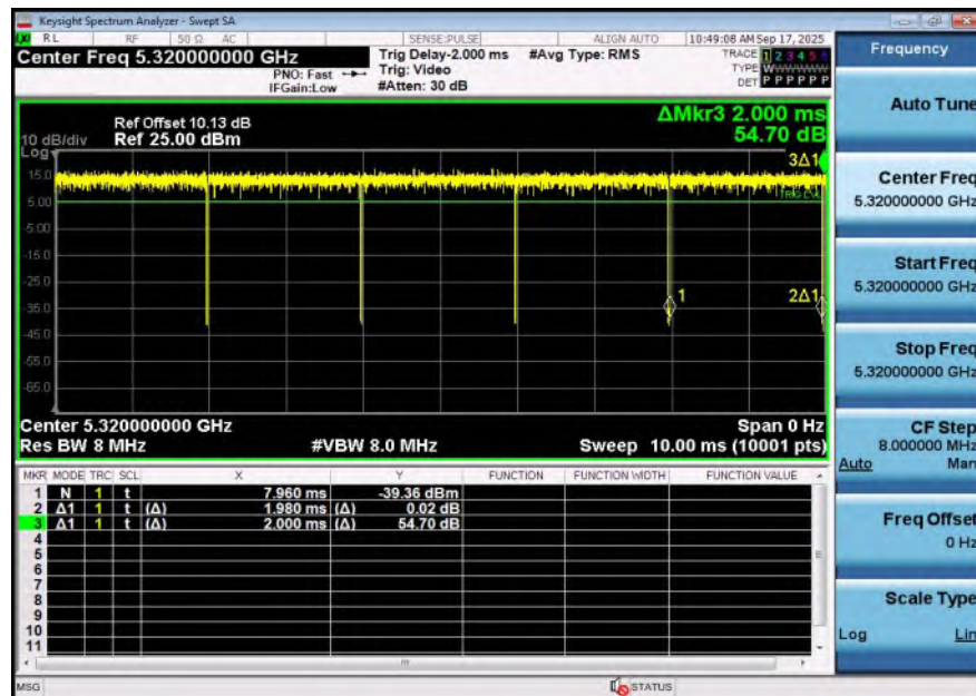
NTNV-11A-Ant2-5320
