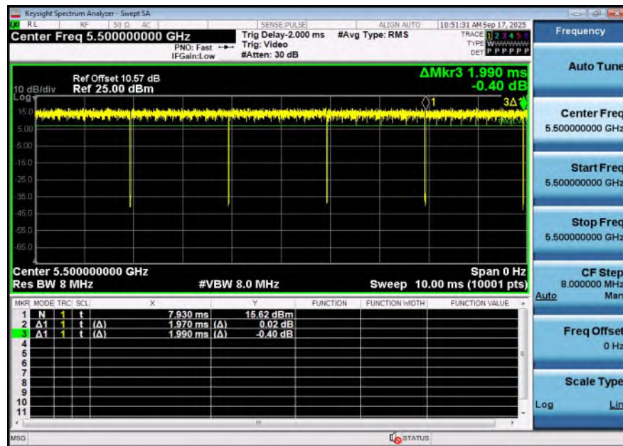
NTNV-11A-Ant2-5500
