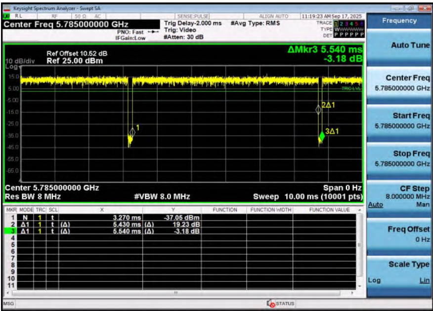
NTNV-11N20SISO-Ant2-5785
