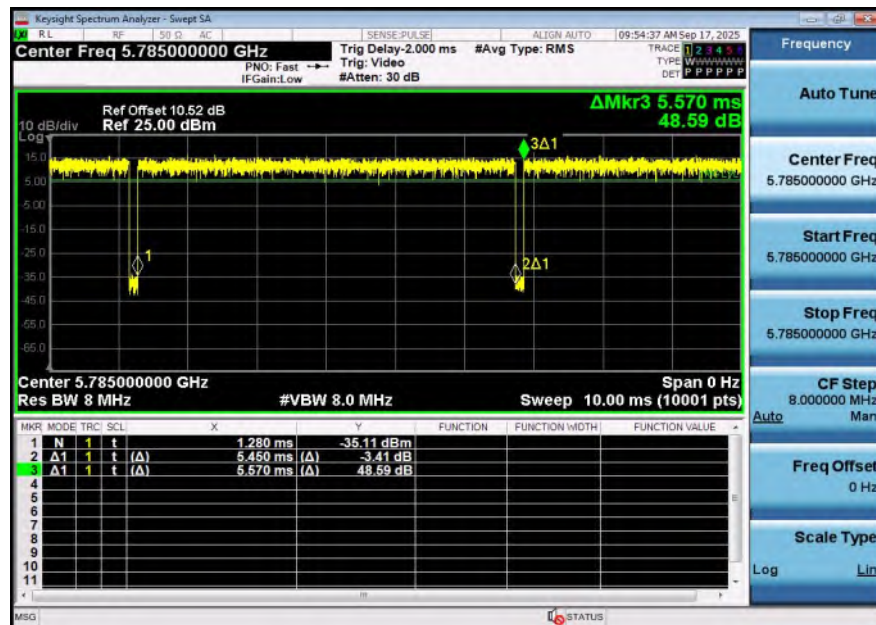
NTNV-11AX20SISO-Ant1-5785
