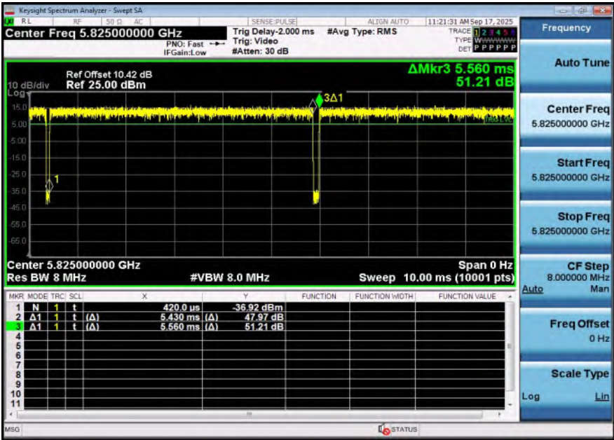
NTNV-11N20SISO-Ant2-5825
