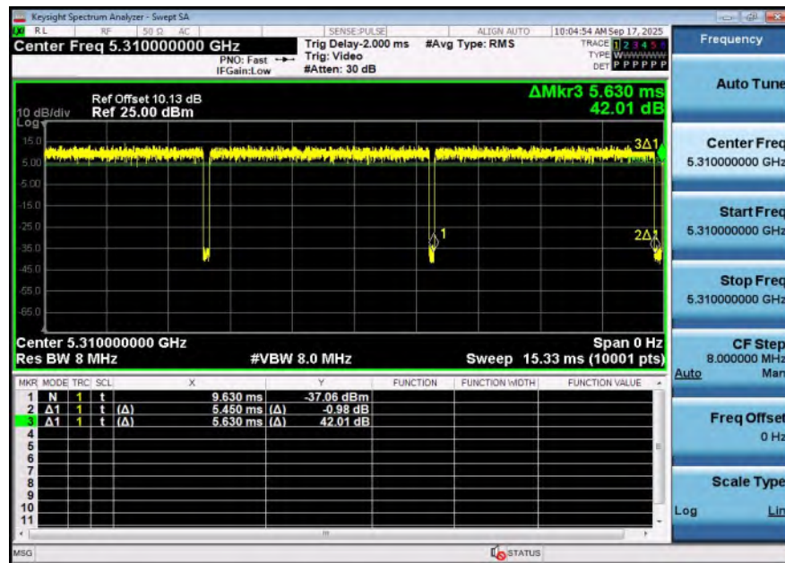
NTNV-11AX40SISO-Ant1-5310
