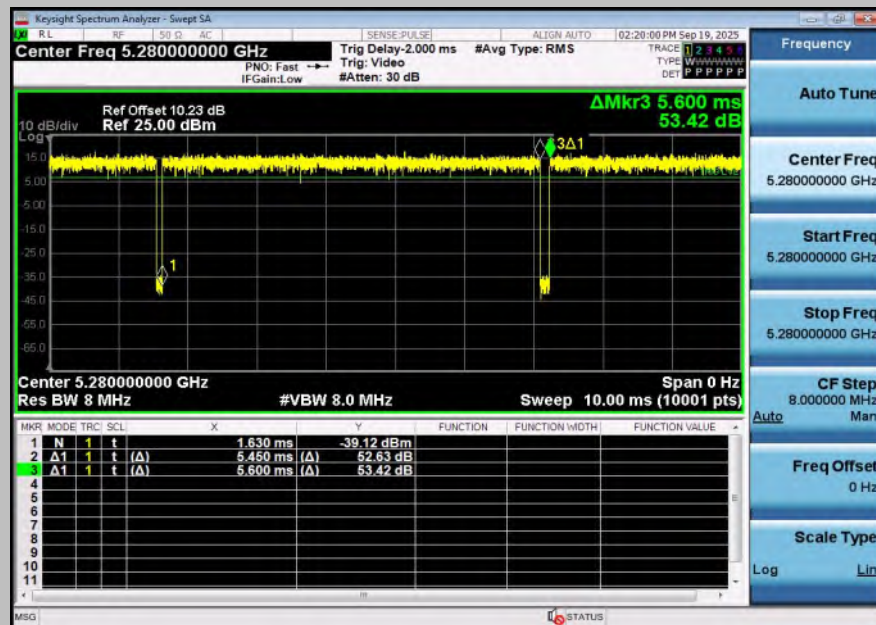
NTNV-11BE20SISO-Ant1-5280
