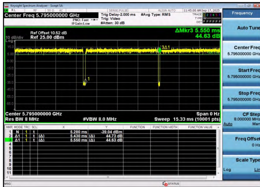
NTNV-11N40SISO-Ant2-5795
