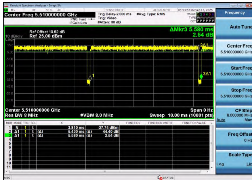
NTNV-11AC40SISO-Ant1-5510
