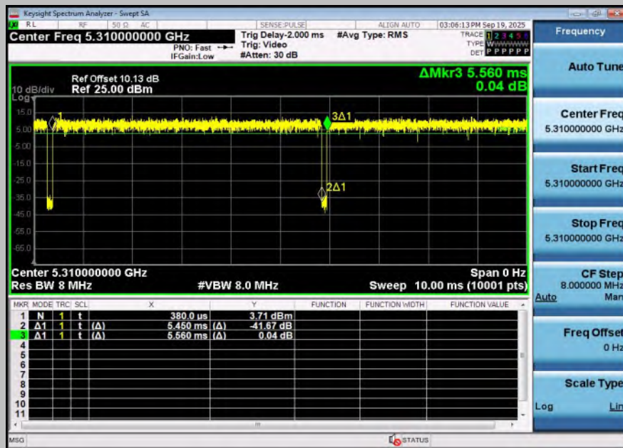
NTNV-11BE40SISO-Ant1-5310
