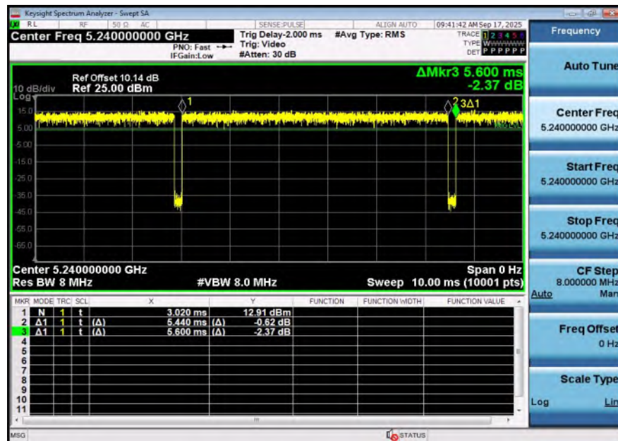
NTNV-11AX20SISO-Ant1-5240
