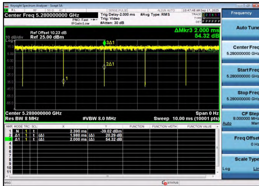
NTNV-11A-Ant2-5280
