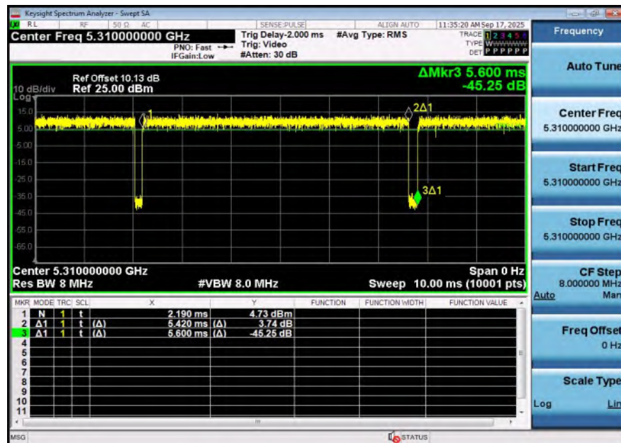
NTNV-11N40SISO-Ant2-5310
