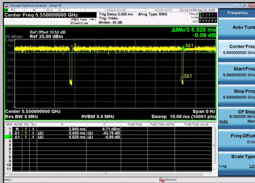
NTNV-11BE40SISO-Ant1-5550
