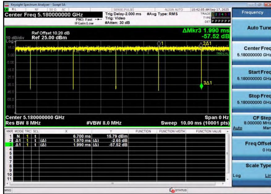
NTNV-11A-Ant2-5180
