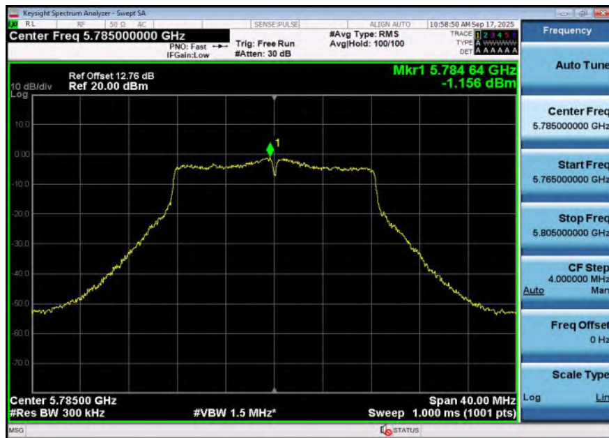
11A-Ant2-5785-PASS
