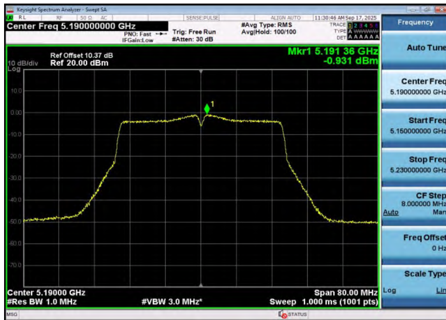
11N40SISO-Ant2-5190-PASS
