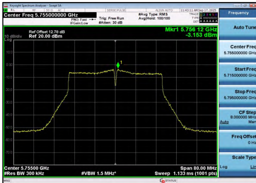
11N40SISO-Ant2-5755-PASS
