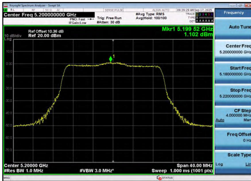
11AX20SISO-Ant1-5200-PASS
