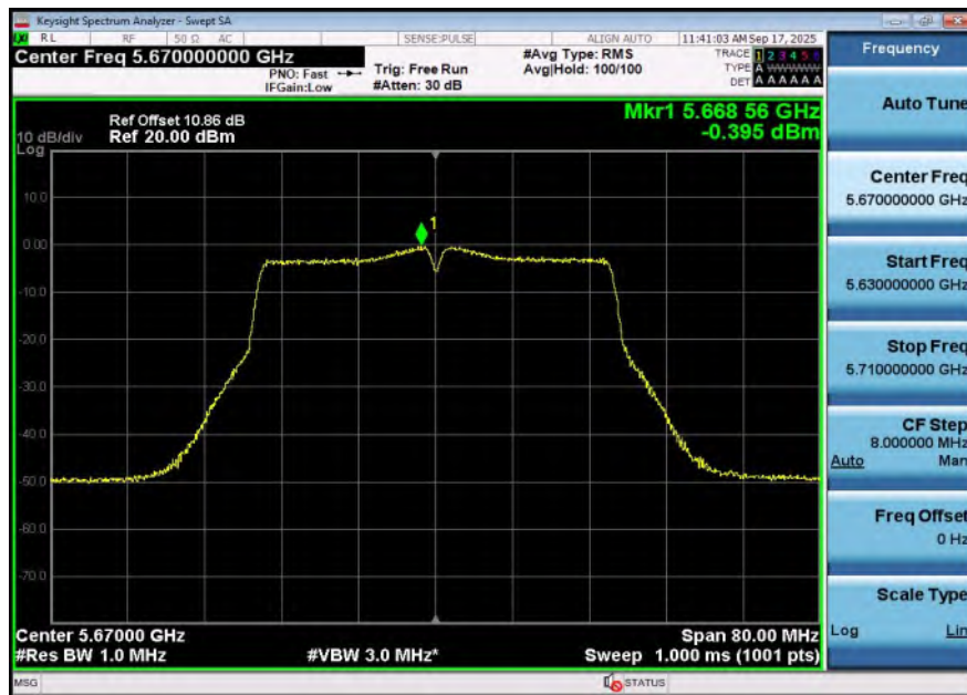
11N40SISO-Ant2-5670-PASS
