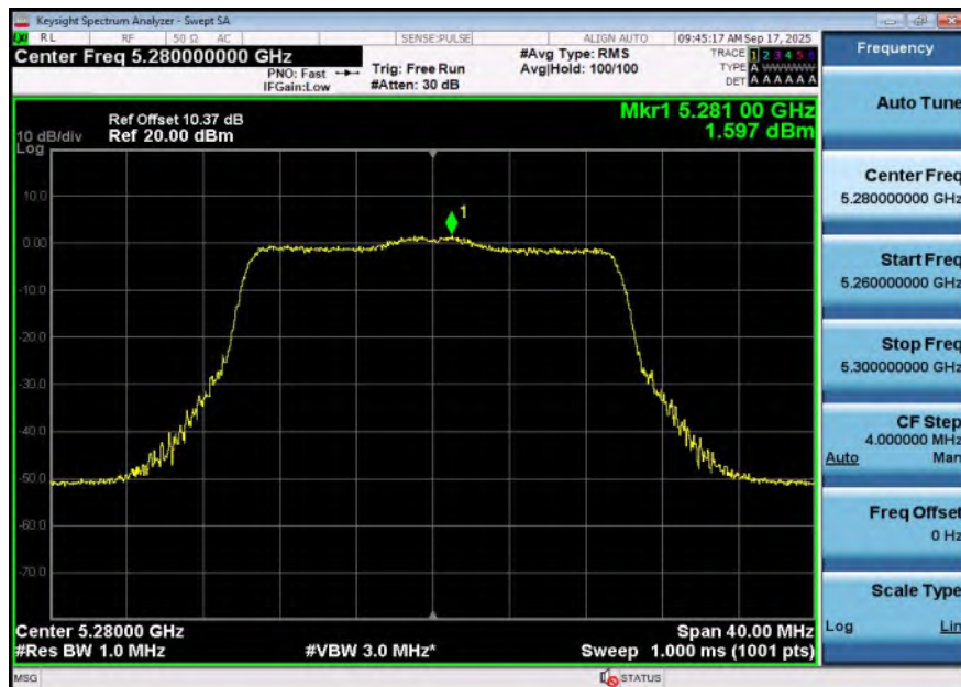
11AX20SISO-Ant1-5280-PASS
