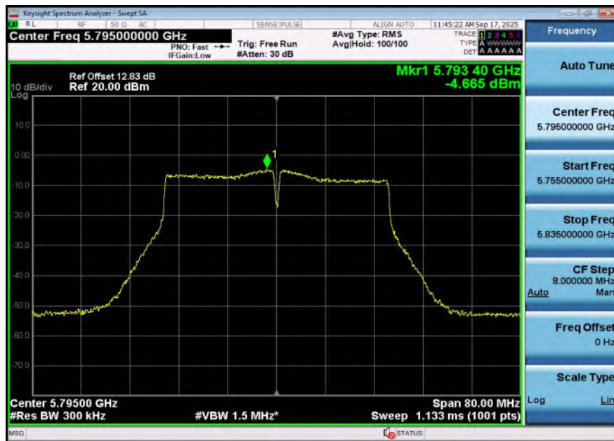
11N40SISO-Ant2-5795-PASS
