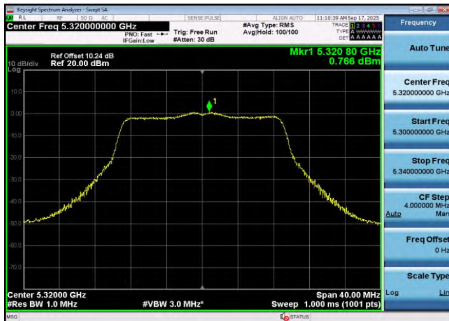
11N20SISO-Ant2-5320-PASS
