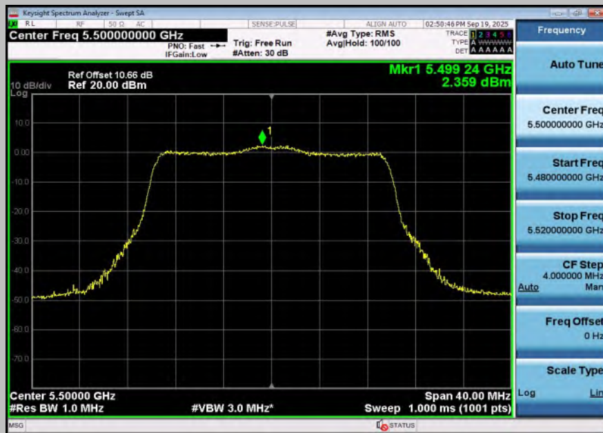
11BE20SISO-Ant1-5500-PASS
