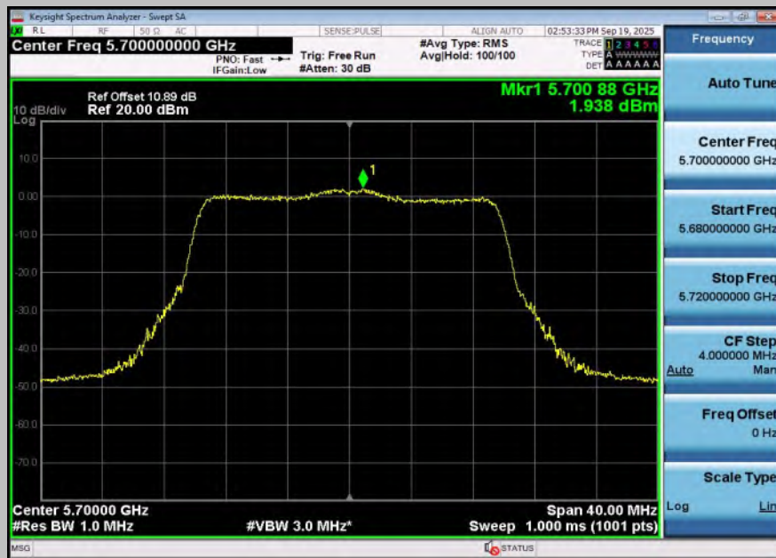
11BE20SISO-Ant1-5700-PASS
