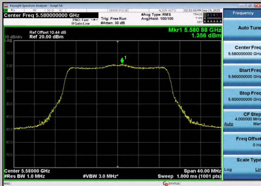
11BE20SISO-Ant1-5580-PASS
