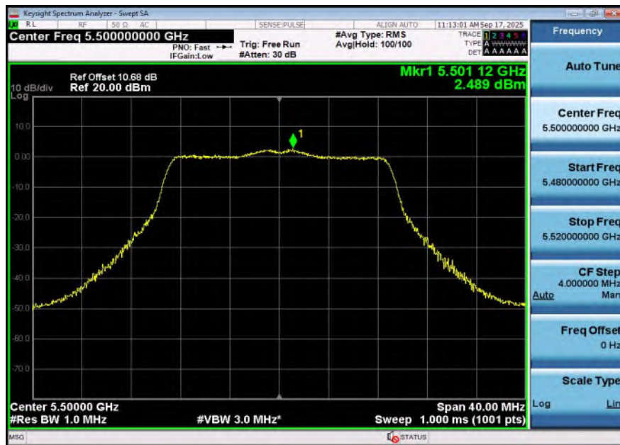
11N20SISO-Ant2-5500-PASS
