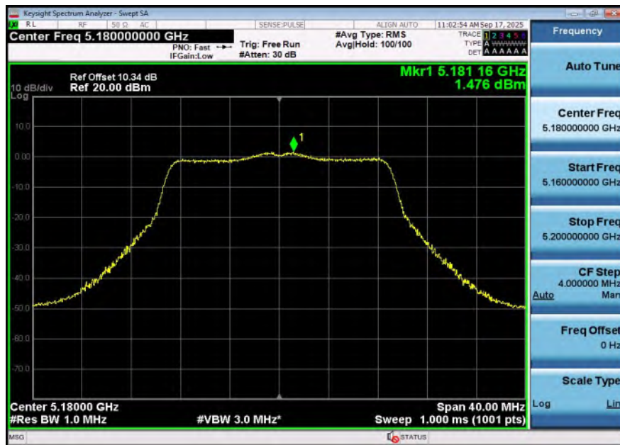
11N20SISO-Ant2-5180-PASS
