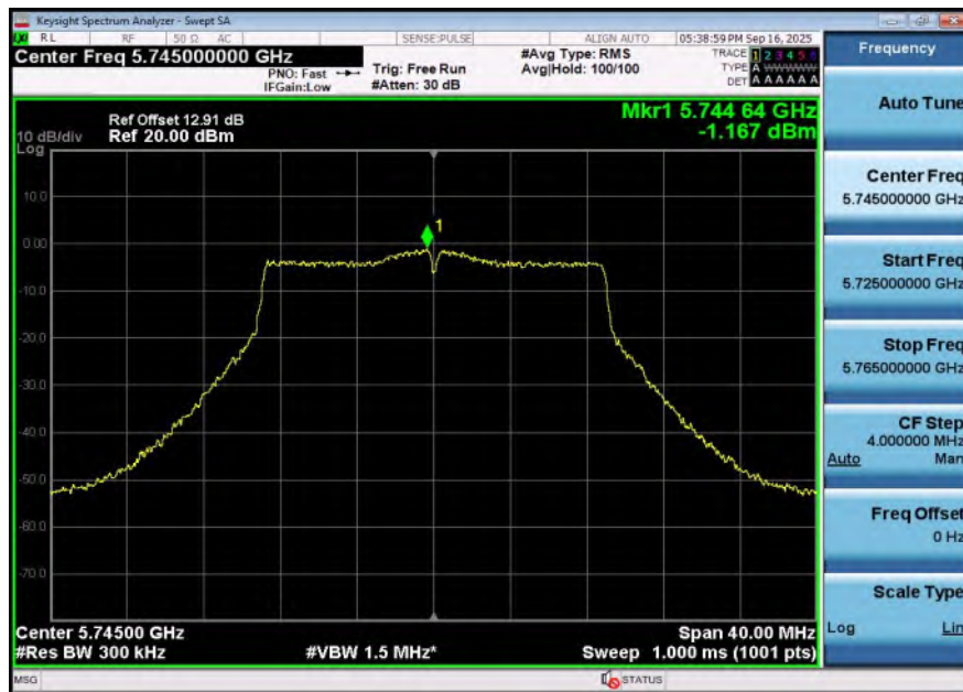
11AC20SISO-Ant1-5745-PASS
