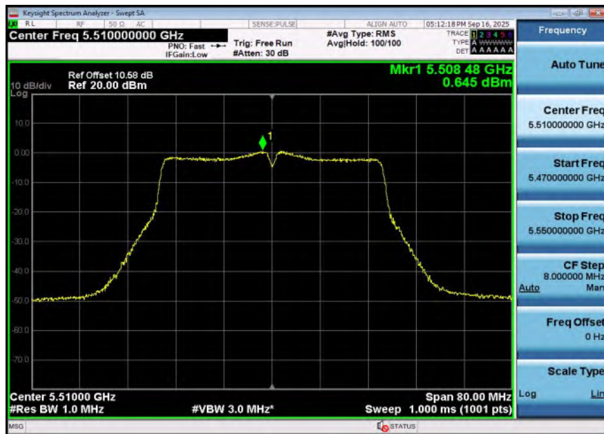
11N40SISO-Ant1-5510-PASS
