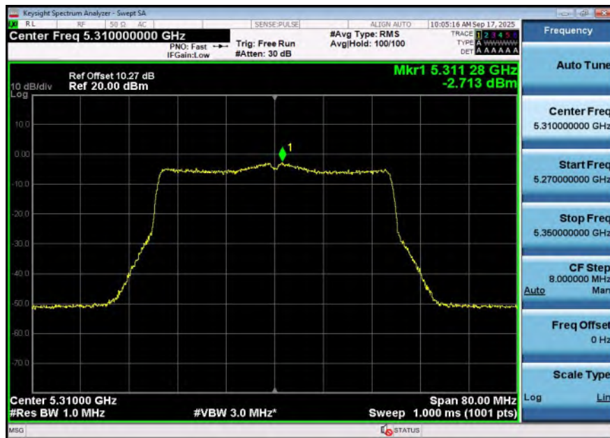
11AX40SISO-Ant1-5310-PASS
