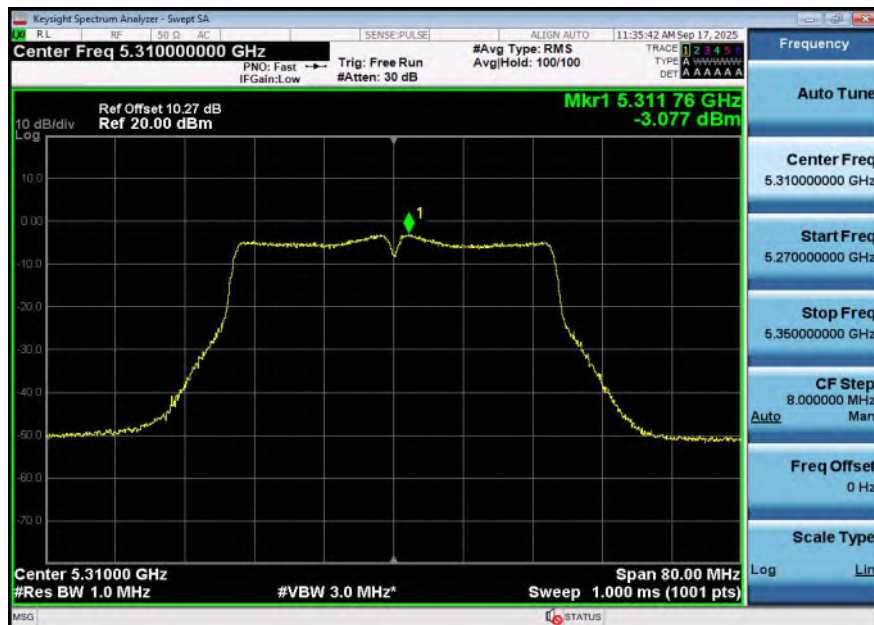
11N40SISO-Ant2-5310-PASS
