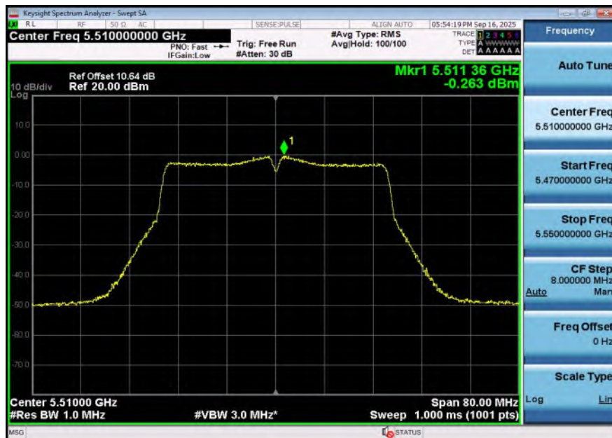
11AC40SISO-Ant1-5510-PASS
