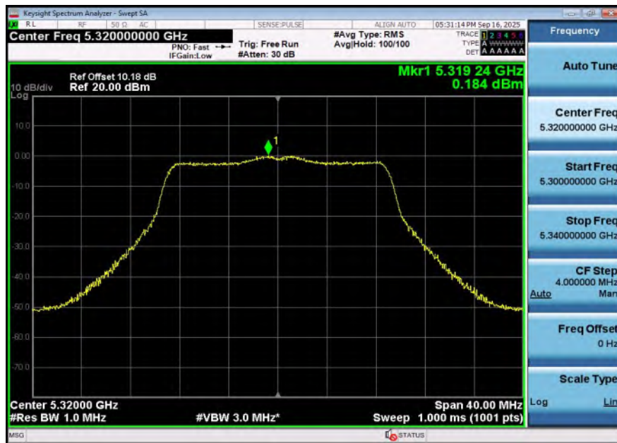
11AC20SISO-Ant1-5320-PASS
