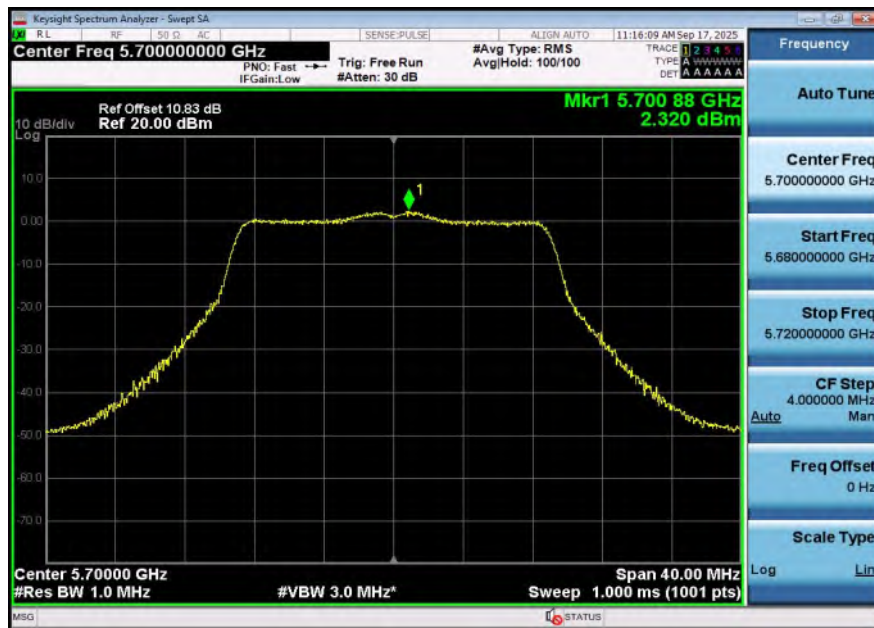
11N20SISO-Ant2-5700-PASS
