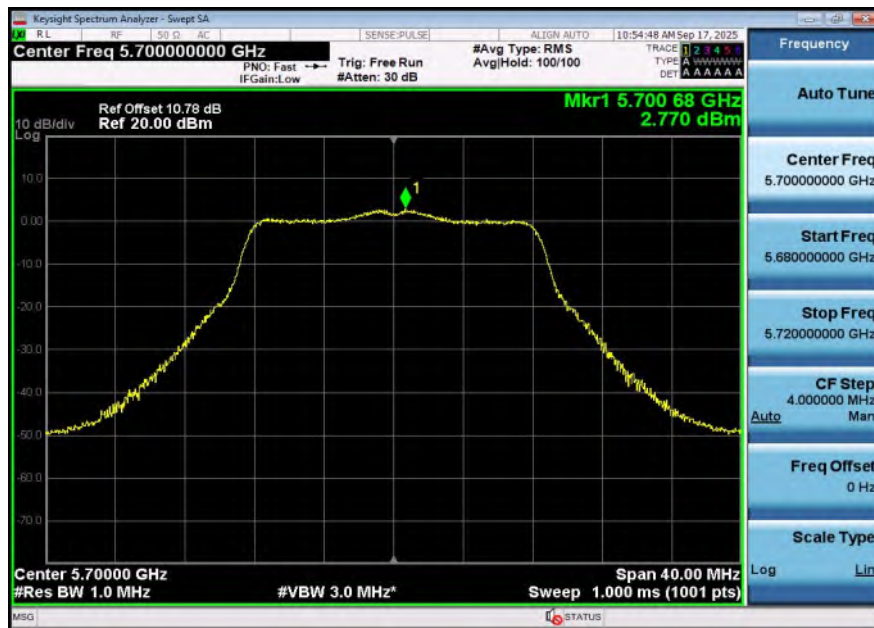
11A-Ant2-5700-PASS
