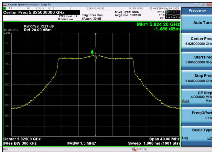
11AC20SISO-Ant1-5825-PASS
