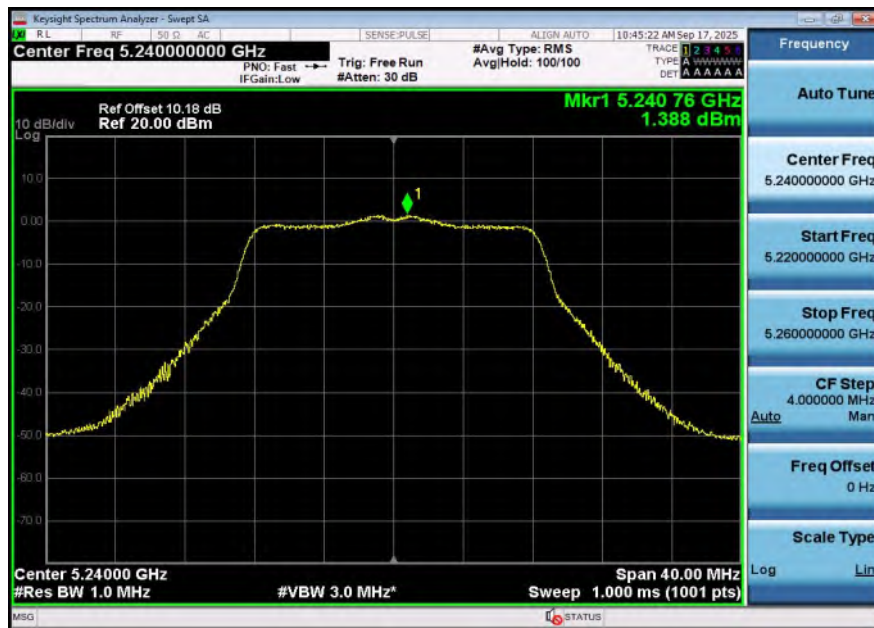
11A-Ant2-5240-PASS
