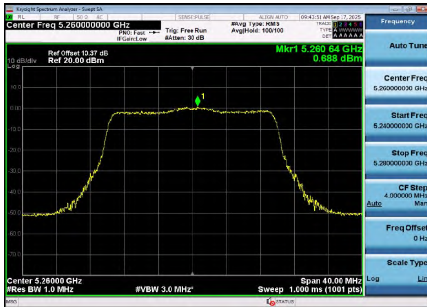
11AX20SISO-Ant1-5260-PASS
