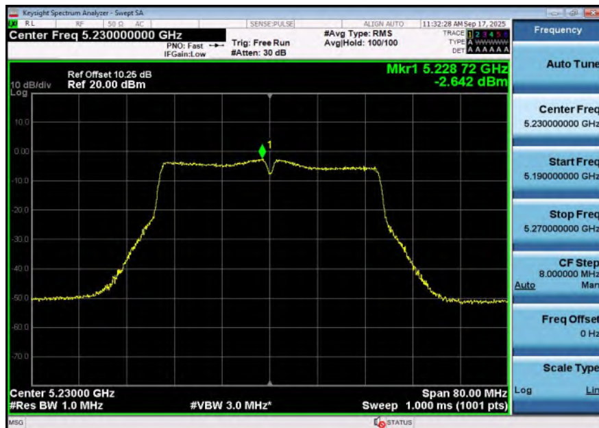
11N40SISO-Ant2-5230-PASS
