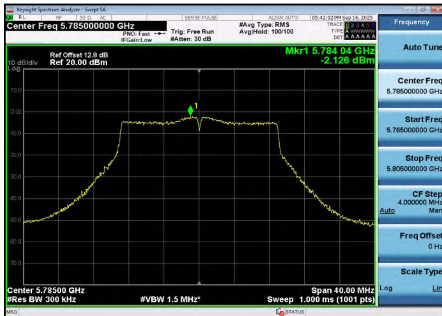
11AC20SISO-Ant1-5785-PASS
