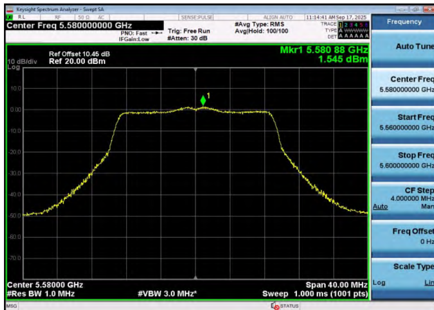
11N20SISO-Ant2-5580-PASS
