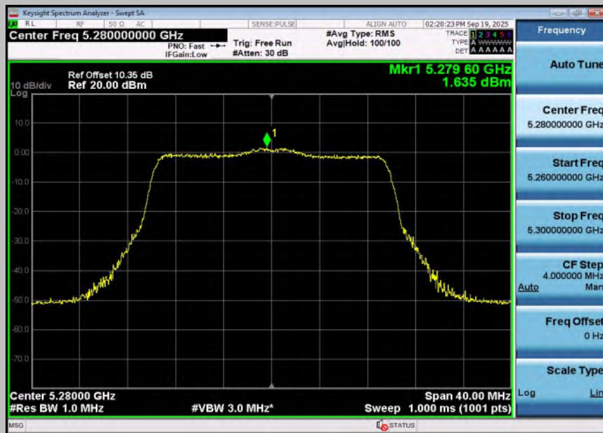
11BE20SISO-Ant1-5280-PASS
