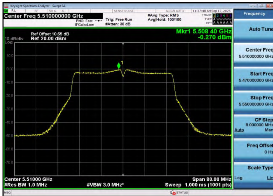
11N40SISO-Ant2-5510-PASS
