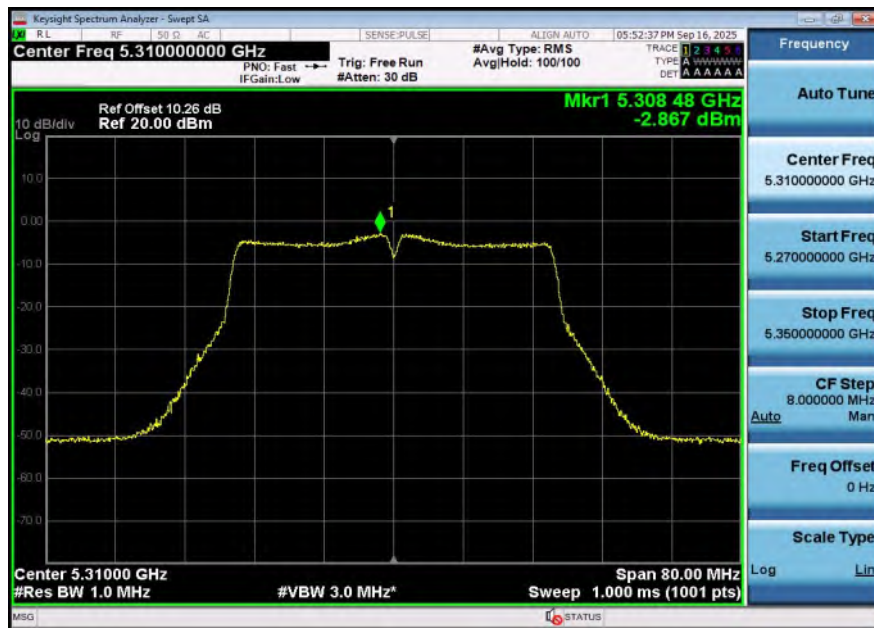
11AC40SISO-Ant1-5310-PASS
