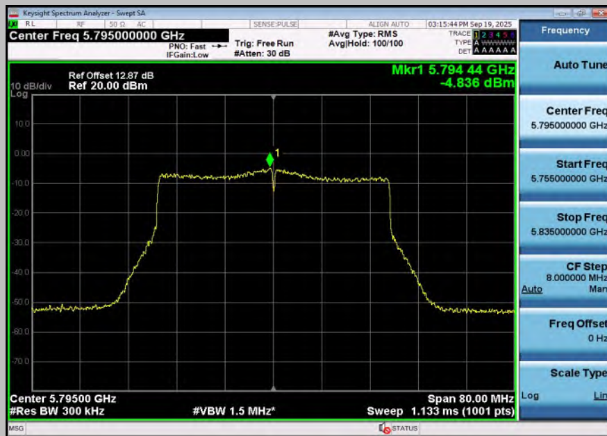
11BE40SISO-Ant1-5795-PASS
