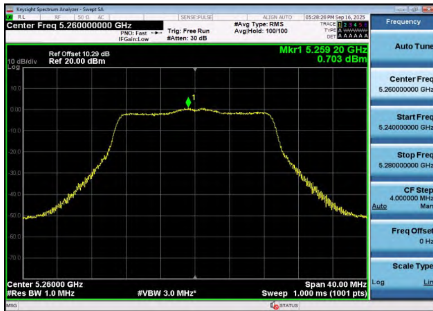
11AC20SISO-Ant1-5260-PASS
