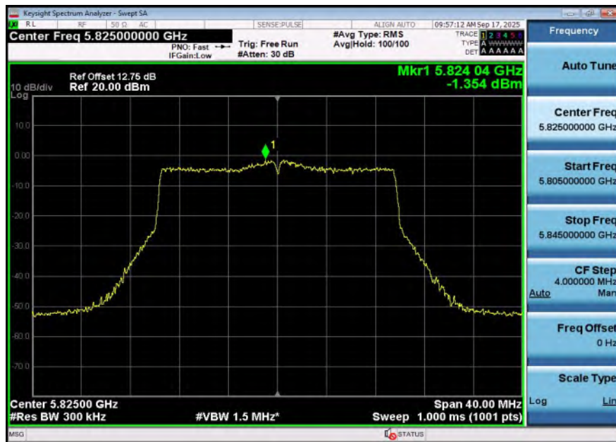
11AX20SISO-Ant1-5825-PASS
