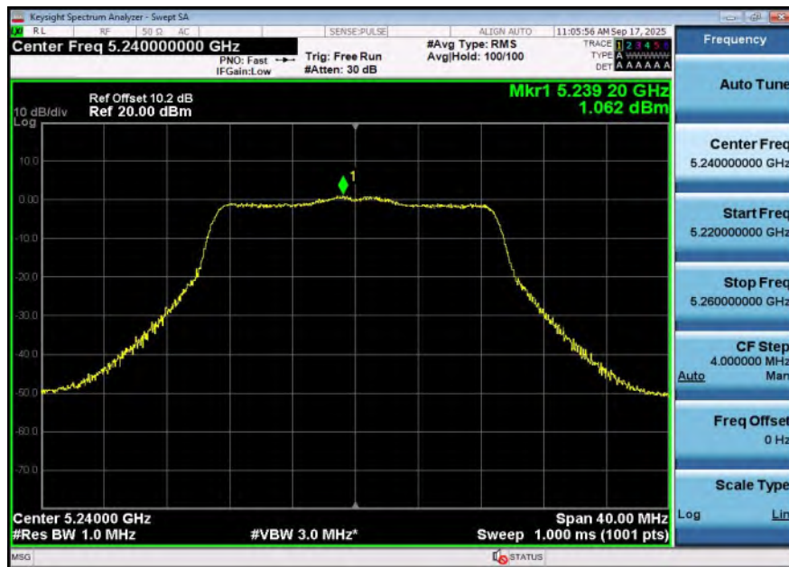
11N20SISO-Ant2-5240-PASS
