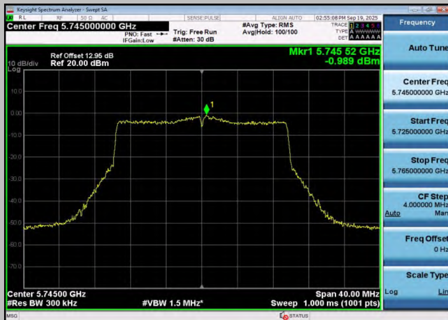
11BE20SISO-Ant1-5745-PASS
