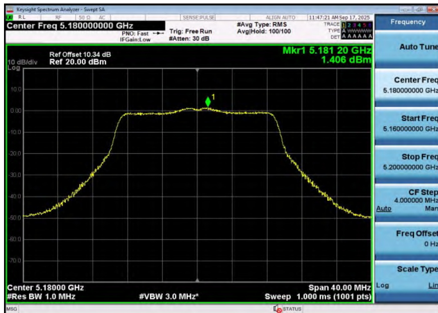
11AC20SISO-Ant2-5180-PASS
