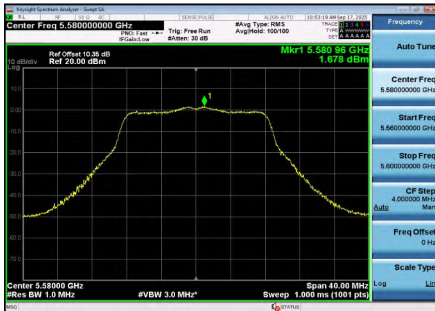
11A-Ant2-5580-PASS
