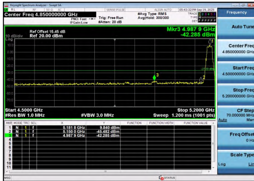
11AC20SISO-Ant1-5180-PASS
