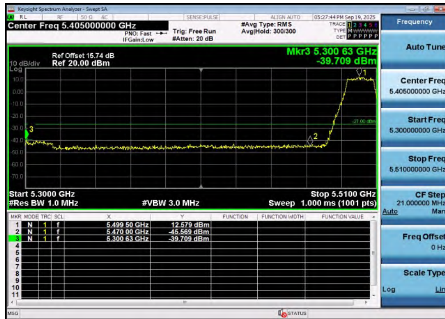
11A-Ant1-5500-PASS
