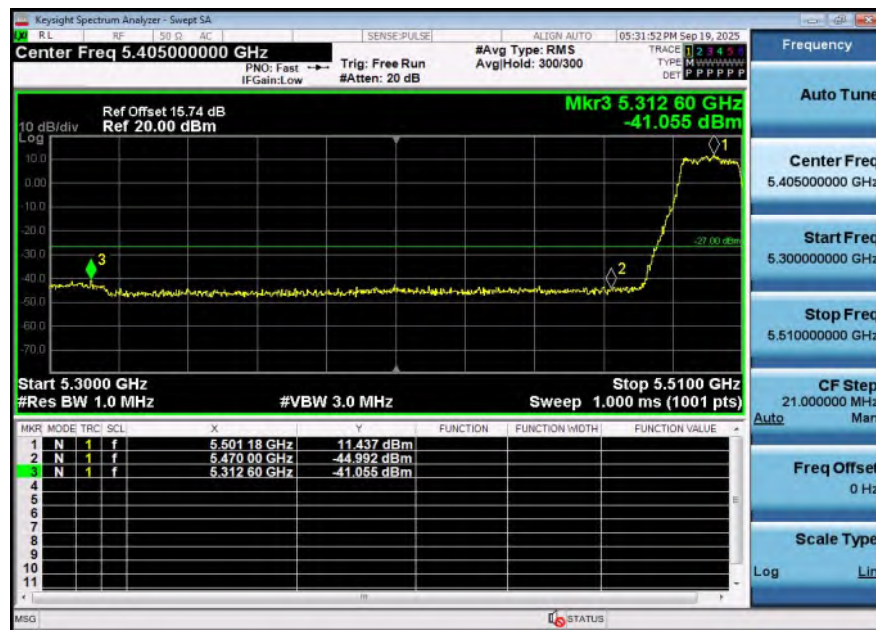
11N20SISO-Ant1-5500-PASS
