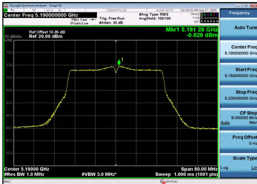
11AC40SISO-Ant2-5190-PASS
