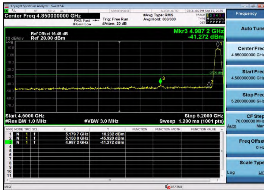
11N20SISO-Ant1-5180-PASS
