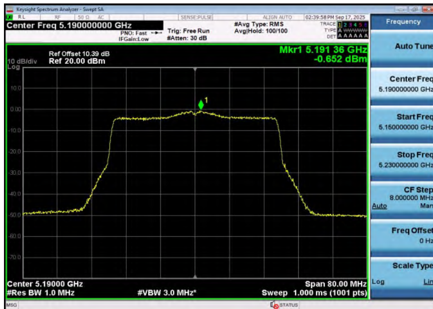
11AX40SISO-Ant2-5190-PASS
