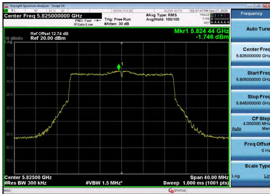
11AX20SISO-Ant2-5825-PASS
