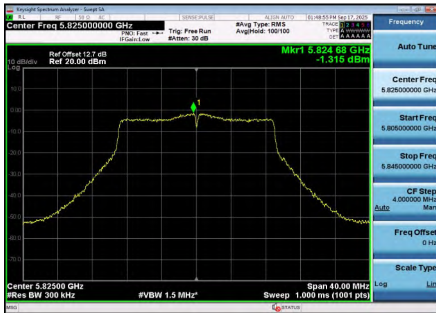
11AC20SISO-Ant2-5825-PASS
