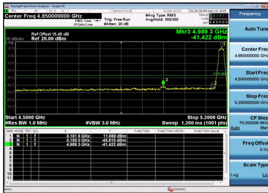
11A-Ant1-5180-PASS
