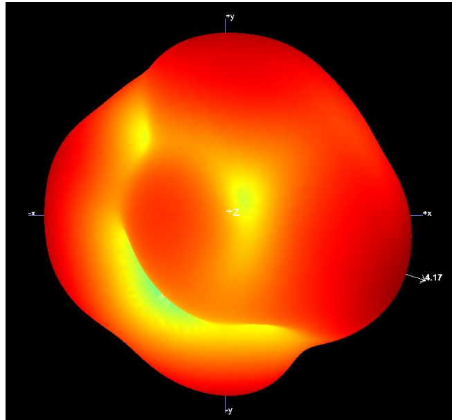
B1.1 3D Pattern for 2400MHz
