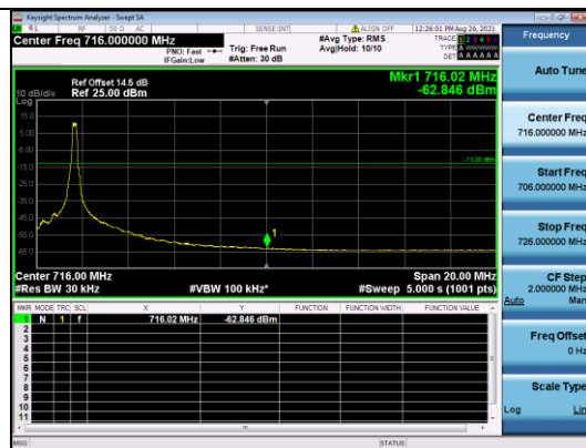
CATM1 B12-10M-High CH-BE-QPSK-1 RB MAX
