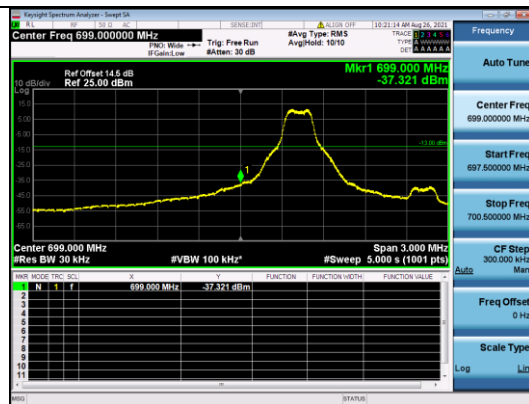
CATM1 B12-3M-Low CH-BE-QPSK-Full RB 0
