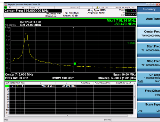
CATM1 B12-5M-High CH-BE-Q16-Full RB 0
