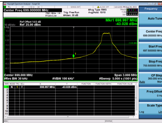
CATM1 B12-10M-Low CH-BE-QPSK-Full RB 0
