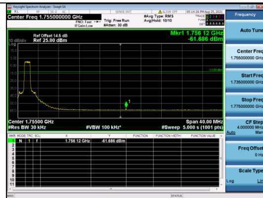
CATM1 B4-20M-High CH-BE-Q16-Full RB 0
