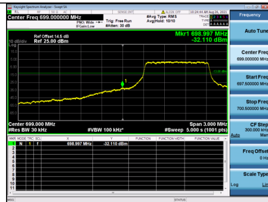
CATM1 B12-3M-Low CH-BE-Q16-Full RB 0
