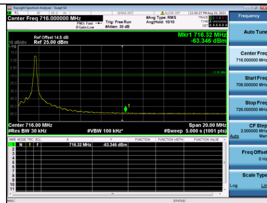
CATM1 B12-10M-High CH-BE-Q16-1 RB MAX
