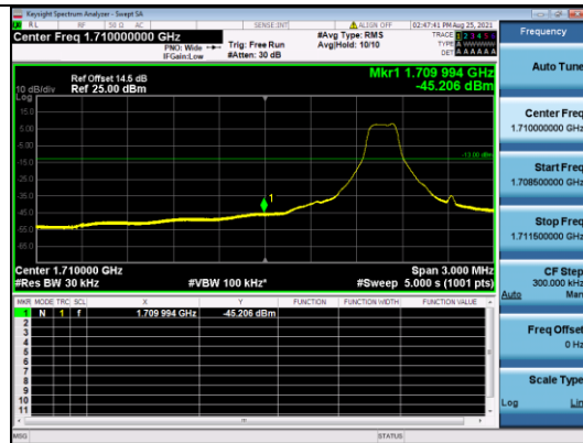
CATM1 B4-10M-Low CH-BE-QPSK-Full RB 0
