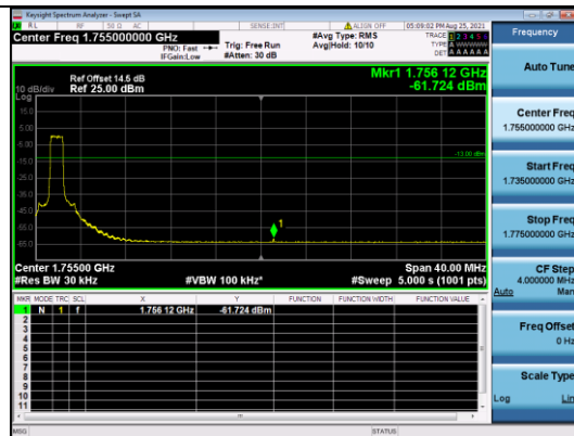
CATM1 B4-20M-High CH-BE-QPSK-Full RB 0
