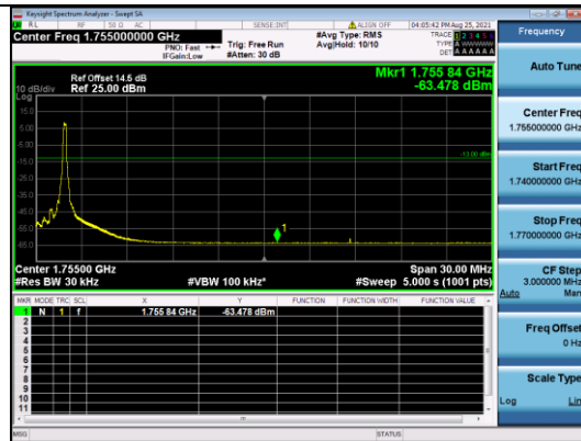
CATM1 B4-15M-High CH-BE-QPSK-Full RB 0
