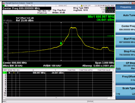
CATM1 B12-5M-Low CH-BE-QPSK-1 RB 0
