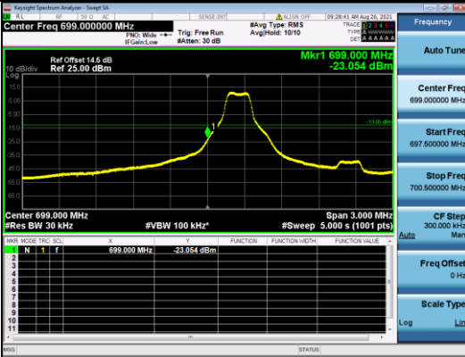
CATM1 B12-1.4M-Low CH-BE-QPSK-Full RB 0
