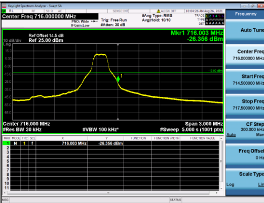
CATM1 B12-1.4M-High CH-BE-QPSK-1 RB MAX
