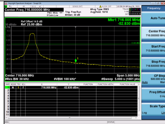
CATM1 B12-3M-High CH-BE-Q16-Full RB 0
