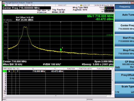
CATM1 B12-3M-High CH-BE-QPSK-Full RB 0
