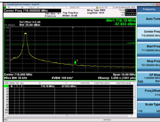
CATM1 B12-5M-High CH-BE-QPSK-Full RB 0
