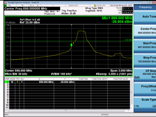
CATM1 B12-1.4M-Low CH-BE-Q16-Full RB 0
