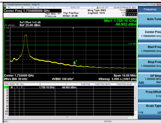
CATM1 B4-5M-High CH-BE-QPSK-Full RB 0
