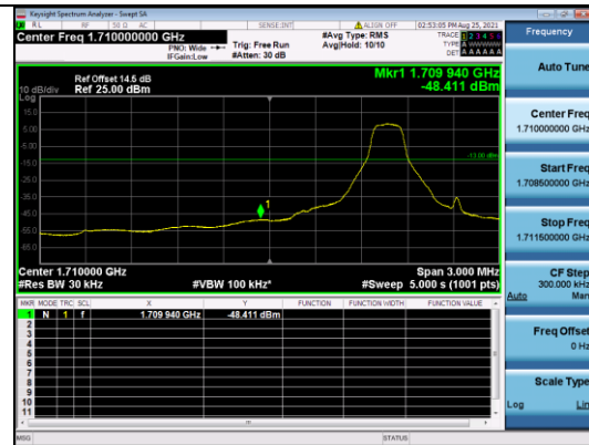
CATM1 B4-10M-Low CH-BE-Q16-Full RB 0
