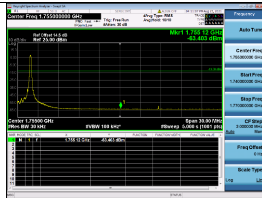
CATM1 B4-15M-High CH-BE-Q16-Full RB 0
