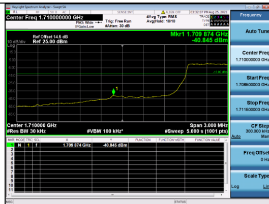
CATM1 B4-15M-Low CH-BE-QPSK-Full RB 0
