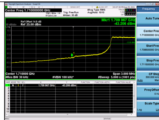
CATM1 B4-15M-Low CH-BE-Q16-Full RB 0
