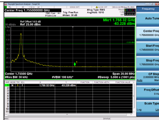
CATM1 B4-10M-High CH-BE-Q16-1 RB MAX
