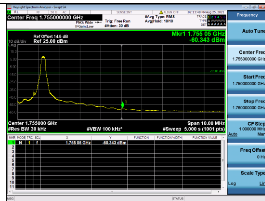
CATM1 B4-5M-High CH-BE-Q16-Full RB 0
