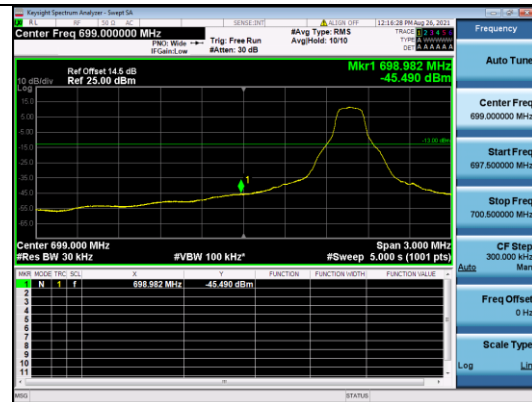
CATM1 B12-10M-Low CH-BE-Q16-Full RB 0
