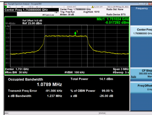
LTE CATM1 B4-5M-High CH-OBW-Q16
