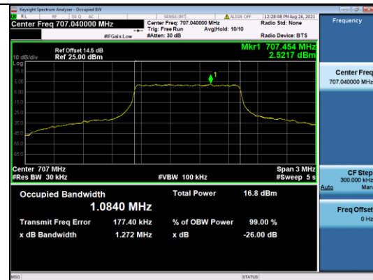
LTE CATM1 B12-10M-High CH-OBW-Q16
