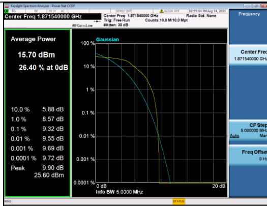
LTE CATM1 B2-20M-High CH-PAPR-QPSK
