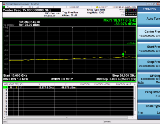
CATM1 B4-1.4M-Mid CH-CSE-1-QPSK-1 RB 0
