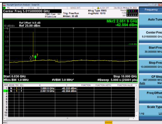
CATM1 B2-15M-Mid CH-CSE-1-QPSK-1 RB 0
