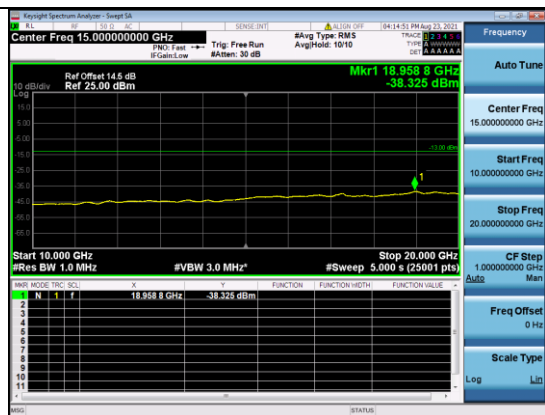
CATM1 B2-3M-High CH-CSE-2-QPSK-1 RB 0
