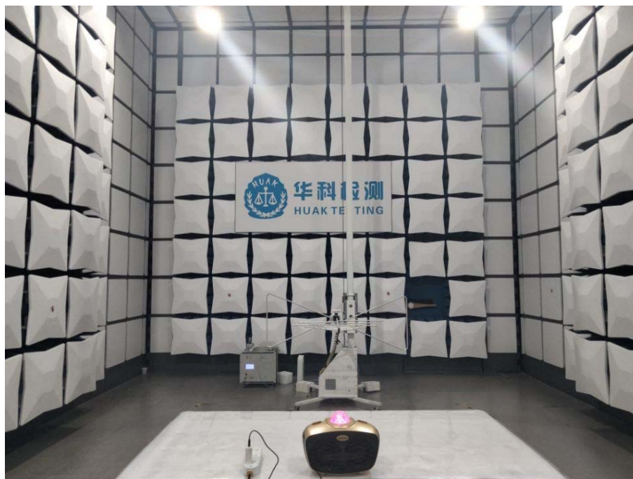
MI-S112B Radiated Emissions
