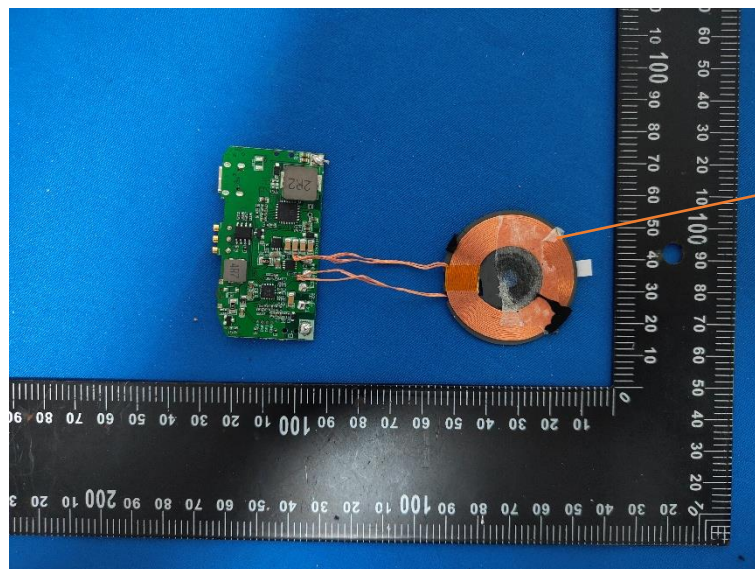
Phone coil antenna
