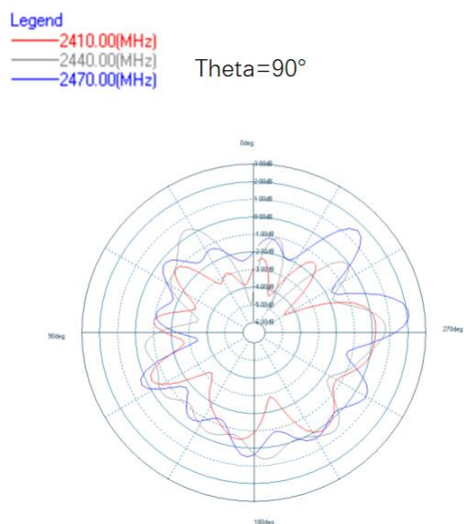
Figure 4: 3D Patterns – XY Plane
