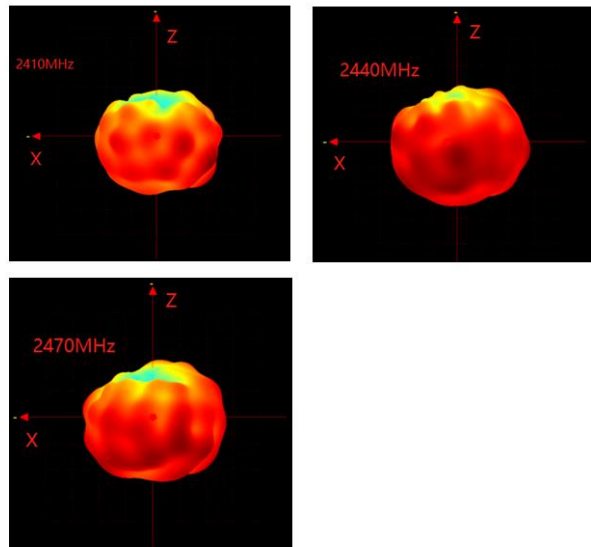
Figure 2: 3D Patterns – XZ Plane
