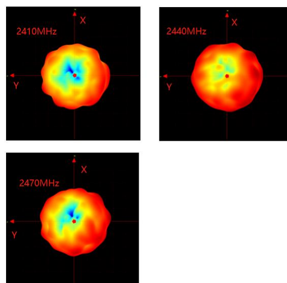
Figure 4: 3D Patterns – XY Plane
