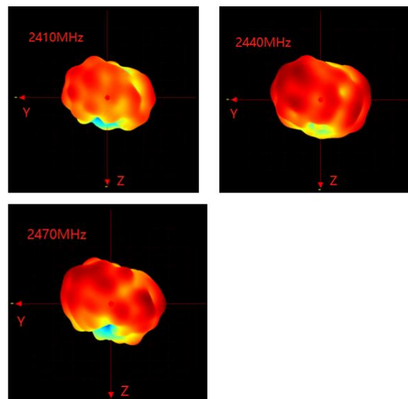
Figure 3: 3D Patterns – YZ Plane
