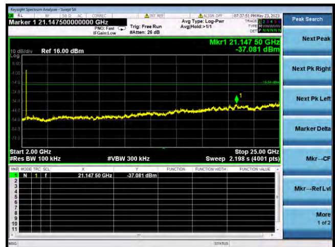
802.11g CHANNEL 1, SPURIOUS 2 GHz ~ 25 GHz
