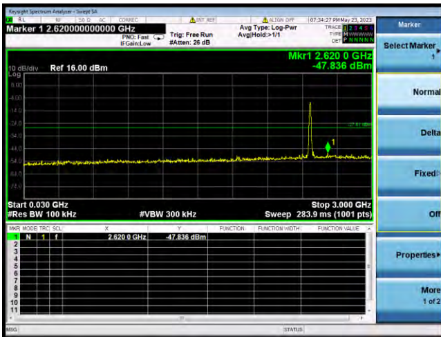
802.11b CHANNEL 13, SPURIOUS 30 MHz ~ 3 GHz
