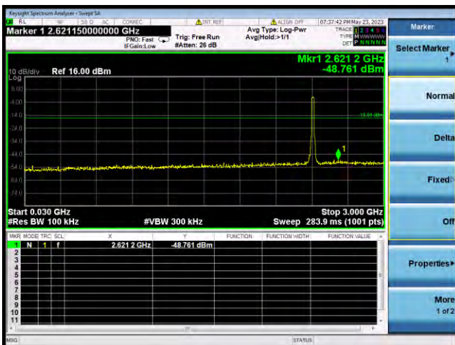
802.11g CHANNEL 1, SPURIOUS 30 MHz ~ 3 GHz
