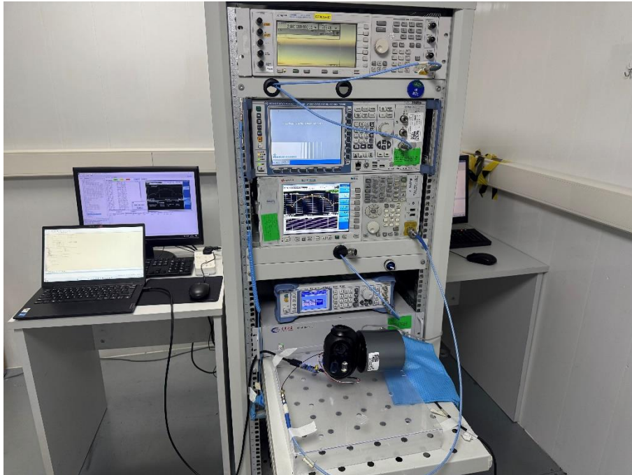
Conducted Test-BLE/WIF
