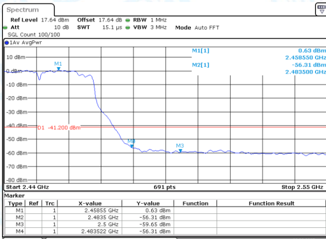
11AX40MIMO-Ant1-2452-PASS
