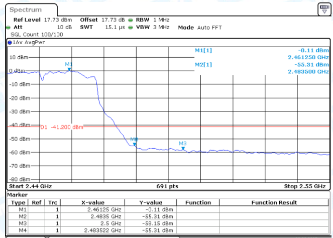
11AX40MIMO-Ant2-2452-PASS
