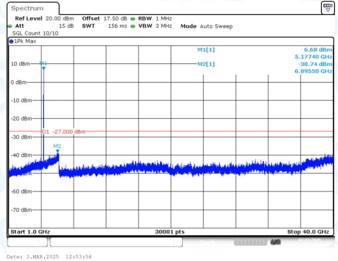
11A-CDD-Ant2-5180-1000~40000-PASS
