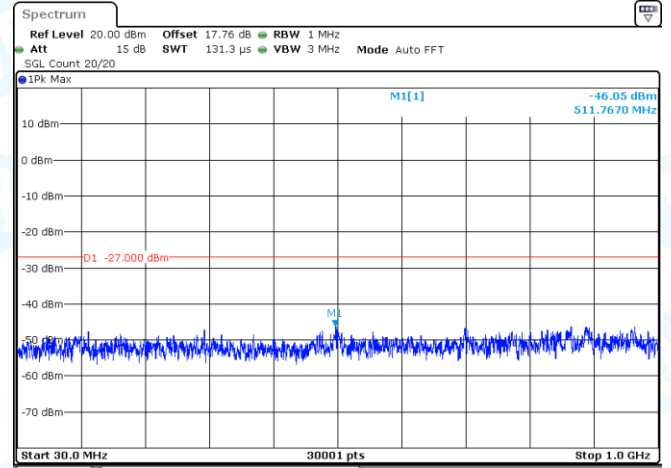
11AX80MIMO-Ant2-5775-30~1000-PASS
