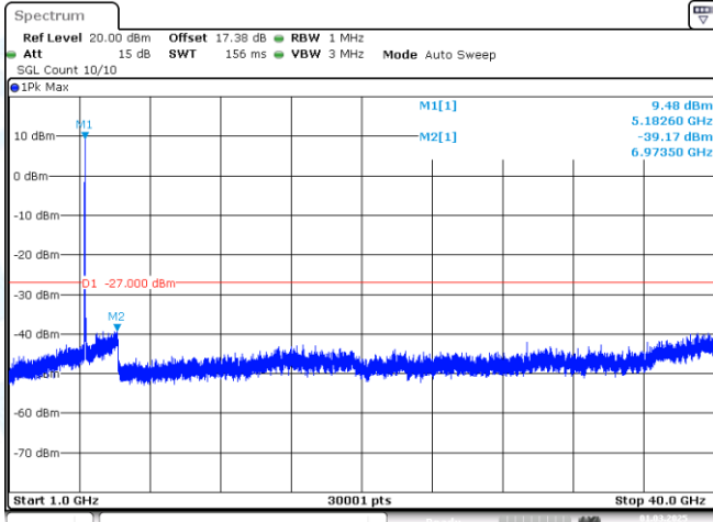
11AX40MIMO-Ant1-5190-1000~40000-PASS
