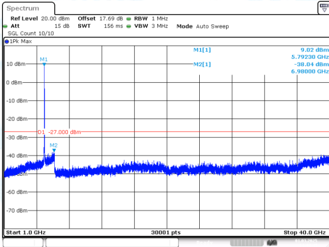
11AC40MIMO-Ant1-5795-1000~40000-PASS
