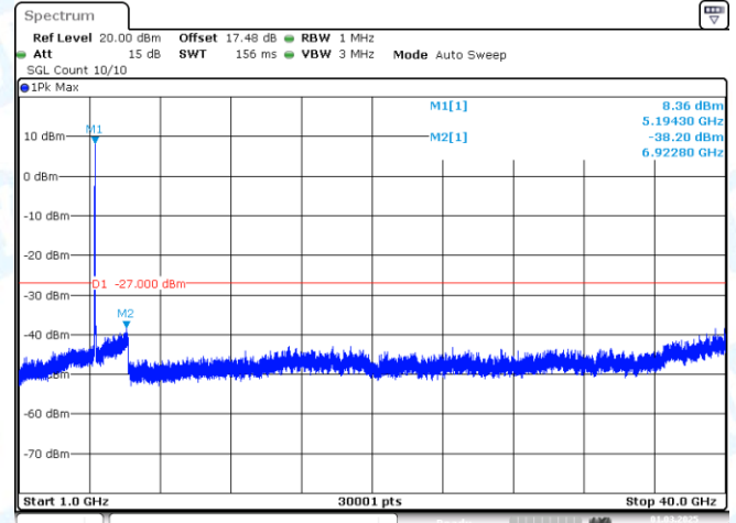
11AX40MIMO-Ant2-5190-1000~40000-PASS
