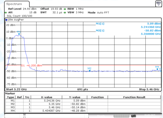
11AX20MIMO-Ant2-5240-PASS
