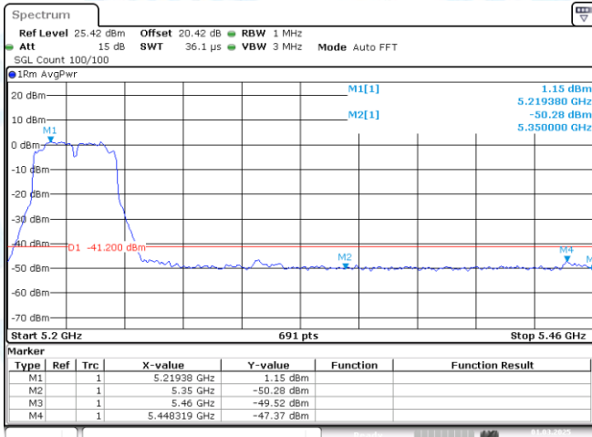
11AC40MIMO-Ant1-5230-PASS
