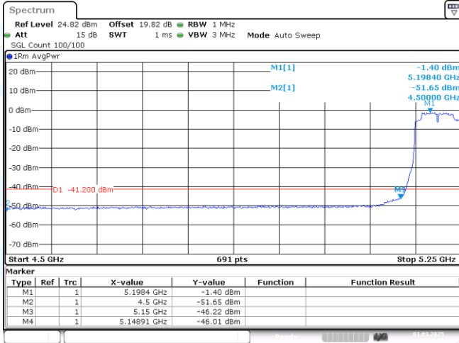
11AC80MIMO-Ant2-5210-PASS
