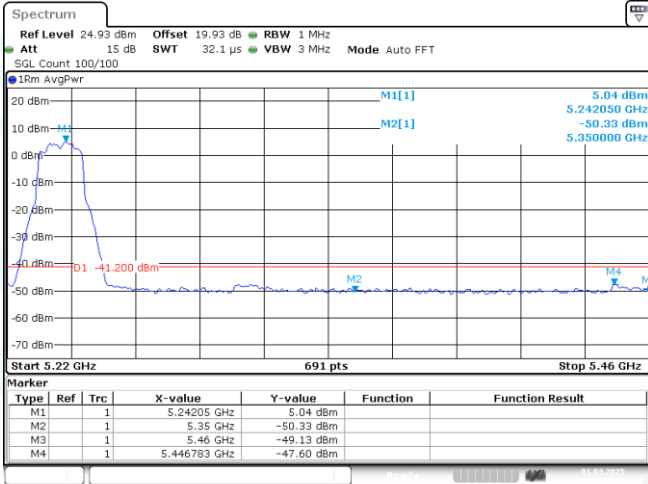
11A-CDD-Ant2-5240-PASS
