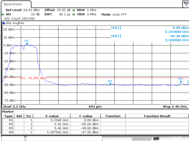
11N40MIMO-Ant2-5230-PASS
