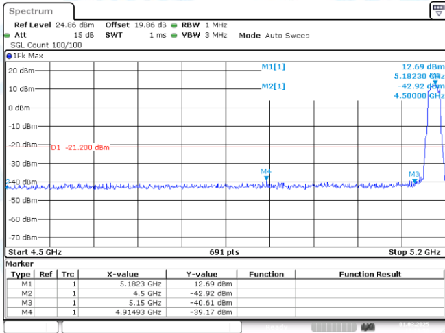
11AX20MIMO-Ant2-5180-PASS
