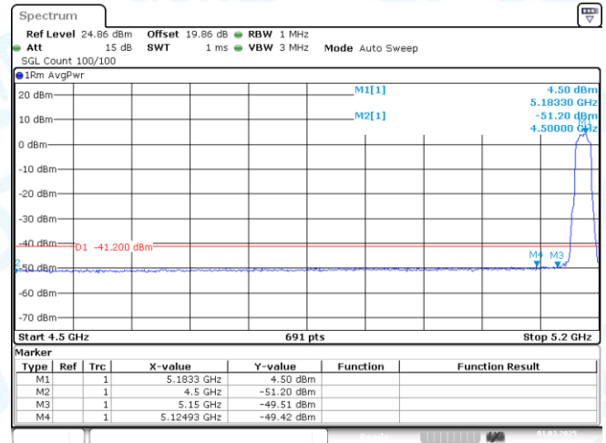
11AX20MIMO-Ant1-5180-PASS
