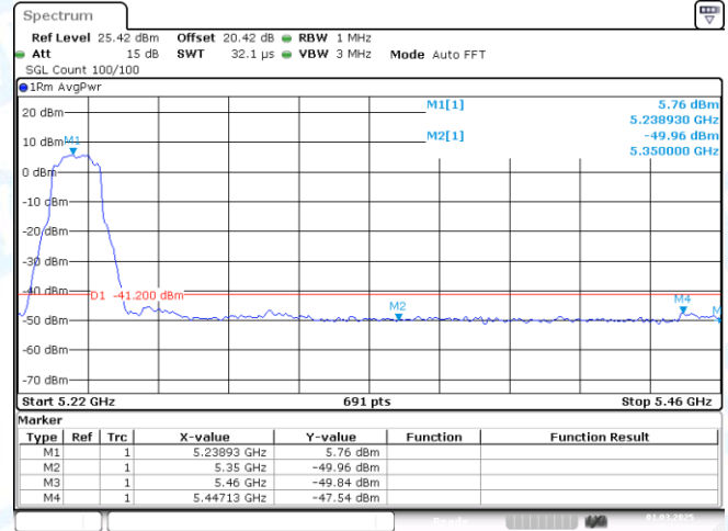
11A-CDD-Ant1-5240-PASS
