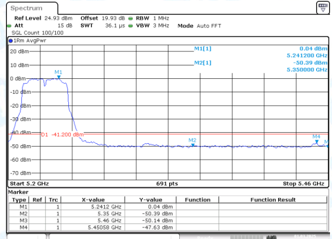
11AC40MIMO-Ant2-5230-PASS
