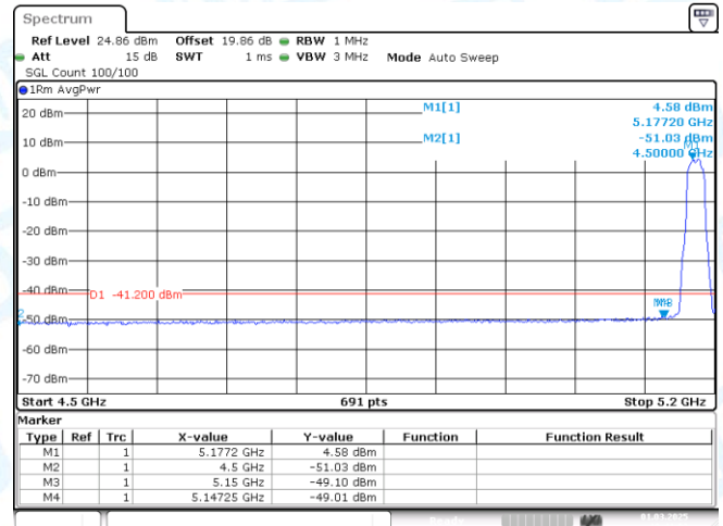
11AC20MIMO-Ant2-5180-PASS
