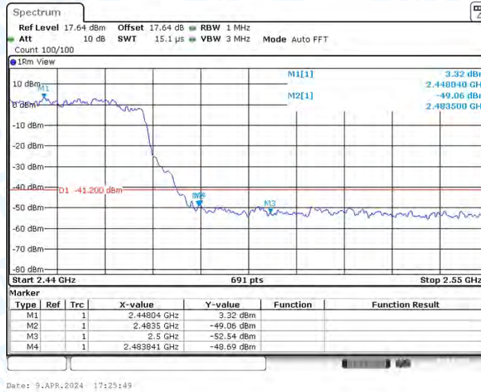
11AX40MIMO_Ant1_High_2452_Peak
