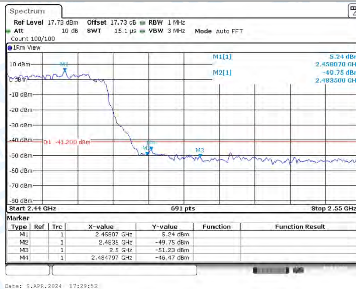
11AX40MIMO_Ant2_High_2452_Peak
