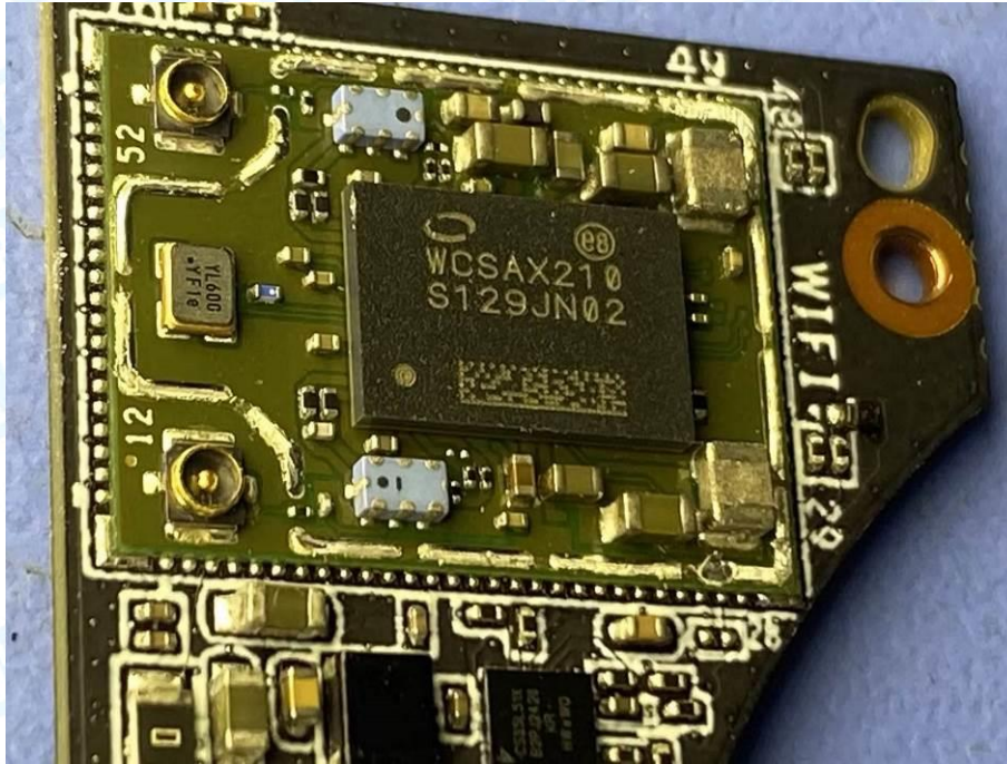
Photo 39 Appearance of PCB
