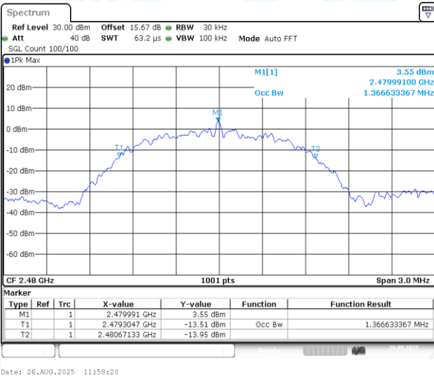
3DH5-Ant1-2480
