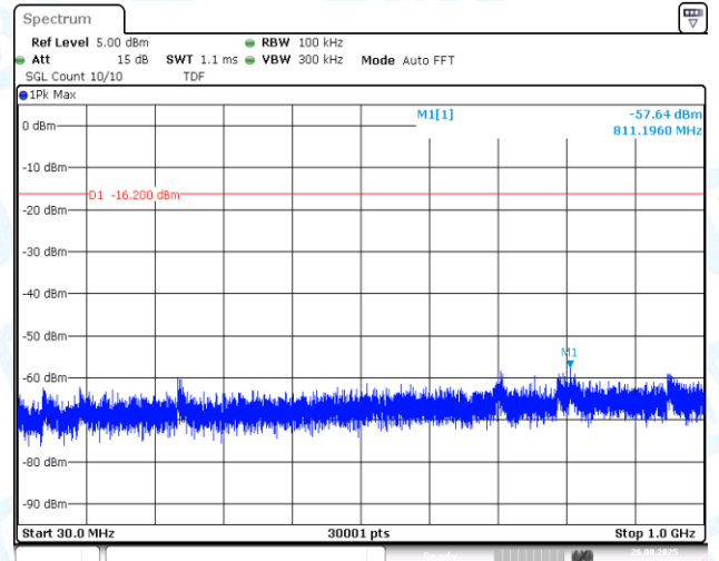
2DH5-Ant1-2441-30~1000-PASS
