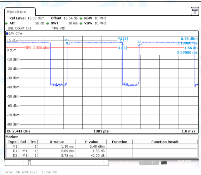
NTVN-3DH5-Ant1-2441
