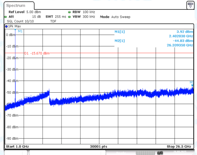
2DH5-Ant1-2402-0~Reference-PASS
