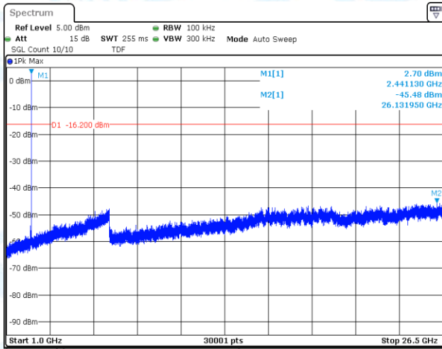
2DH5-Ant1-2441-0~Reference-PASS
