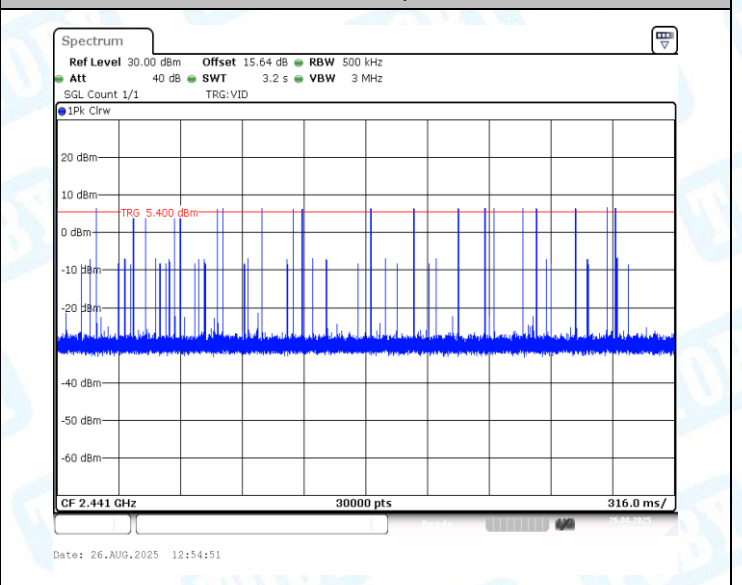
2DH3-Ant1-Hop-PASS
