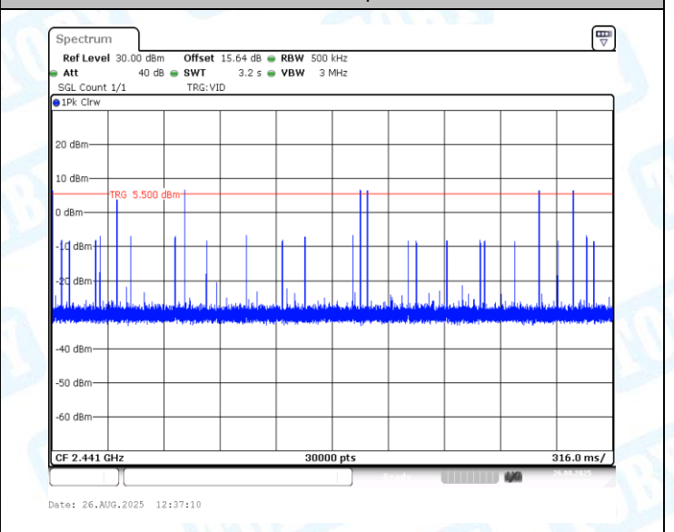
2DH5-Ant1-Hop-PASS
