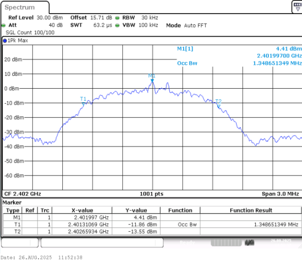
3DH5-Ant1-2402
