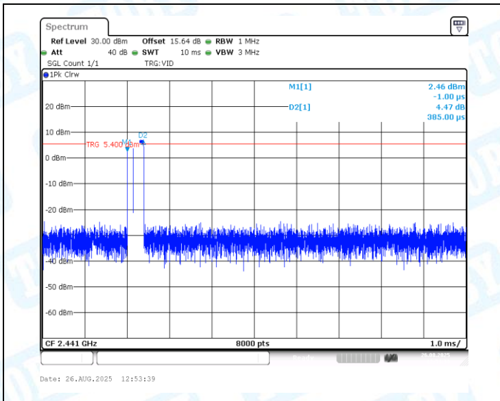
2DH1-Ant1-Hop-PASS
