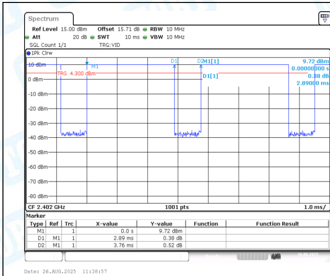
NTNV-DH5-Ant1-2402
