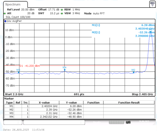
3DH5-Ant1-2402-PASS
