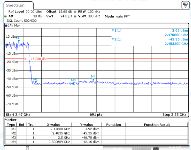
3DH5-Ant1-2480-PASS
