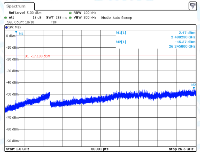
2DH5-Ant1-2480-0~Reference-PASS
