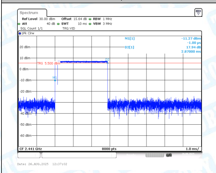
2DH5-Ant1-Hop-PASS
