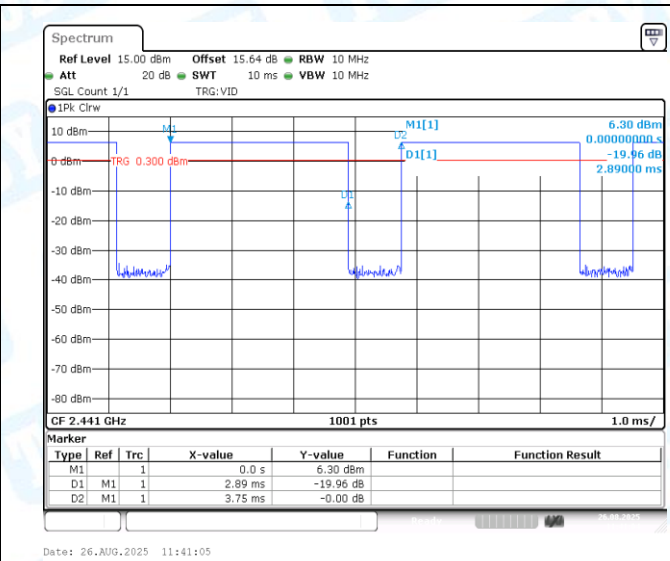
NTNV-DH5-Ant1-2441
