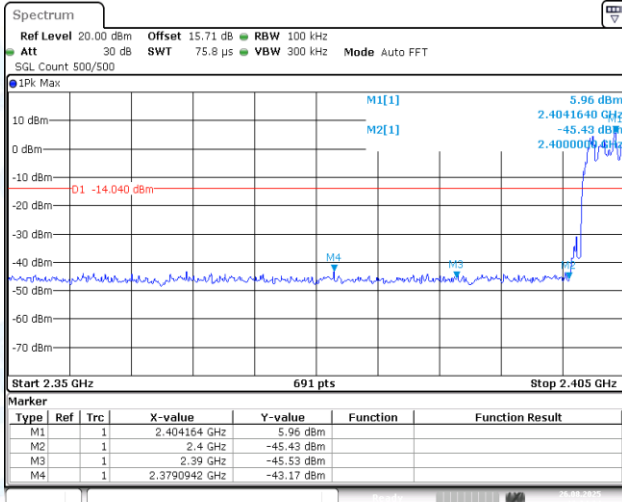
2DH5-Ant1-Hop_2402-PASS
