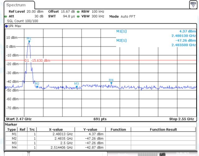
2DH5-Ant1-Hop_2480-PASS
