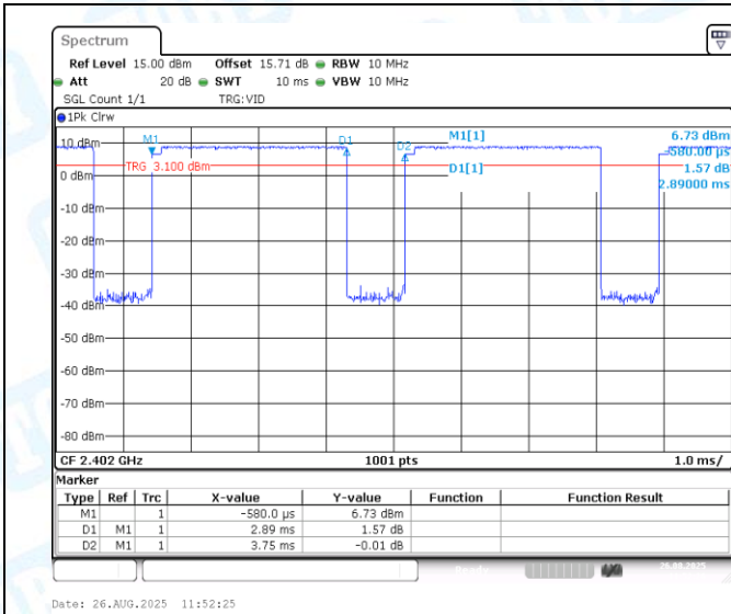
NTVN-3DH5-Ant1-2402
