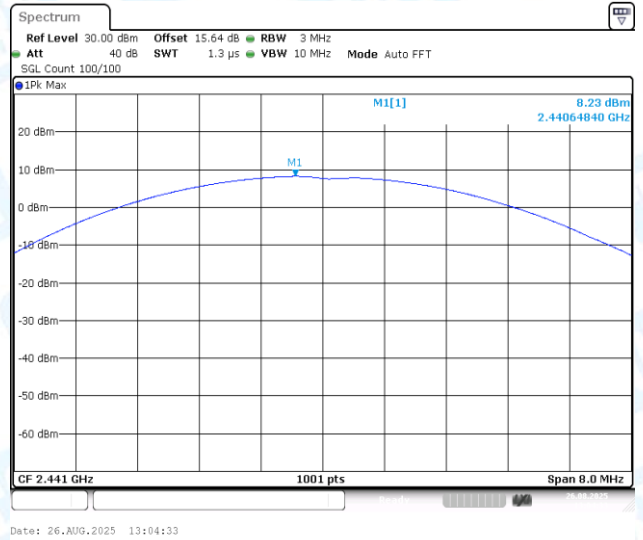
3DH5-Ant1-2441-PASS
