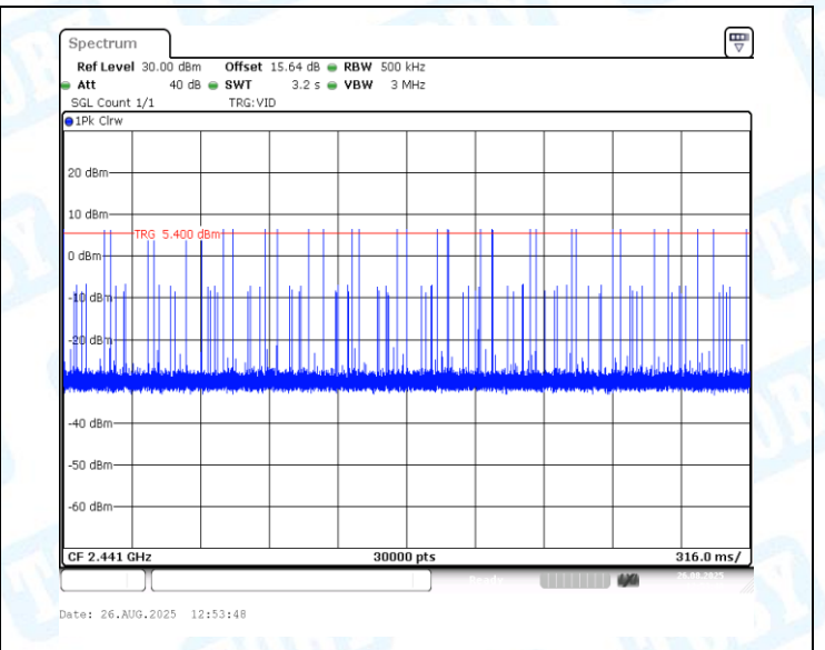
2DH1-Ant1-Hop-PASS
