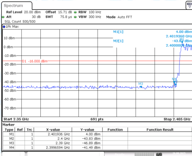
3DH5-Ant1-2402-PASS
