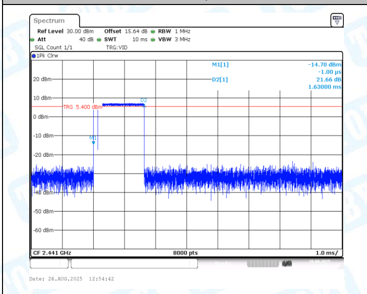
2DH3-Ant1-Hop-PASS
