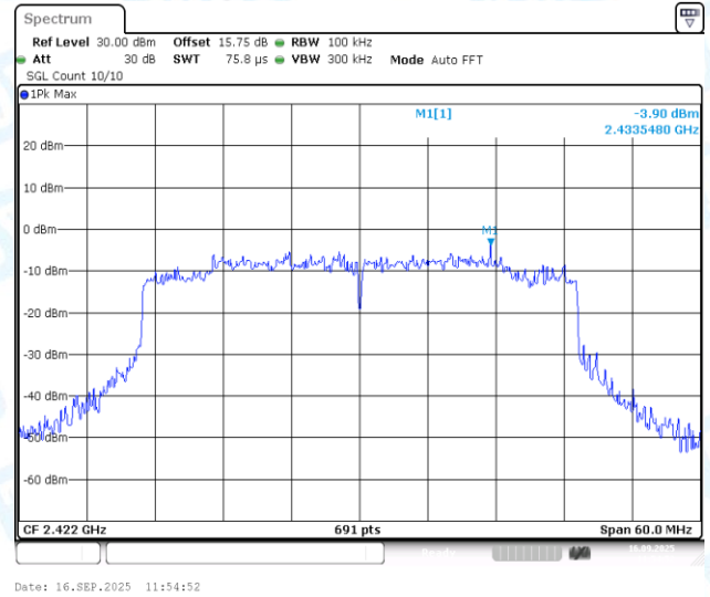
11AX40MIMO-Ant2-2422-0~Reference-PASS
