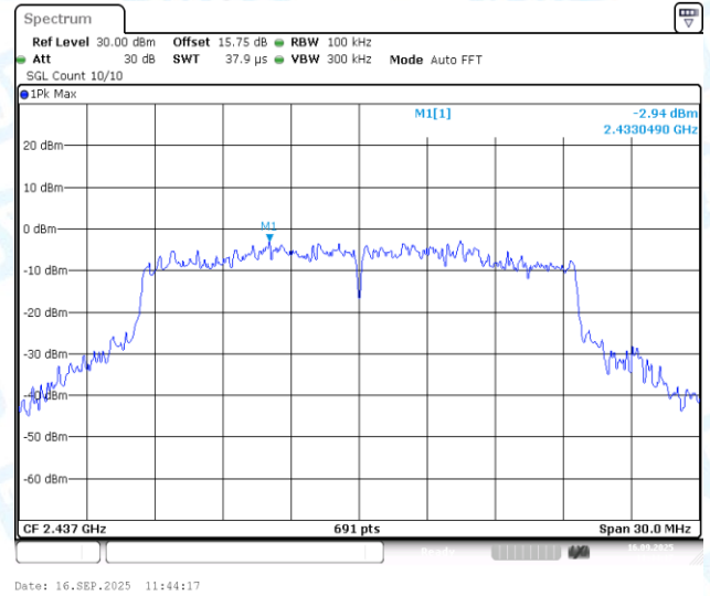
11AX20MIMO-Ant2-2437-0~Reference-PASS
