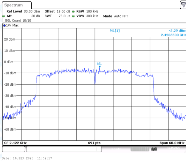
11AX40MIMO-Ant1-2422-0~Reference-PASS
