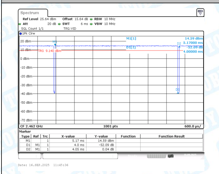
NTVN-11AX20MIMO-Ant1-2462
