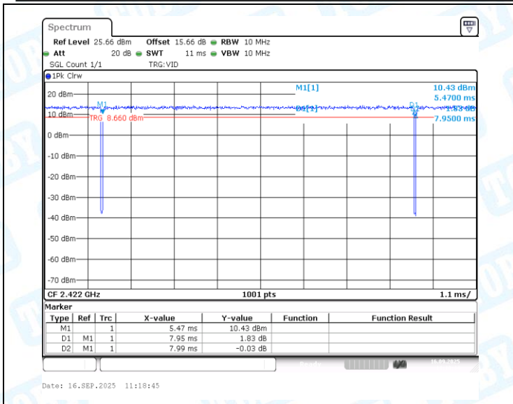
NTNV-11N40MIMO-Ant1-2422
