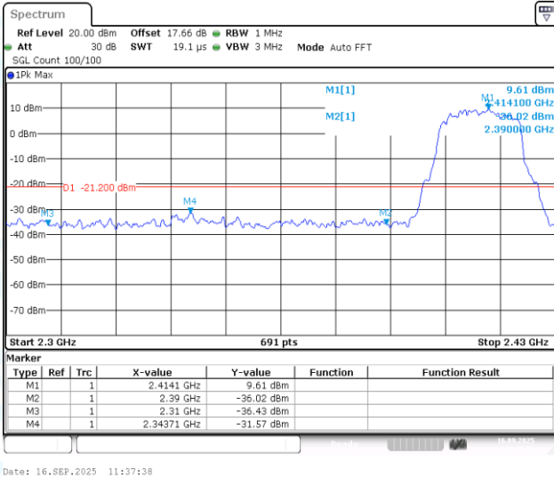
11AX20MIMO-Ant1-2412-PASS
