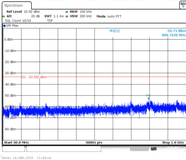
11AX20MIMO-Ant1-2437-30~1000-PASS
