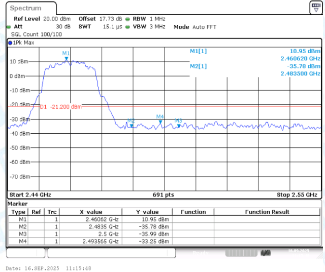
11N20MIMO-Ant2-2462-PASS
