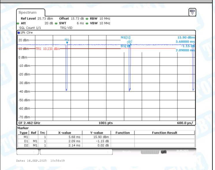
NTNV-11G-CDD-Ant2-2462
