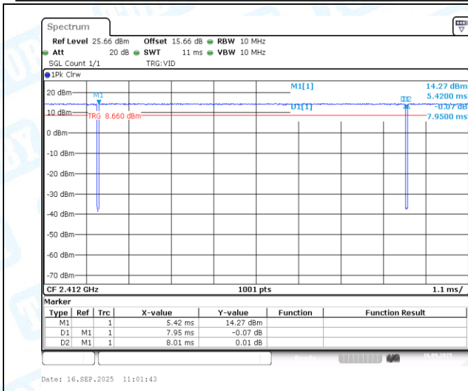
NTNV-11N20MIMO-Ant1-2412
