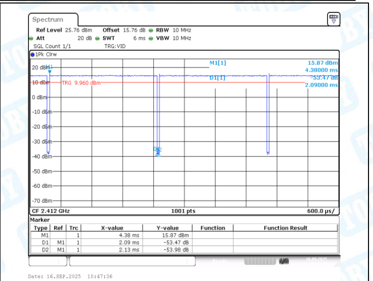
NTNV-11G-CDD-Ant2-2412
