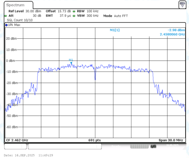
11AX20MIMO-Ant2-2462-0~Reference-PASS
