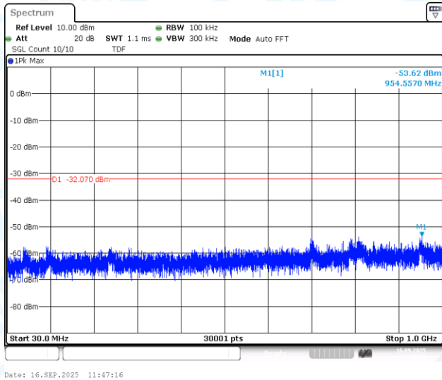
11AX20MIMO-Ant1-2462-30~1000-PASS
