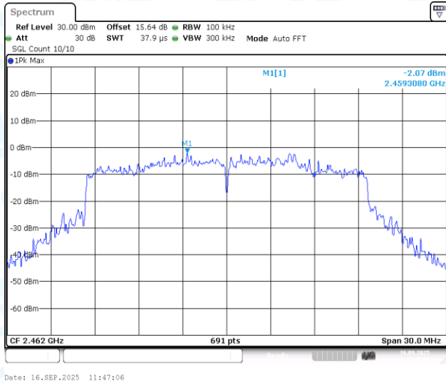
11AX20MIMO-Ant1-2462-0~Reference-PASS
