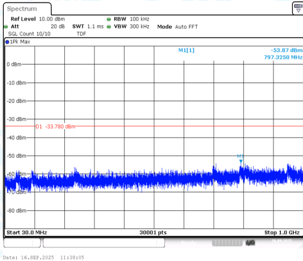
11AX20MIMO-Ant1-2412-30~1000-PASS
