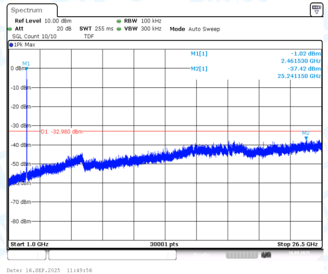
11AX20MIMO-Ant2-2462-1000~26500-PASS
