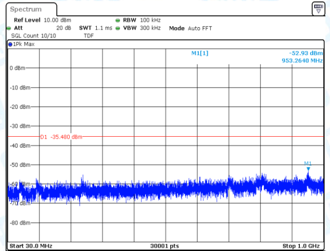
11AX40MIMO-Ant2-2452-0~Reference-PASS
