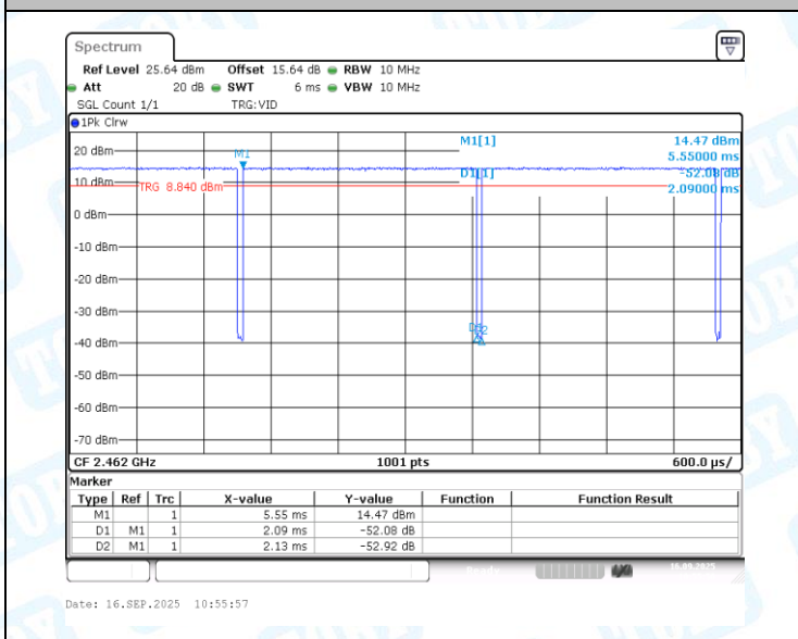
NTNV-11G-CDD-Ant1-2462
