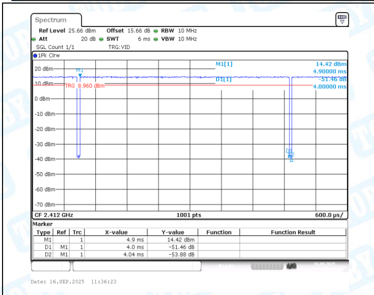
NTVN-11AX20MIMO-Ant1-2412
