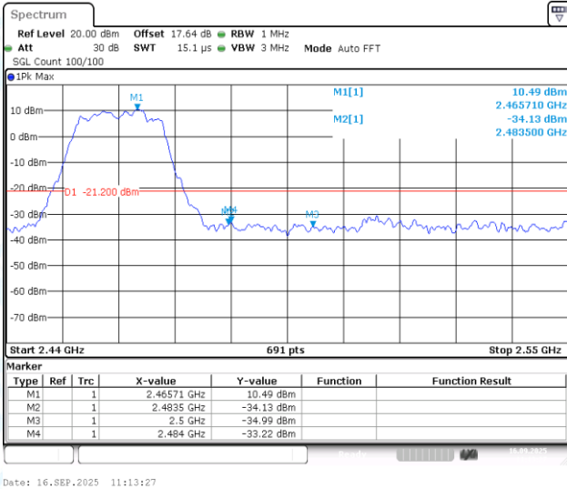
11N20MIMO-Ant1-2462-PASS
