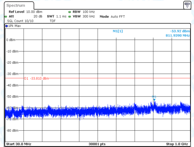
11AX40MIMO-Ant2-2437-0~Reference-PASS
