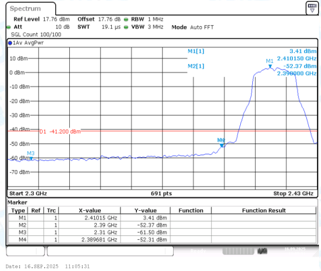
11N20MIMO-Ant2-2412-PASS
