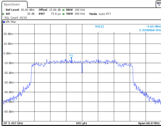
11AX40MIMO-Ant1-2437-0~Reference-PASS
