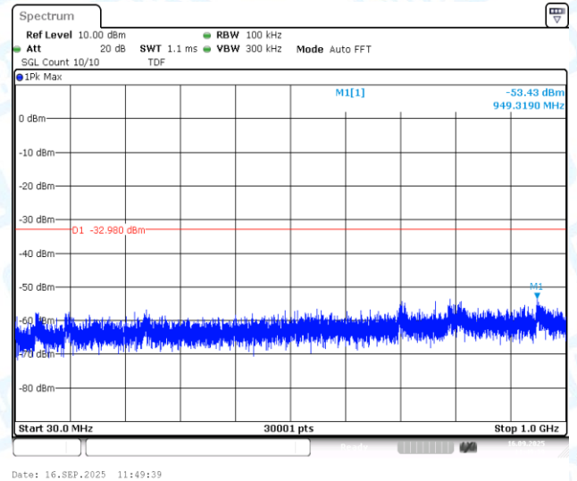
11AX20MIMO-Ant2-2462-30~1000-PASS
