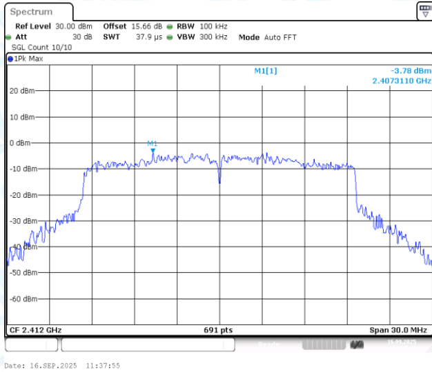
11AX20MIMO-Ant1-2412-0~Reference-PASS
