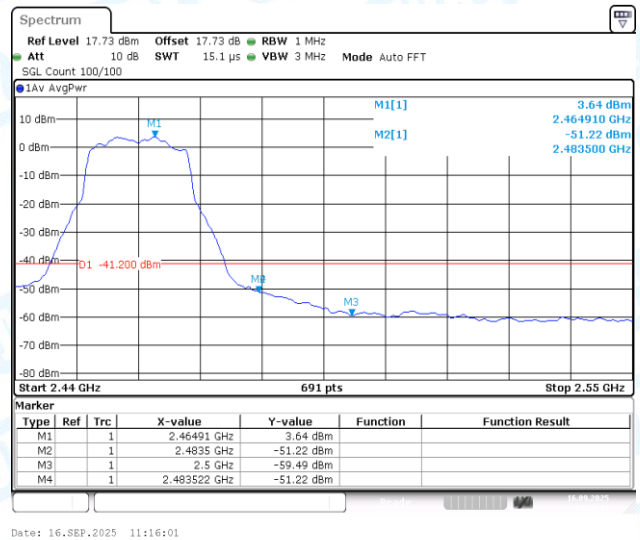
11N20MIMO-Ant2-2462-PASS
