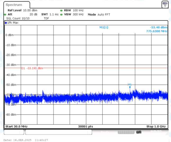
11AX20MIMO-Ant2-2412-30~1000-PASS
