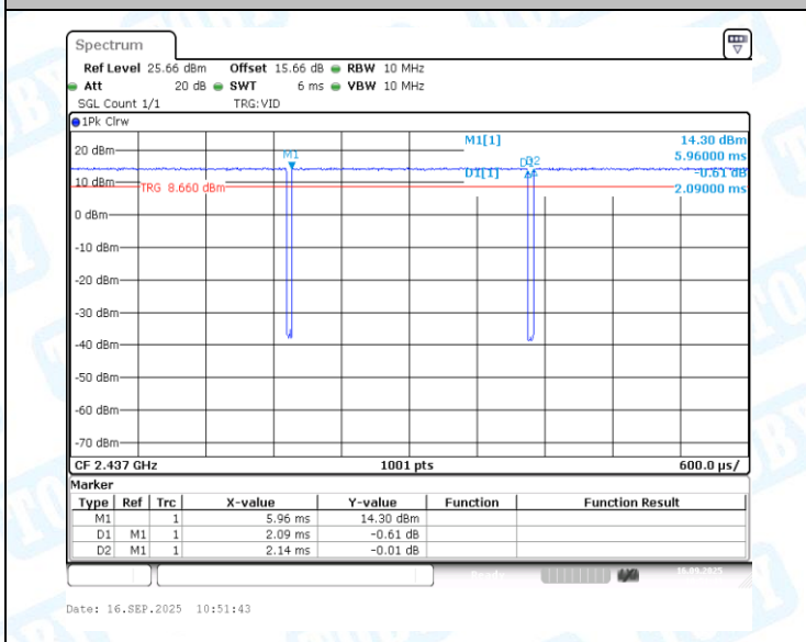
NTNV-11G-CDD-Ant1-2437
