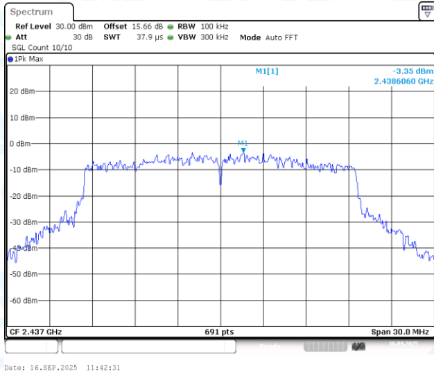
11AX20MIMO-Ant1-2437-0~Reference-PASS
