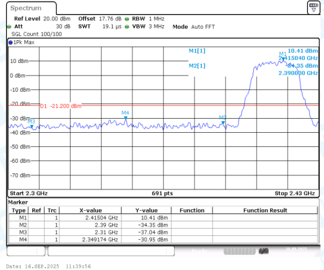
11AX20MIMO-Ant2-2412-PASS
