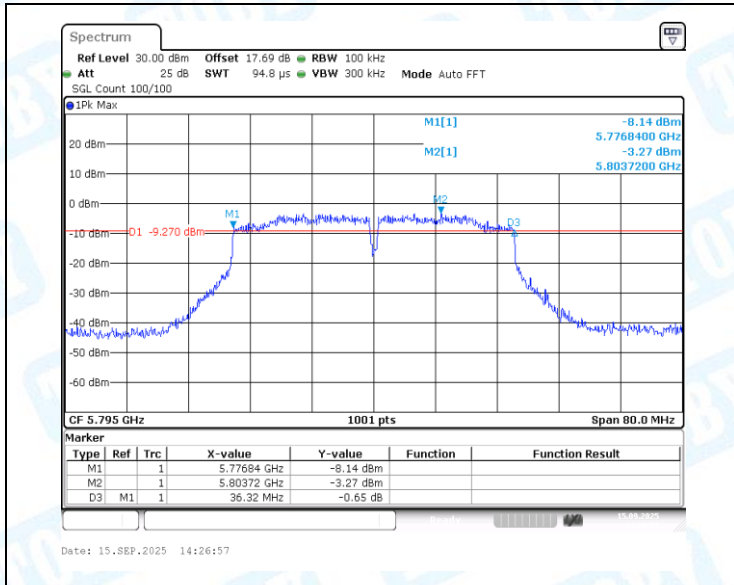
11AC40MIMO-Ant1-5795-PASS
