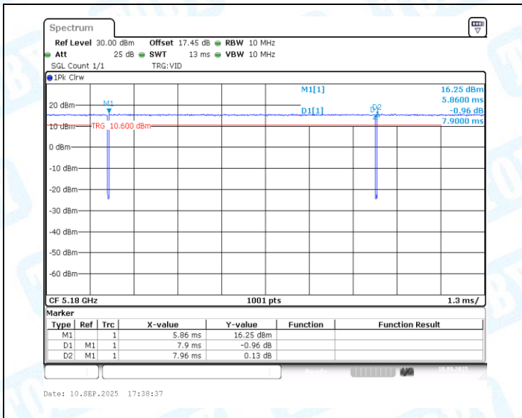
NTNV-11AC20MIMO-Ant1-5180
