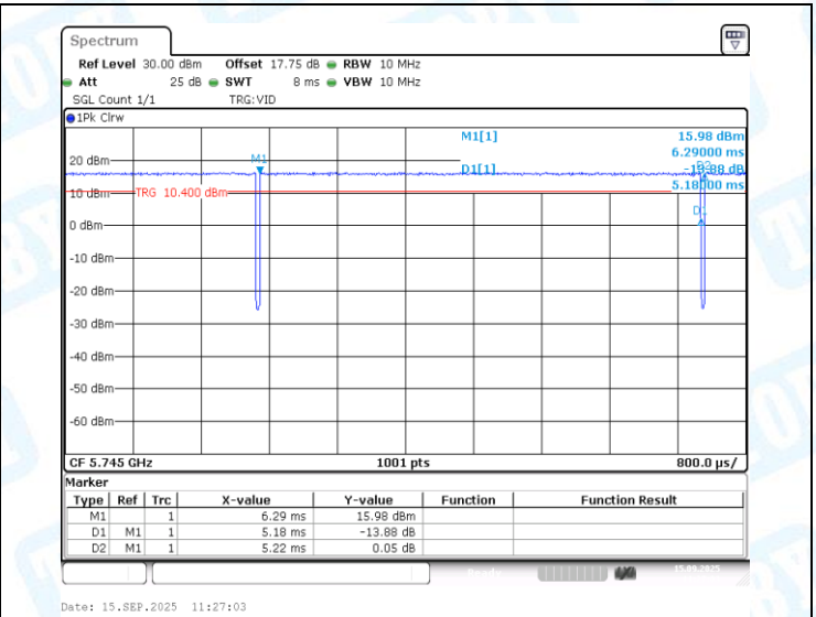
NTNV-11N20MIMO-Ant2-5745
