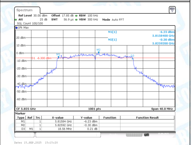
11AX20MIMO-Ant2-5825-PASS
