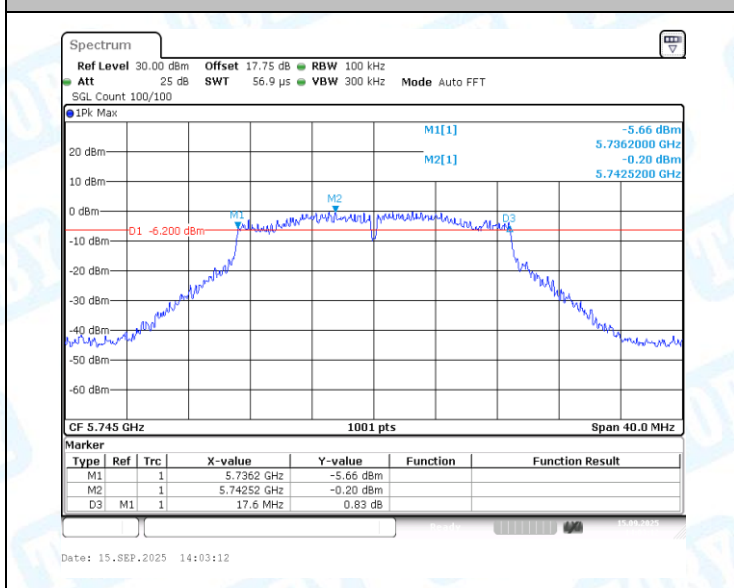
11AC20MIMO-Ant1-5745-PASS
