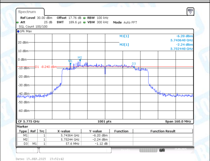
11AX80MIMO-Ant2-5775-PASS
