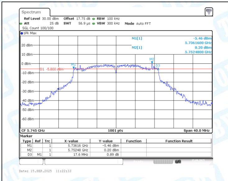
11N20MIMO-Ant1-5745-PASS
