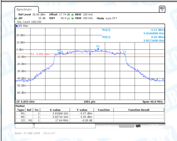
11AX20MIMO-Ant1-5825-PASS
