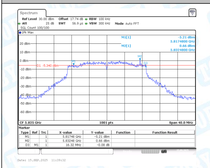
11N20MIMO-Ant1-5825-PASS
