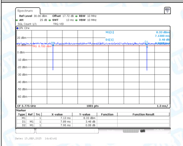
NTNV-11AC80MIMO-Ant1-5775
