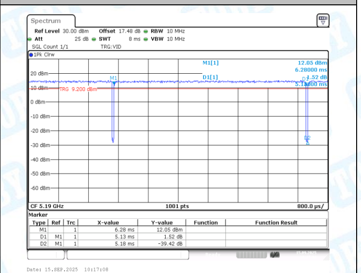
NTVN-11AX40MIMO-Ant2-5190
