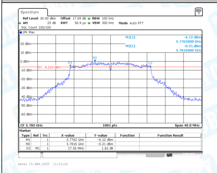
11N20MIMO-Ant1-5785-PASS
