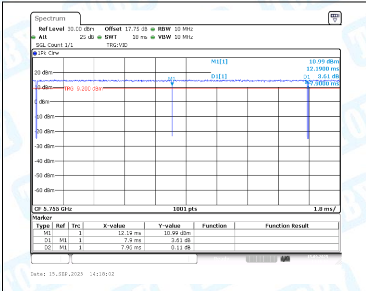
NTNV-11AC40MIMO-Ant1-5755
