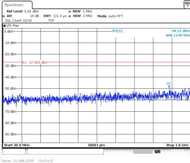
11AX80MIMO-Ant1-5210-30~1000-PASS
