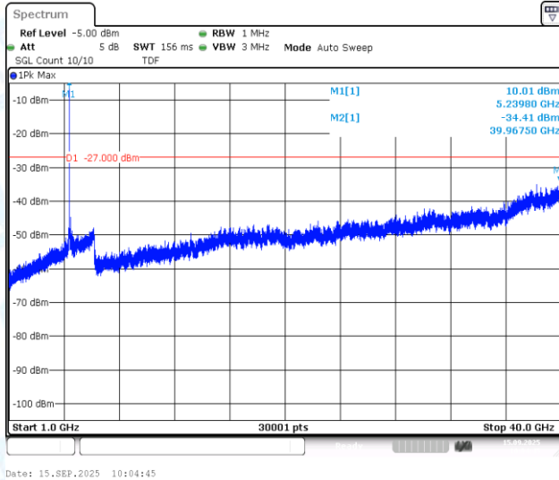
11AX20MIMO-Ant1-5240-1000~40000-PASS
