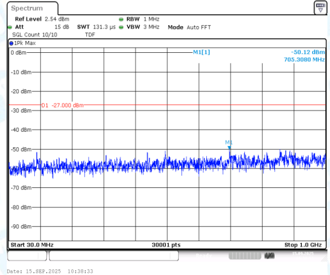
11AX80MIMO-Ant2-5210-30~1000-PASS
