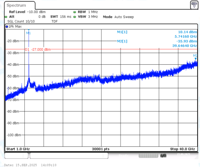
11AC20MIMO-Ant2-5745-1000~40000-PASS
