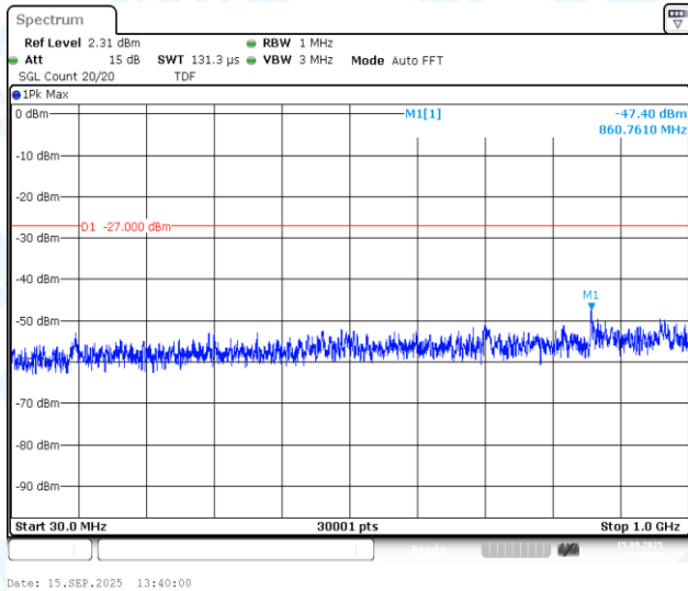
11AC20MIMO-Ant1-5785-30~1000-PASS
