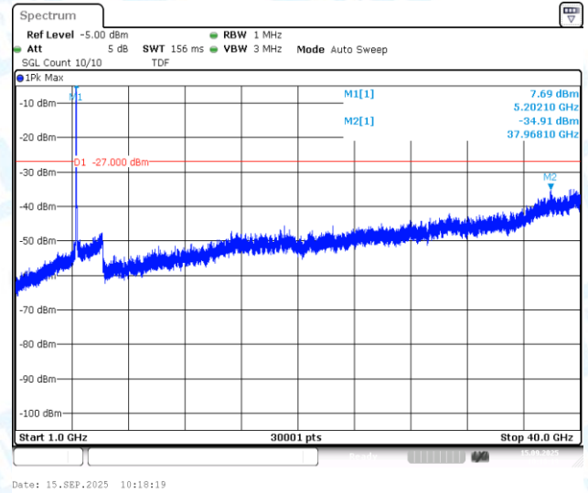
11AX40MIMO-Ant2-5190-1000~40000-PASS
