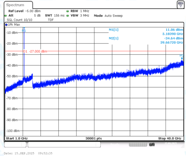
11AX20MIMO-Ant2-5180-1000~40000-PASS
