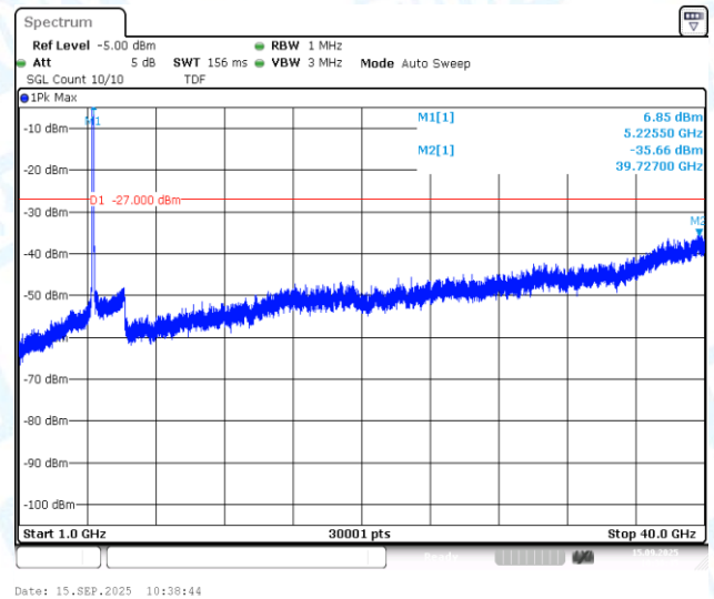
11AX80MIMO-Ant2-5210-1000~40000-PASS
