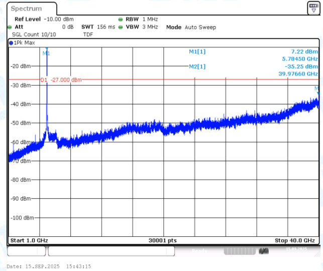
11AX40MIMO-Ant2-5795-1000~40000-PASS
