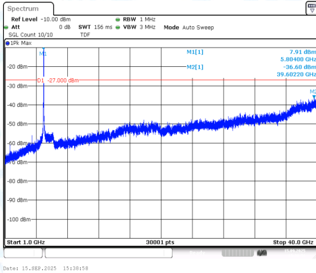
11AX40MIMO-Ant1-5795-1000~40000-PASS
