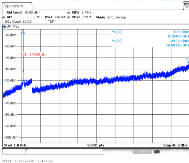
11AX80MIMO-Ant1-5210-1000~40000-PASS
