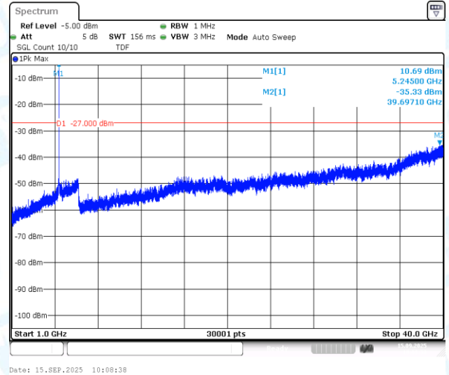
11AX20MIMO-Ant2-5240-1000~40000-PASS
