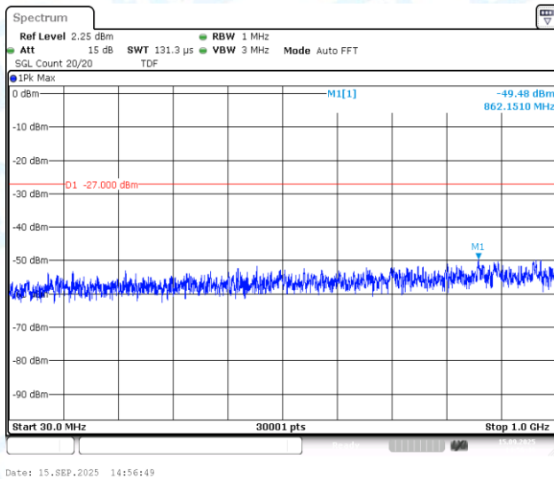
11AX20MIMO-Ant1-5745-30~1000-PASS
