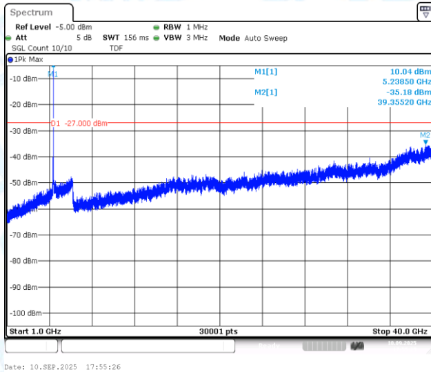
11AC20MIMO-Ant1-5240-1000~40000-PASS
