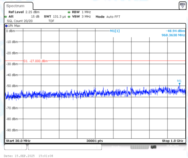
11AX20MIMO-Ant2-5745-30~1000-PASS
