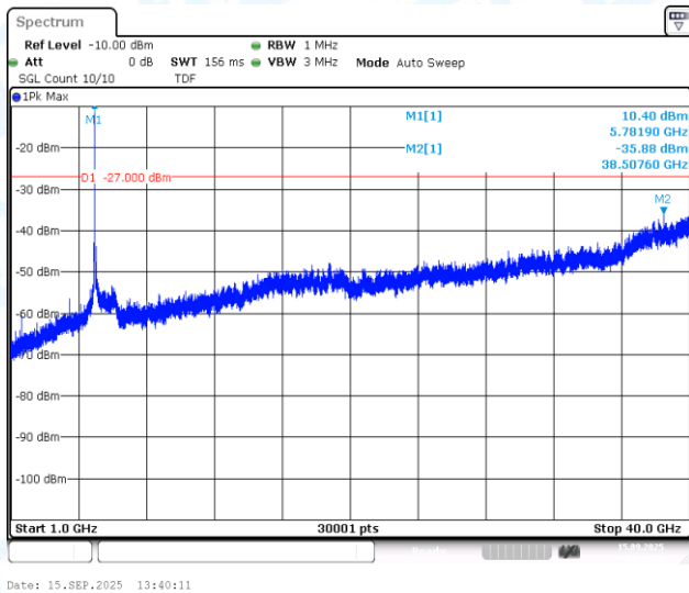
11AC20MIMO-Ant1-5785-1000~40000-PASS
