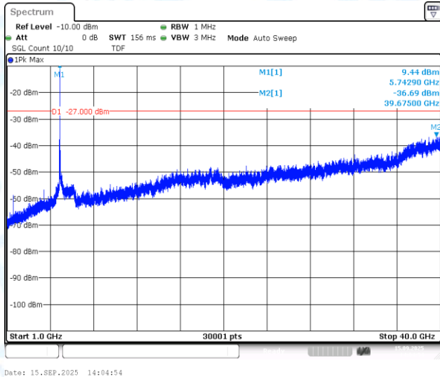
11AC20MIMO-Ant1-5745-1000~40000-PASS
