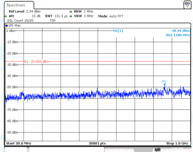
11N40MIMO-Ant2-5795-30~1000-PASS
