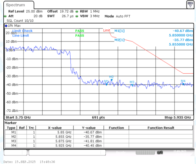
11AX80MIMO-Ant1-5775-PASS
