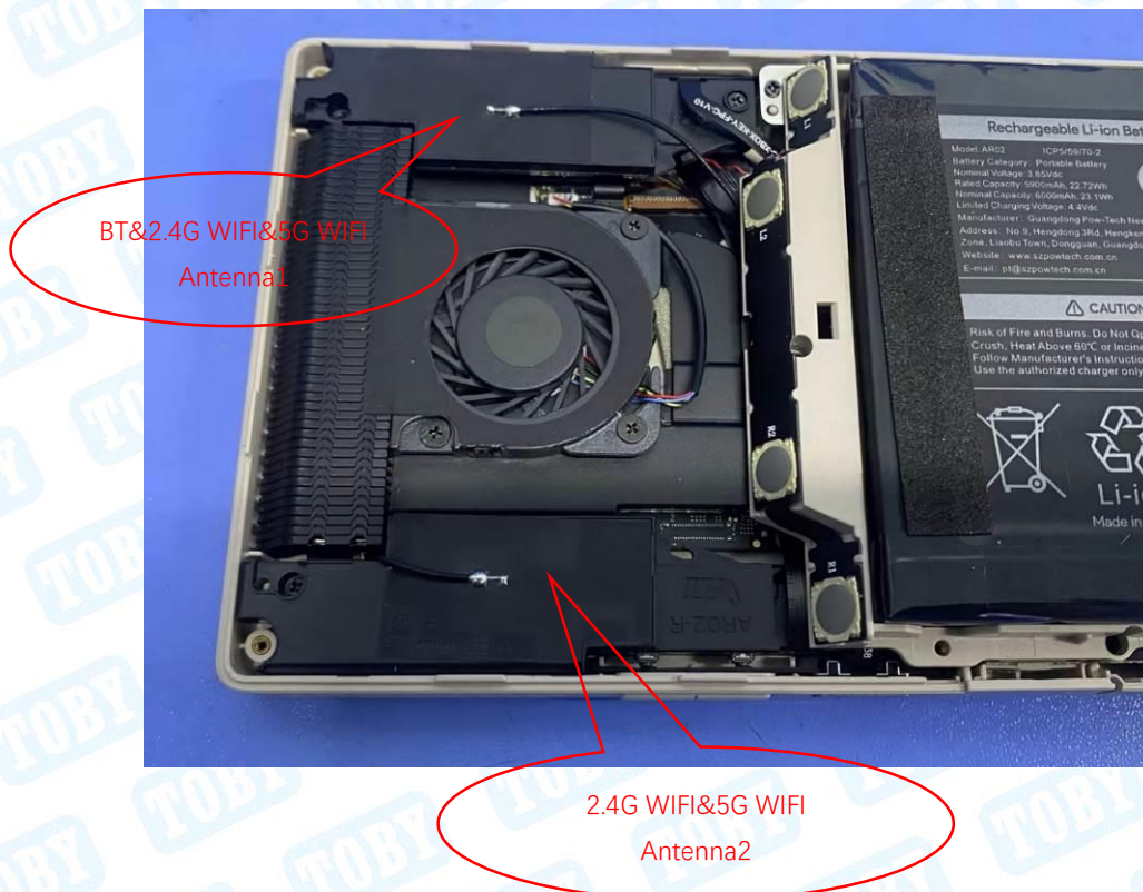
Photo 8 Internal of EUT
