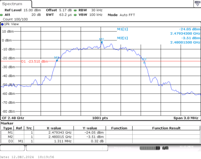
3DH5-Ant1-2480
