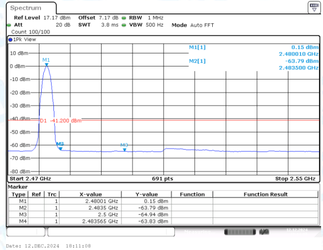
2DH5-Ant1-2480-PASS
