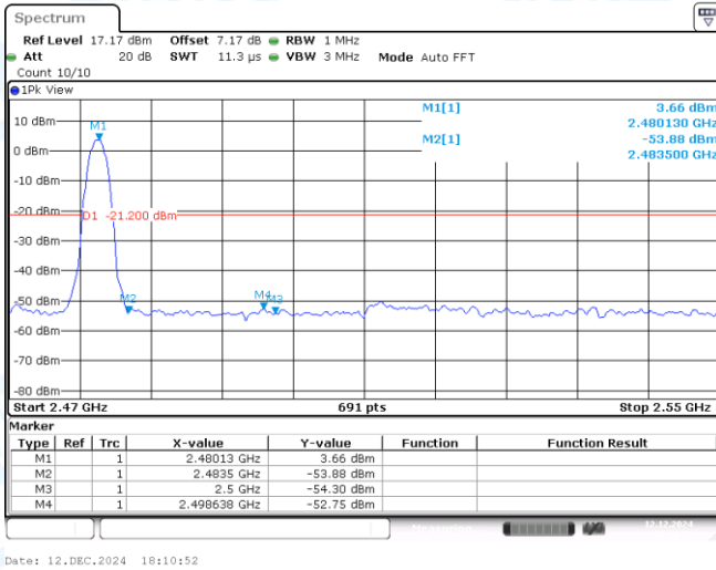
2DH5-Ant1-2480-PASS
