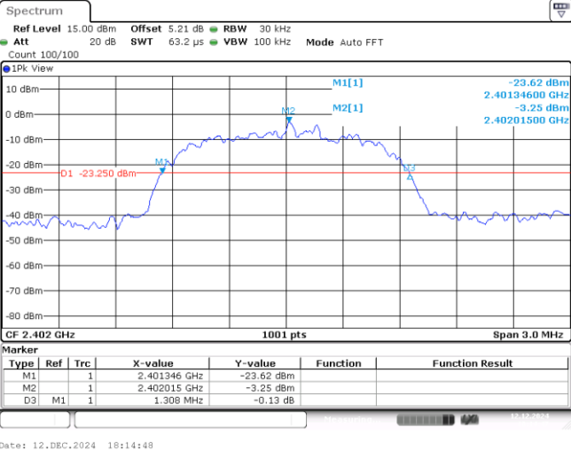
3DH5-Ant1-2402
