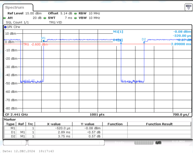
NTNV-3DH5-Ant1-2441
