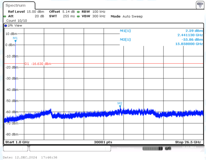
DH5-Ant1-2441-1000~26500-PASS
