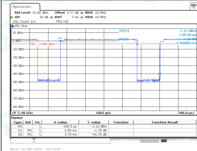
NTNV-3DH5-Ant1-2480
