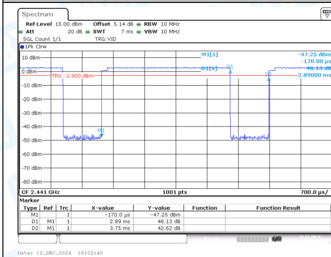
NTVN-2DH5-Ant1-2441
