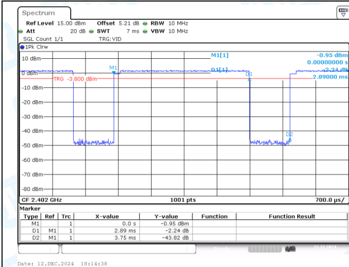
NTNV-3DH5-Ant1-2402
