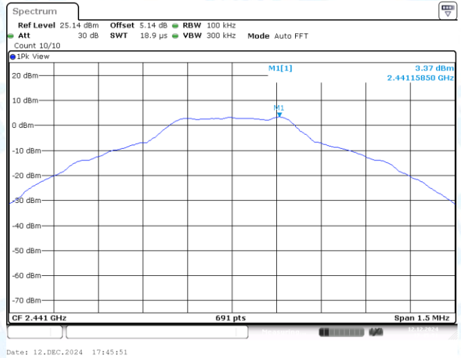
DH5-Ant1-2441-0~Reference-PASS
