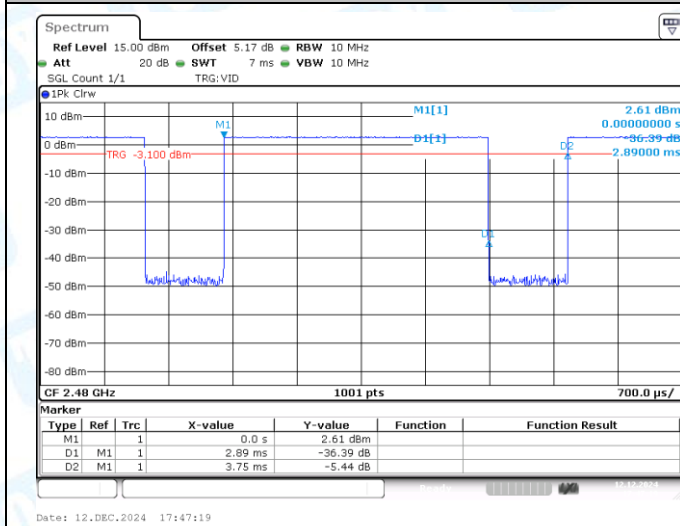
NTVN-DH5-Ant1-2480
