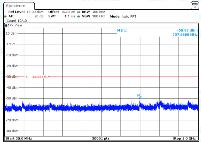
11AX20MIMO-Ant2-2462-0~Reference-PASS
