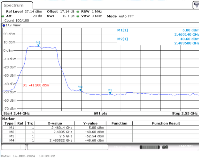
11G-CDD-Ant1-2462-PASS
