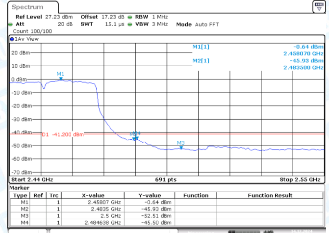
11N40MIMO-Ant2-2452-PASS
