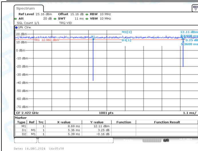
NTNV-11N40MIMO-Ant1-2422
