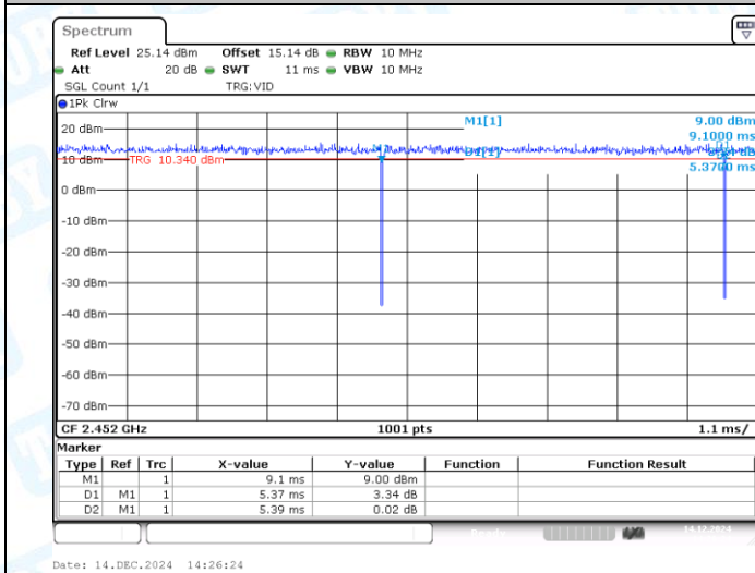
NTNV-11N40MIMO-Ant1-2452
