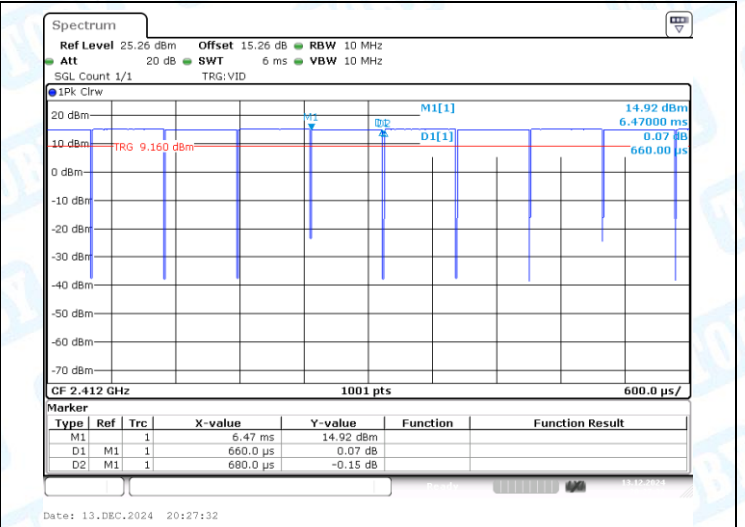
NTNV-11B-CDD-Ant2-2412
