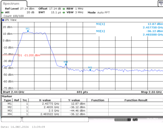
11G-CDD-Ant1-2462-PASS
