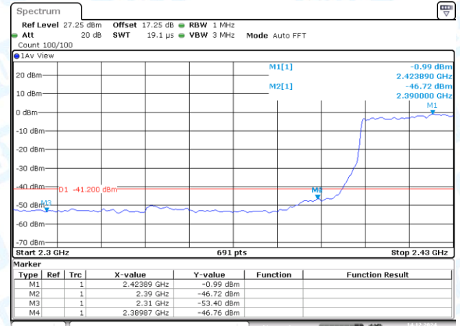
11AX40MIMO-Ant2-2422-PASS
