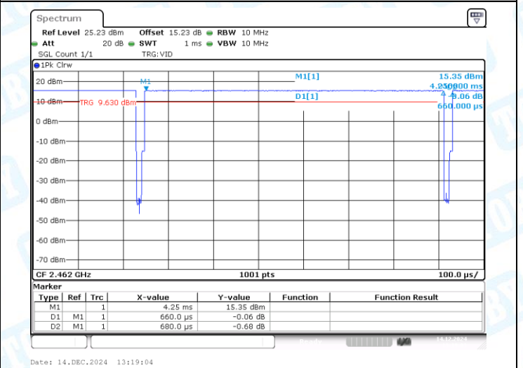
NTNV-11B-CDD-Ant2-2462
