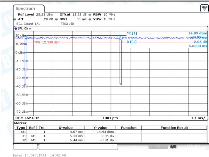
NTNV-11N20MIMO-Ant2-2462
