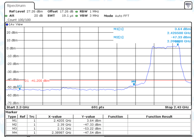
11AX20MIMO-Ant2-2412-PASS
