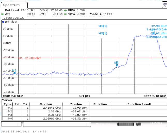
11N20MIMO-Ant1-2412-PASS
