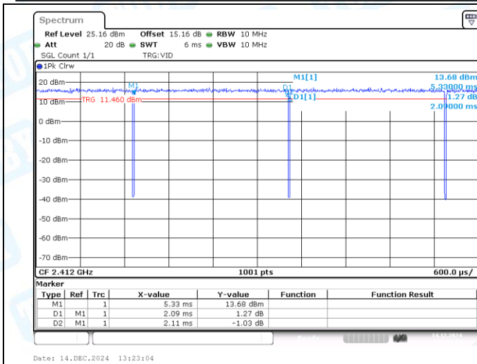
NTNV-11G-CDD-Ant1-2412
