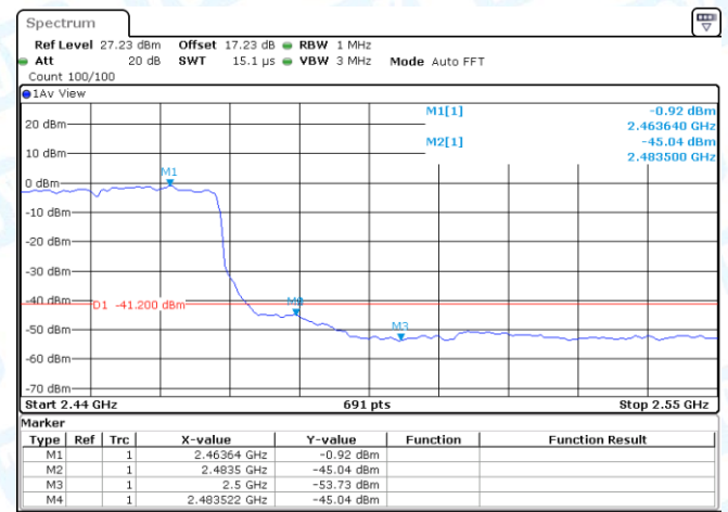
11AX40MIMO-Ant2-2452-PASS
