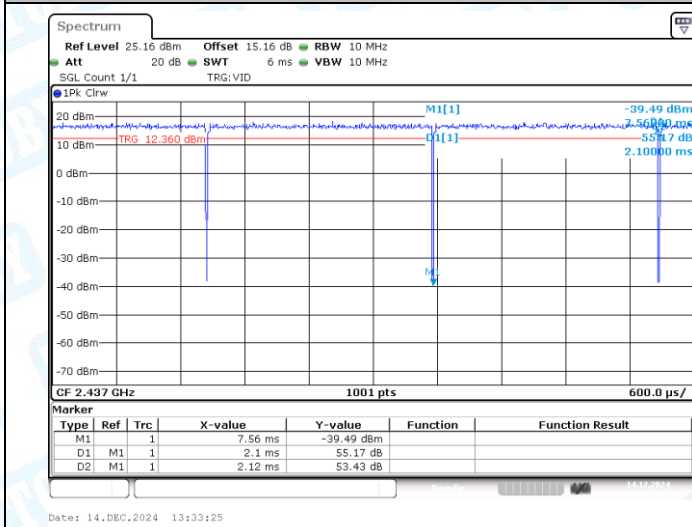
NTNV-11G-CDD-Ant1-2437
