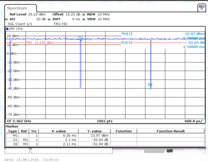
NTNV-11G-CDD-Ant2-2462
