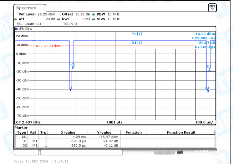
NTNV-11B-CDD-Ant2-2437
