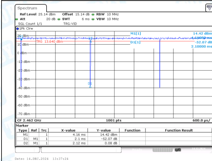
NTNV-11G-CDD-Ant1-2462
