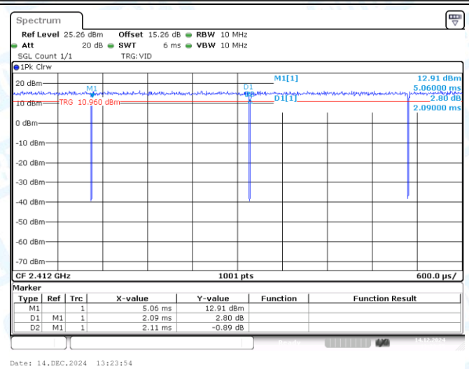
NTNV-11G-CDD-Ant2-2412
