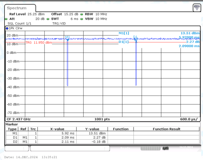
NTNV-11G-CDD-Ant2-2437
