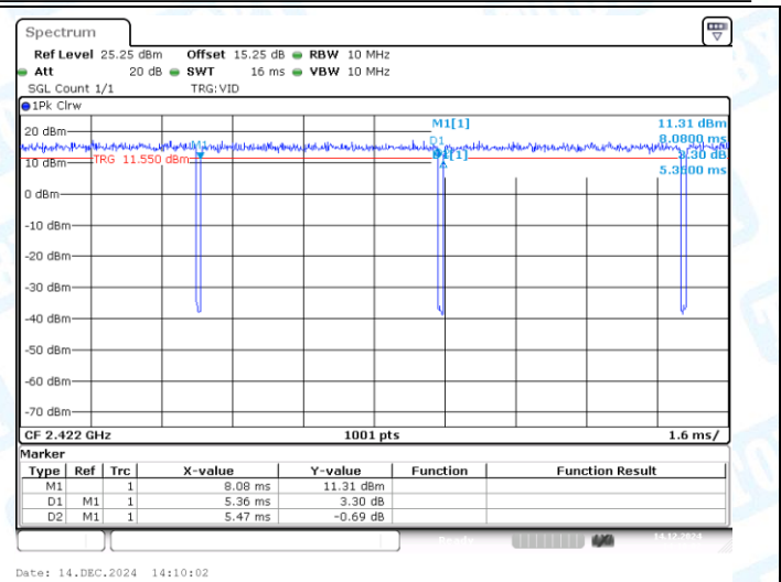
NTNV-11N40MIMO-Ant2-2422
