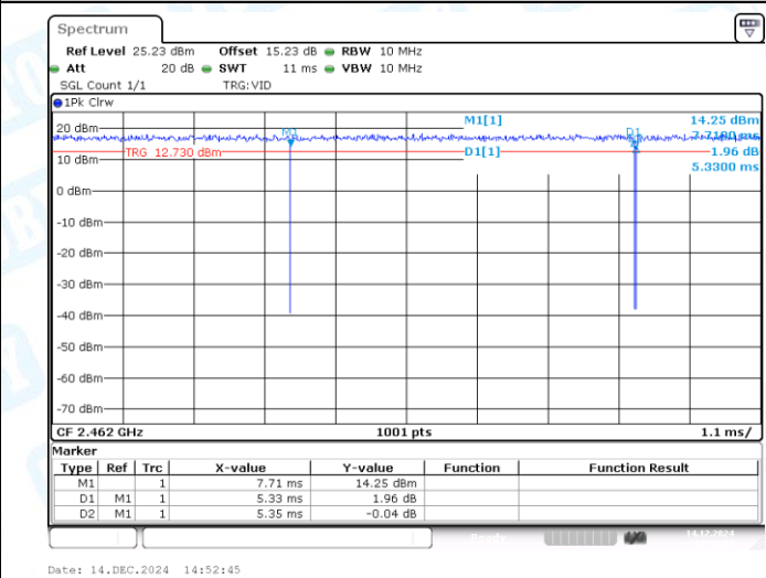
NTNV-11AX20MIMO-Ant2-2462
