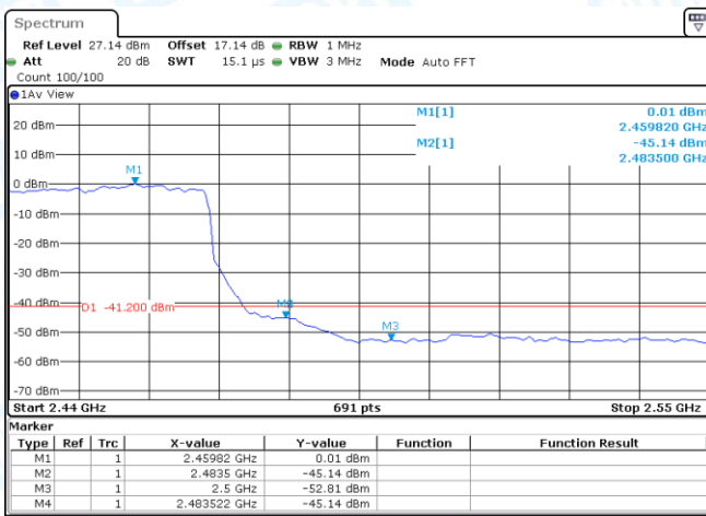
11AX40MIMO-Ant1-2452-PASS
