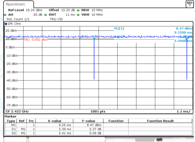
NTNV-11AX40MIMO-Ant2-2422
