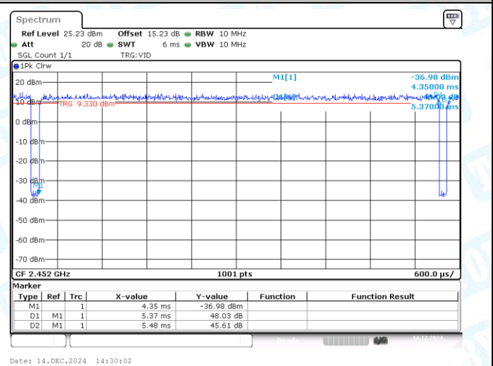
NTNV-11N40MIMO-Ant2-2452
