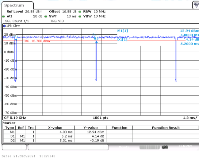
NTNV-11AC40MIMO-Ant1-5190
