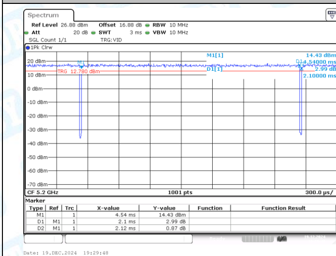
NTNV-11A-CDD-Ant1-5200
