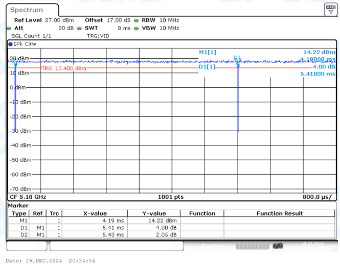
NTNV-11AC20MIMO-Ant2-5180
