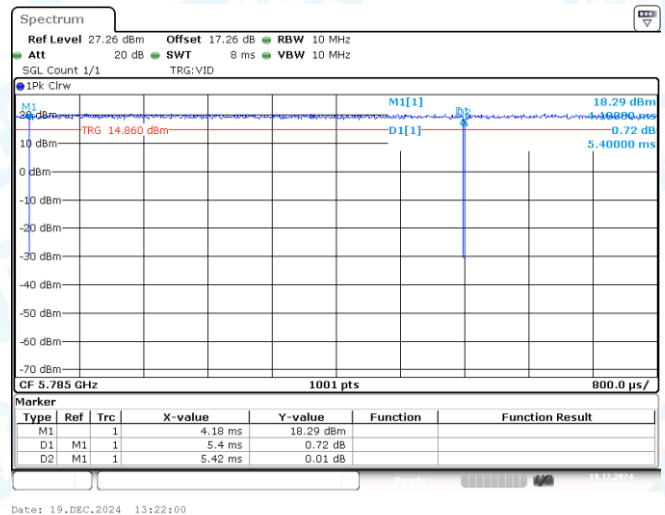
NTNV-11AC20MIMO-Ant2-5785
