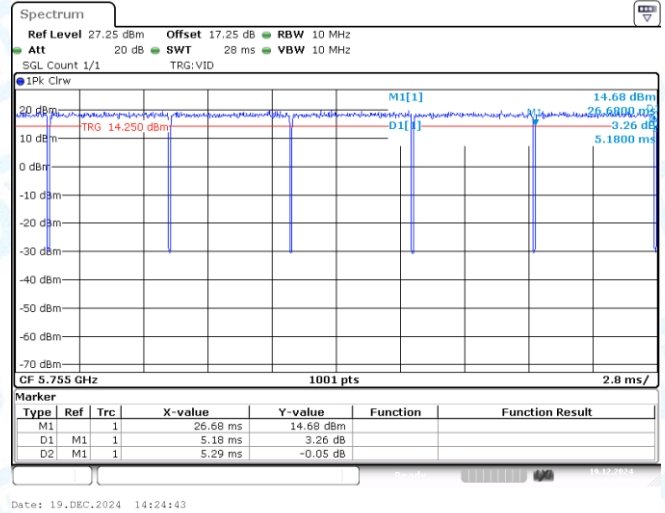
NTNV-11AC40MIMO-Ant2-5755
