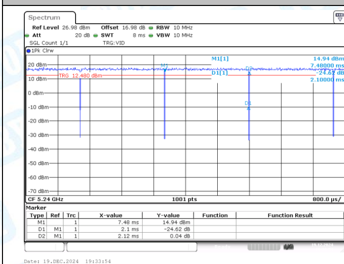
NTNV-11A-CDD-Ant1-5240
