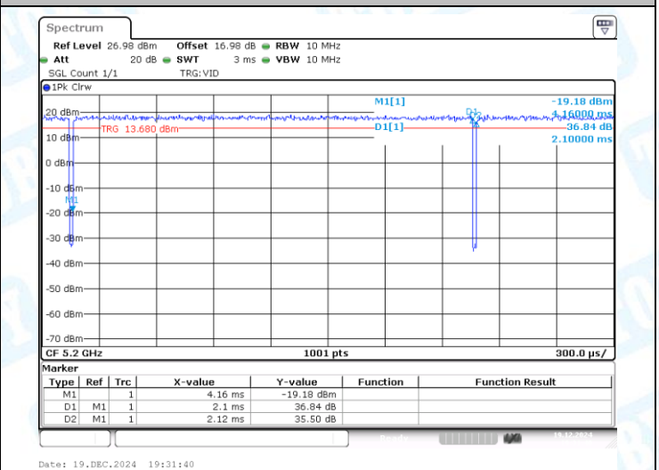
NTNV-11A-CDD-Ant2-5200
