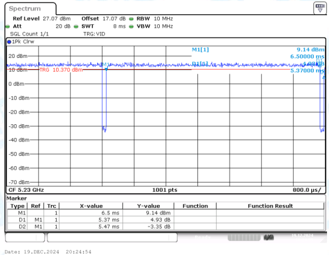
NTNV-11N40MIMO-Ant2-5230
