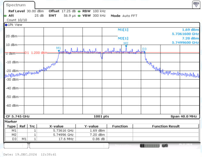
11N20MIMO-Ant2-5745-PASS
