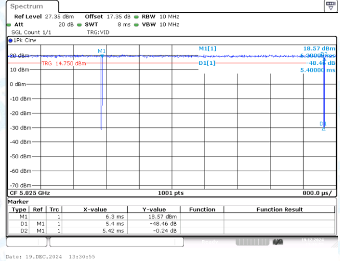
NTNV-11AC20MIMO-Ant2-5825
