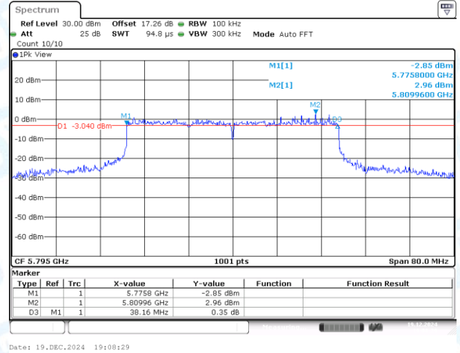
11AX40MIMO-Ant2-5795-PASS
