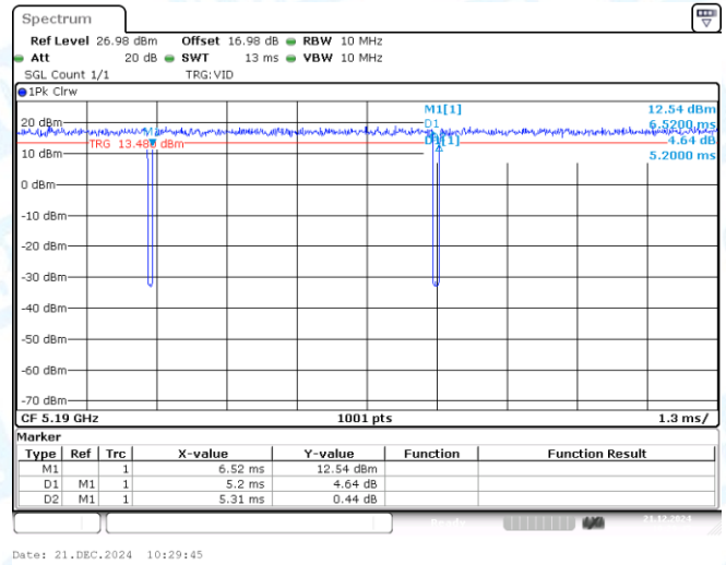
NTNV-11AC40MIMO-Ant2-5190
