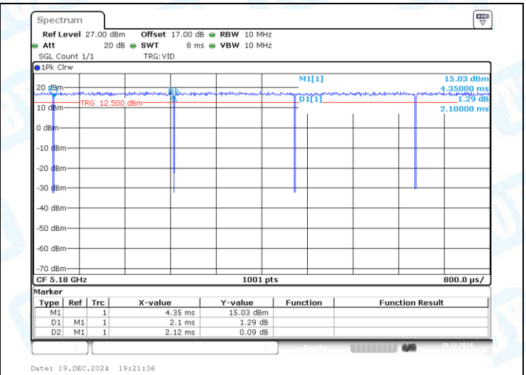
NTNV-11A-CDD-Ant2-5180
