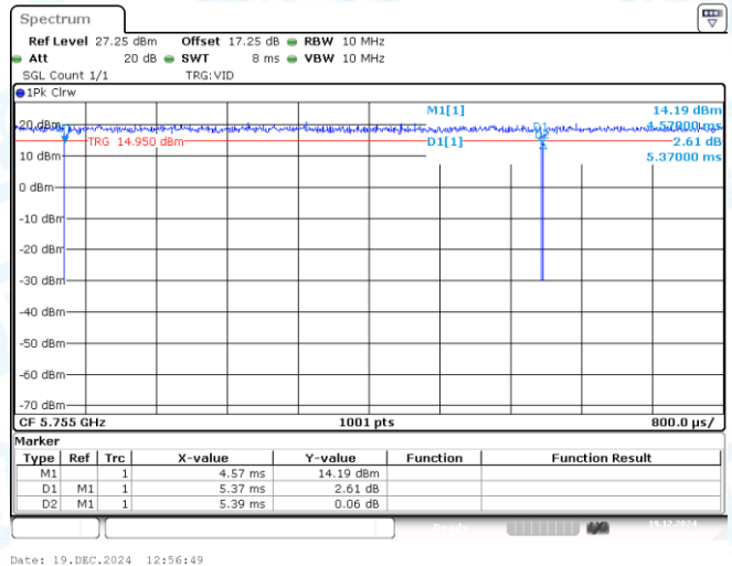
NTNV-11N40MIMO-Ant2-5755
