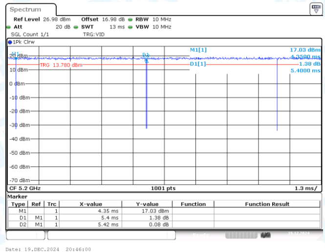
NTNV-11AC20MIMO-Ant2-5200
