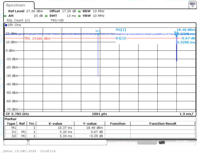
NTNV-11N20MIMO-Ant2-5785
