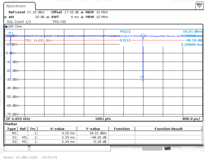
NTNV-11N20MIMO-Ant2-5825
