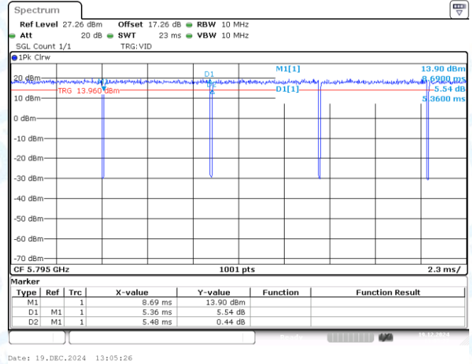
NTNV-11N40MIMO-Ant2-5795
