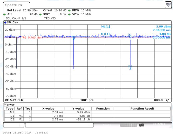
NTNV-11AC80MIMO-Ant2-5210
