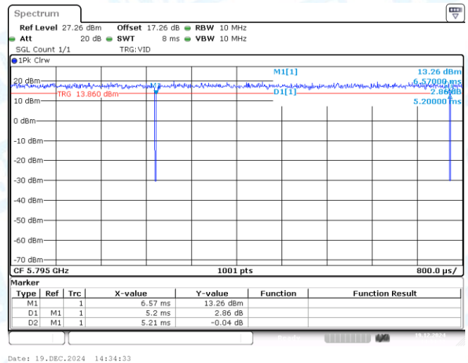
NTNV-11AC40MIMO-Ant2-5795
