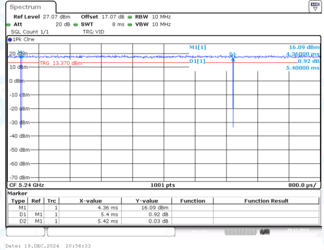
NTNV-11AC20MIMO-Ant2-5240
