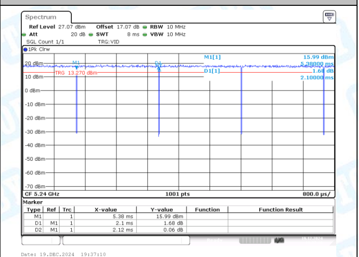
NTNV-11A-CDD-Ant2-5240
