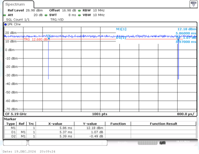
NTNV-11N40MIMO-Ant2-5190
