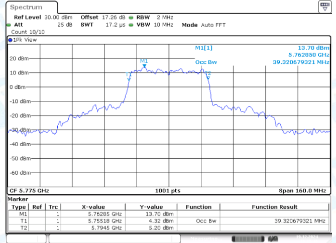
11AX80MIMO-Ant2-5775
