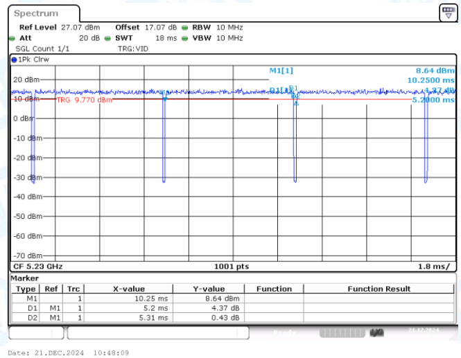
NTNV-11AC40MIMO-Ant2-5230
