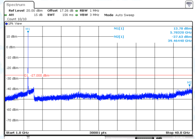
11A-CDD-Ant2-5785-1000~40000-PASS
