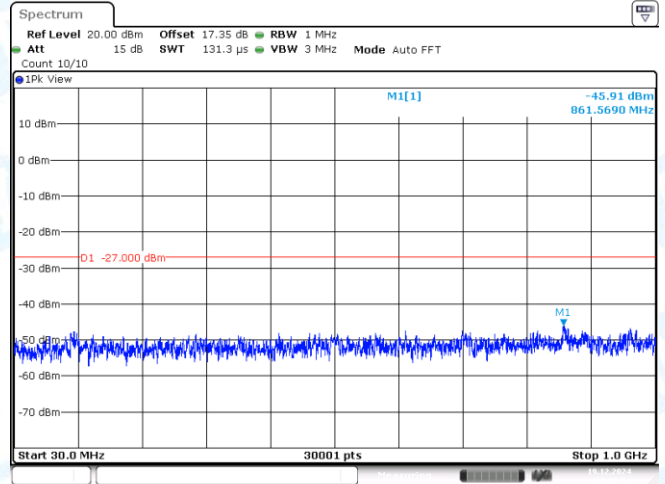
11AC20MIMO-Ant2-5825-30~1000-PASS
