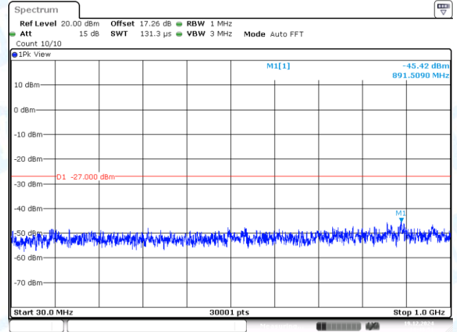
11AC80MIMO-Ant2-5775-30~1000-PASS
