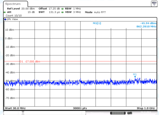
11AX40MIMO-Ant2-5755-30~1000-PASS
