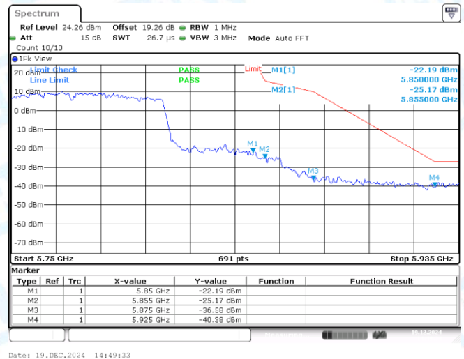
11AC80MIMO-Ant2-5775-PASS
