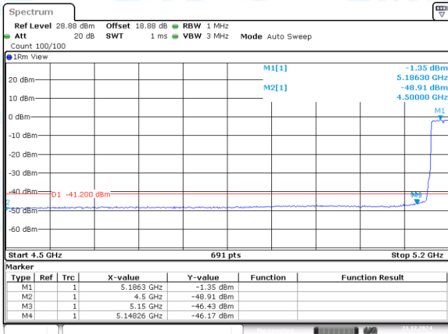
11AX40MIMO-Ant1-5190-PASS
