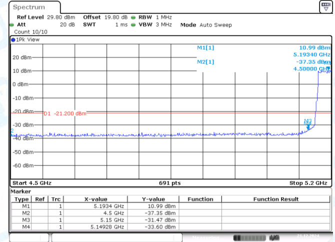
11AX40MIMO-Ant2-5190-PASS
