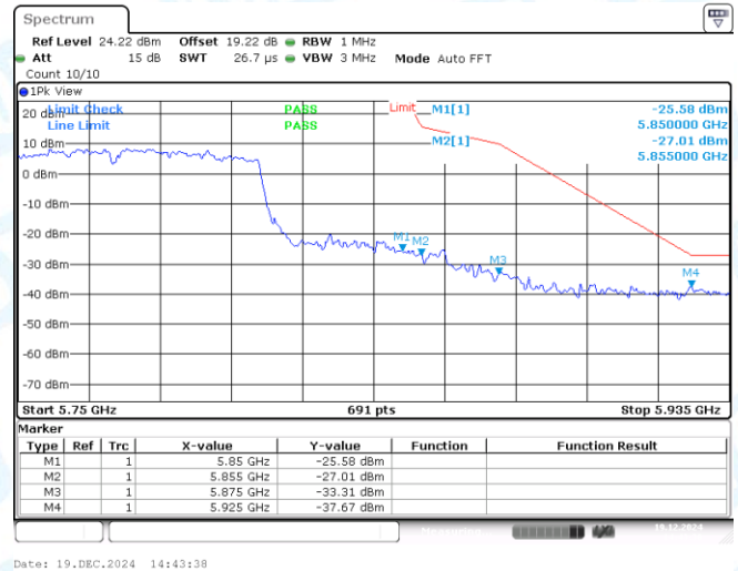
11AC80MIMO-Ant1-5775-PASS
