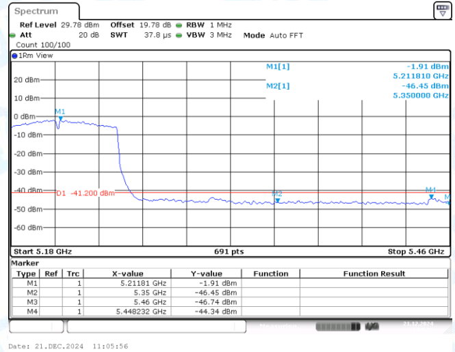
11AC80MIMO-Ant2-5210-PASS
