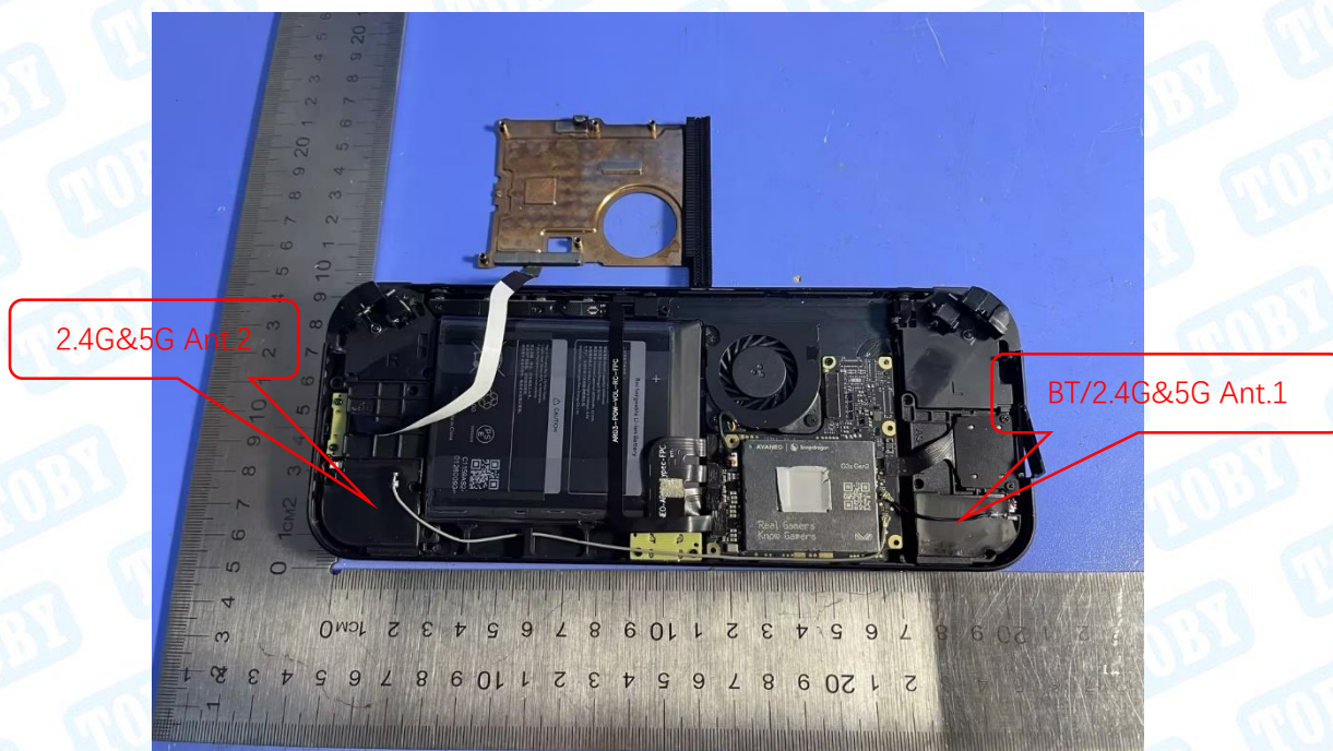
Photo 8 Internal of EUT
