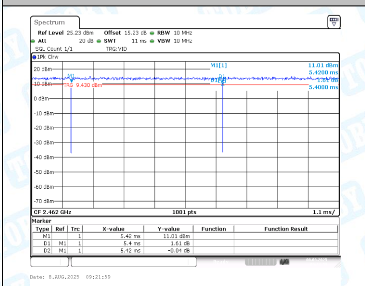
NTVN-11AX20MIMO-Ant2-2462
