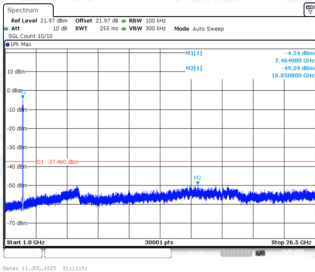
11AX40MIMO-Ant1-2452-1000~26500-PASS
