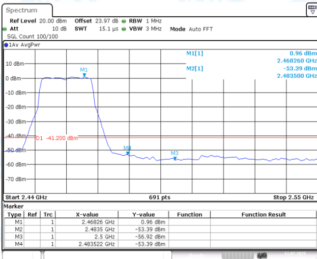
11N20MIMO-Ant1-2462-PASS
