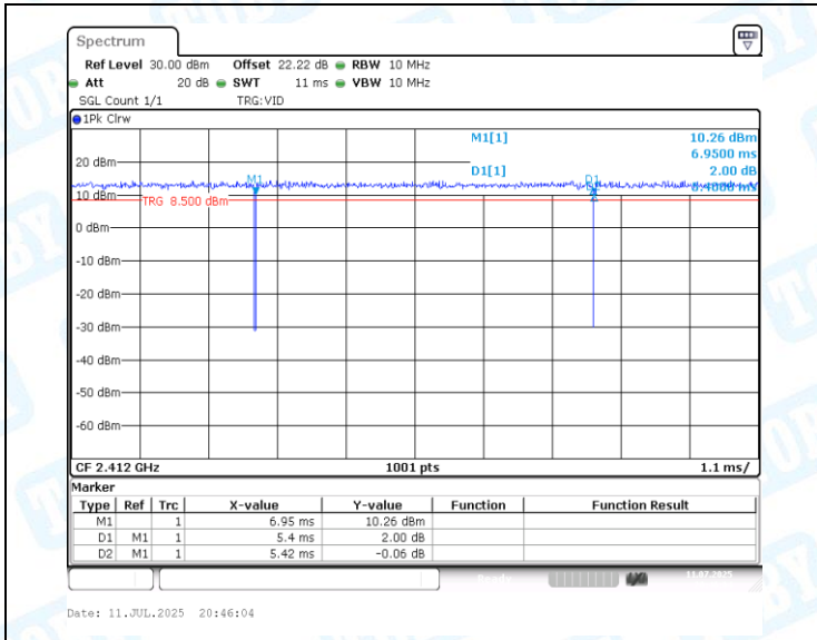
NTVN-11AX20MIMO-Ant2-2412
