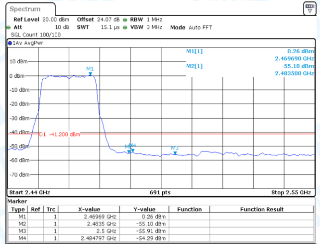
11AX20MIMO-Ant2-2462-PASS
