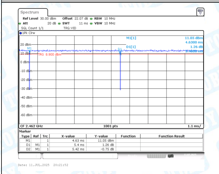
NTNV-11N20MIMO-Ant2-2462
