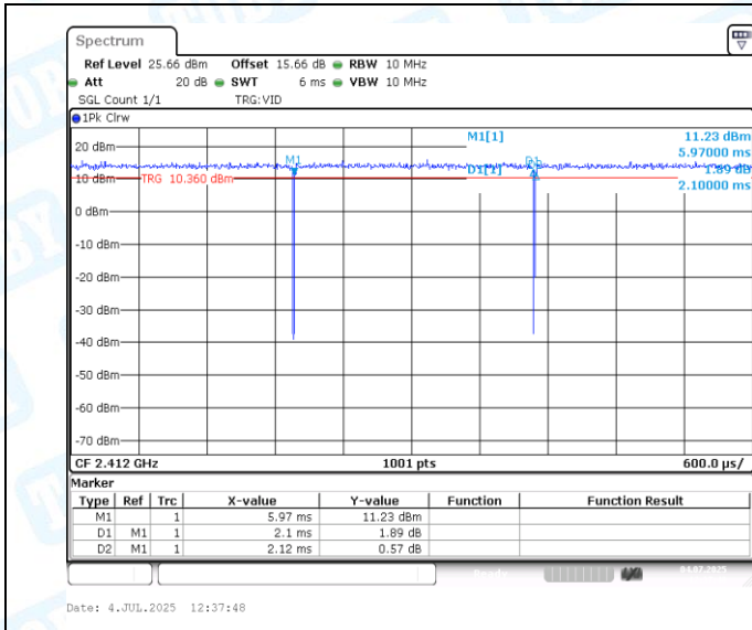
NTNV-11G-CDD-Ant1-2412
