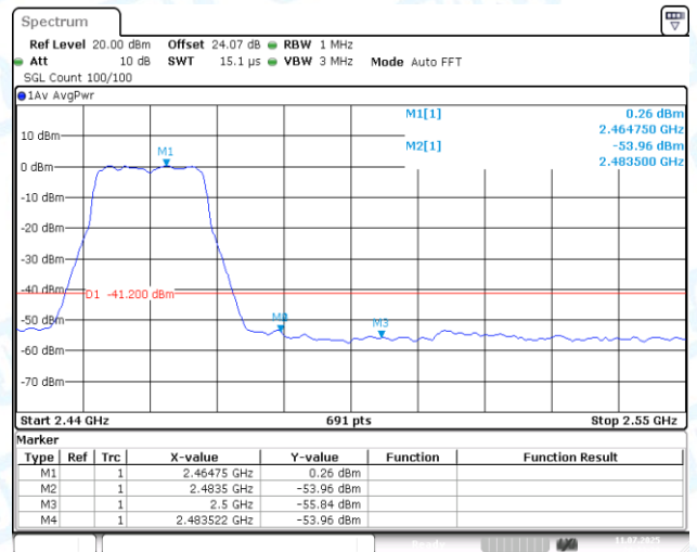
11N20MIMO-Ant2-2462-PASS
