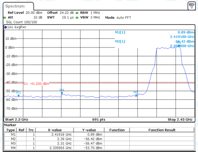
11G-CDD-Ant2-2412-PASS
