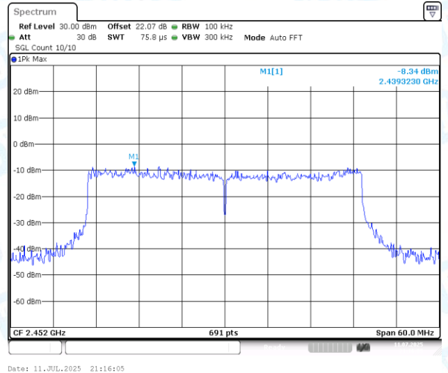
11AX40MIMO-Ant2-2452-0~Reference-PASS
