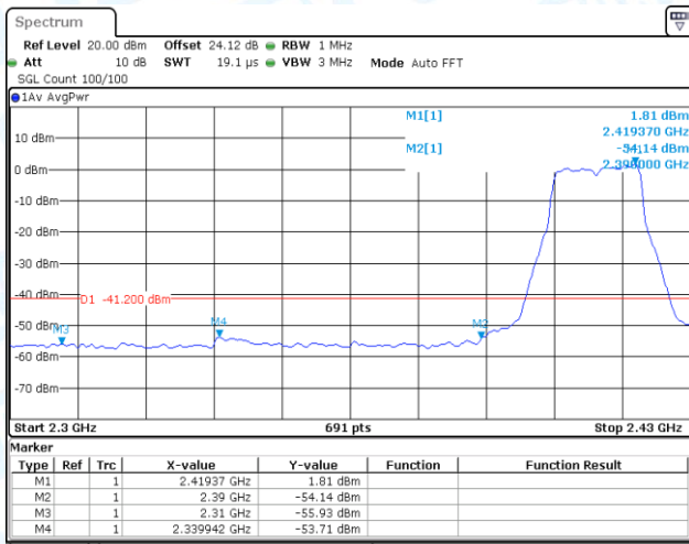
11G-CDD-Ant1-2412-PASS
