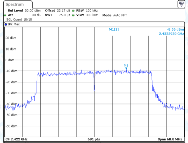
11AX40MIMO-Ant2-2422-0~Reference-PASS
