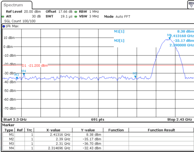
11B-CDD-Ant1-2412-PASS
