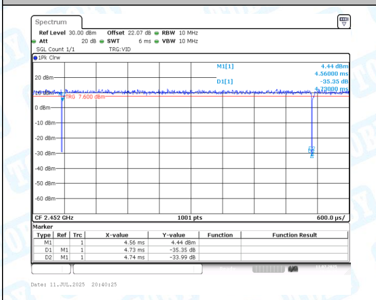
NTNV-11N40MIMO-Ant2-2452
