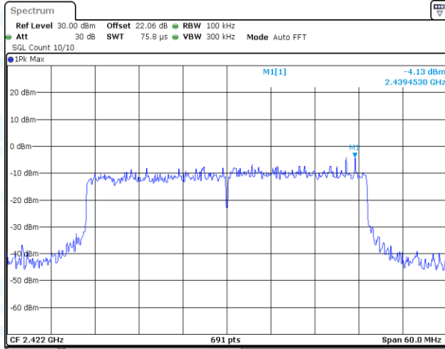
11AX40MIMO-Ant1-2422-0~Reference-PASS
