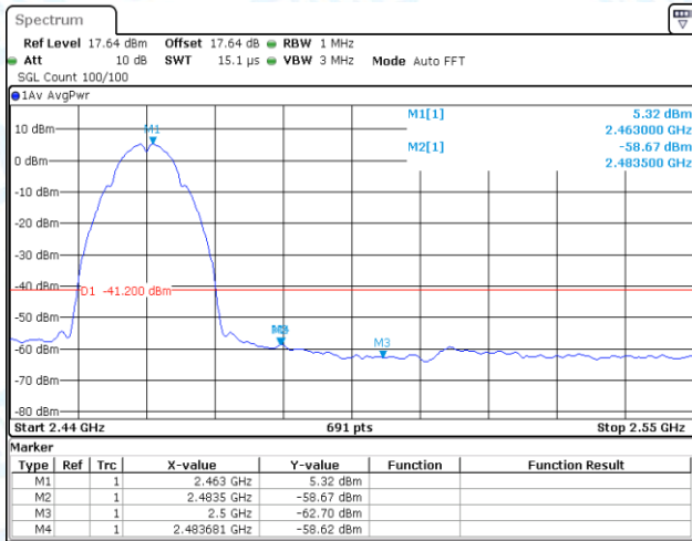
11B-CDD-Ant1-2462-PASS
