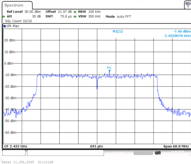
11AX40MIMO-Ant1-2452-0~Reference-PASS
