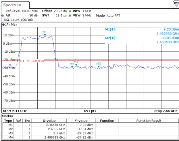
11AX20MIMO-Ant1-2462-PASS
