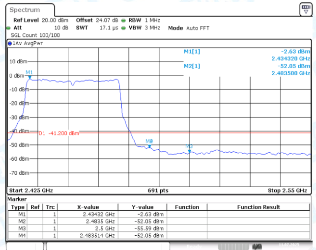
11AX40MIMO-Ant2-2452-PASS
