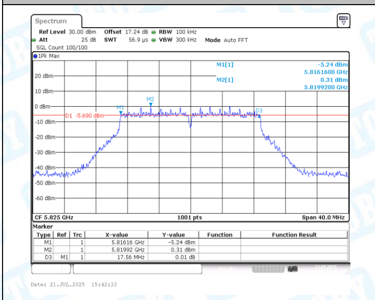
11AC20MIMO-Ant1-5825-PASS
