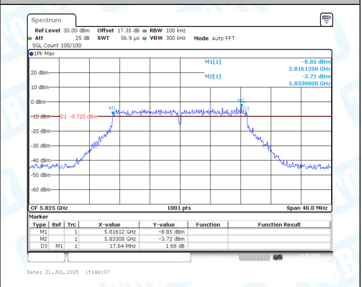
11AC20MIMO-Ant2-5825-PASS
