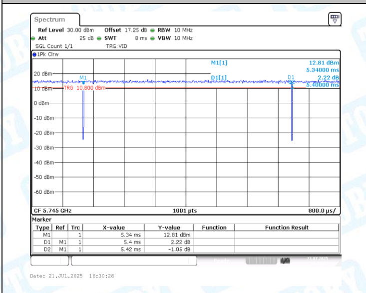
NTVN-11AX20MIMO-Ant1-5745
