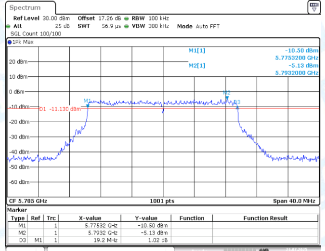
11AX20MIMO-Ant2-5785-PASS
