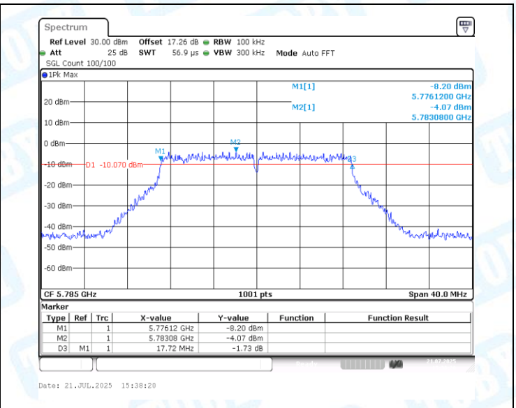
11AC20MIMO-Ant2-5785-PASS
