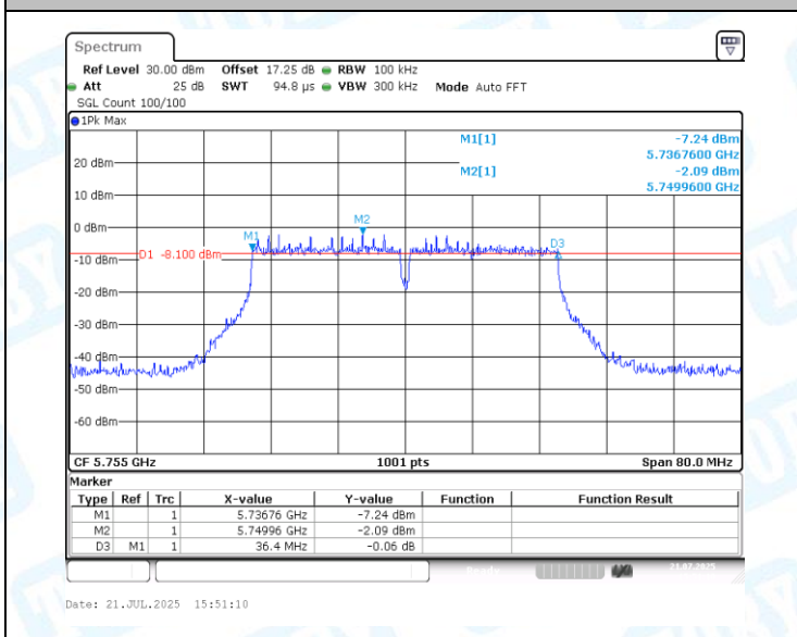
11AC40MIMO-Ant1-5755-PASS
