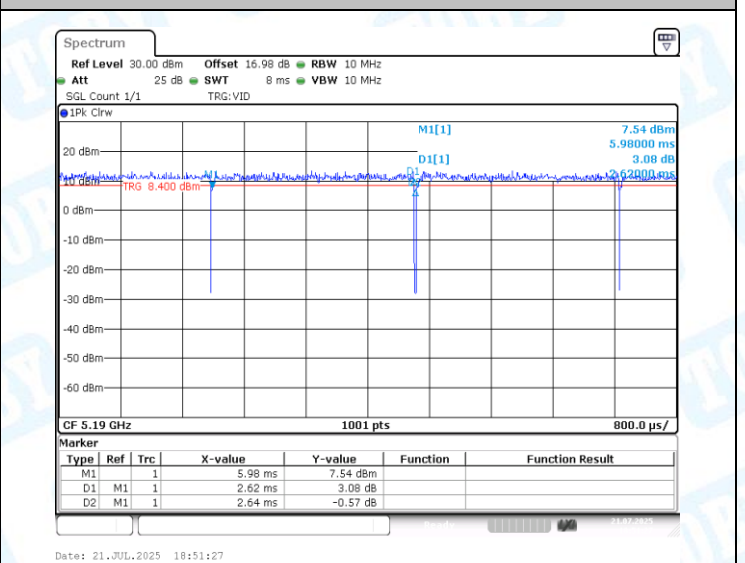
NTNV-11AC40MIMO-Ant2-5190
