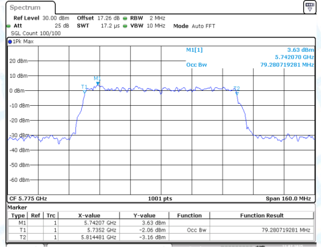
11AX80MIMO-Ant2-5775
