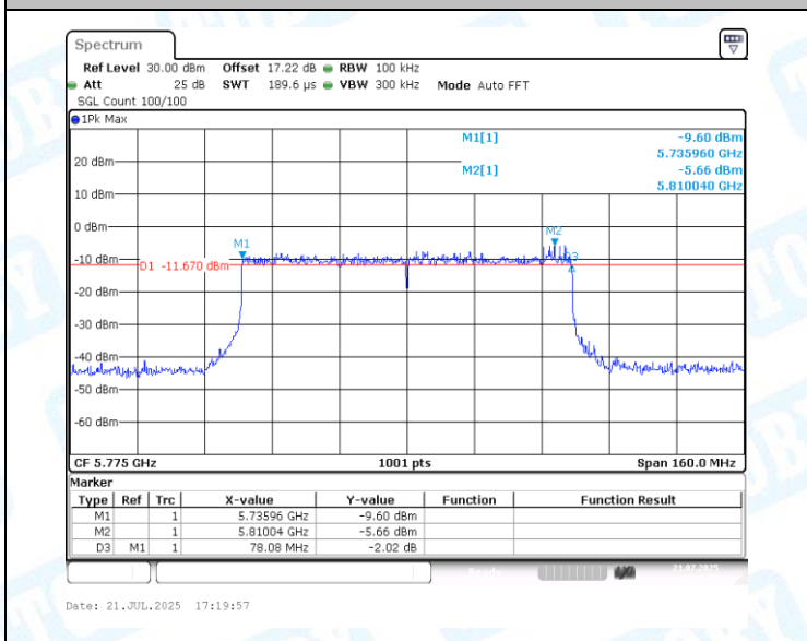
11AX80MIMO-Ant1-5775-PASS
