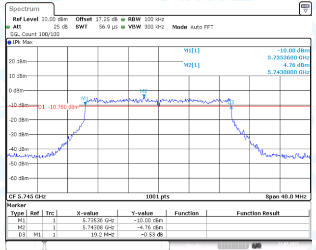
11AX20MIMO-Ant2-5745-PASS
