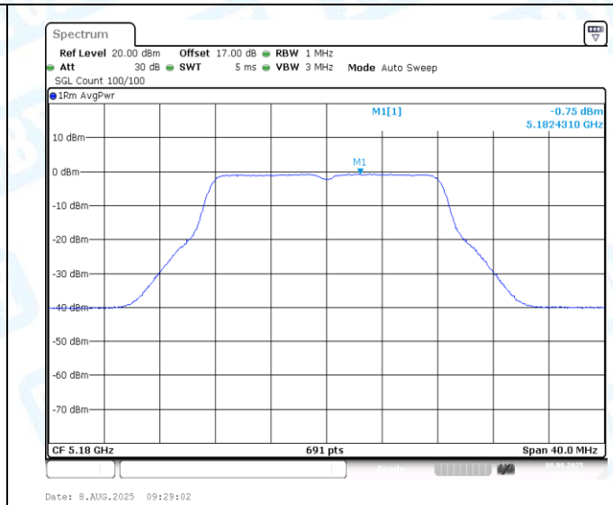
11A-CDD-Ant2-5180-PASS
