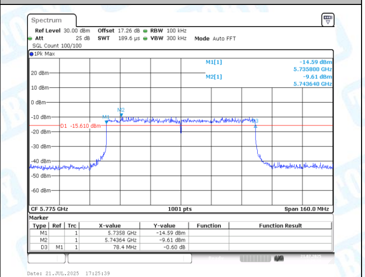
11AX80MIMO-Ant2-5775-PASS
