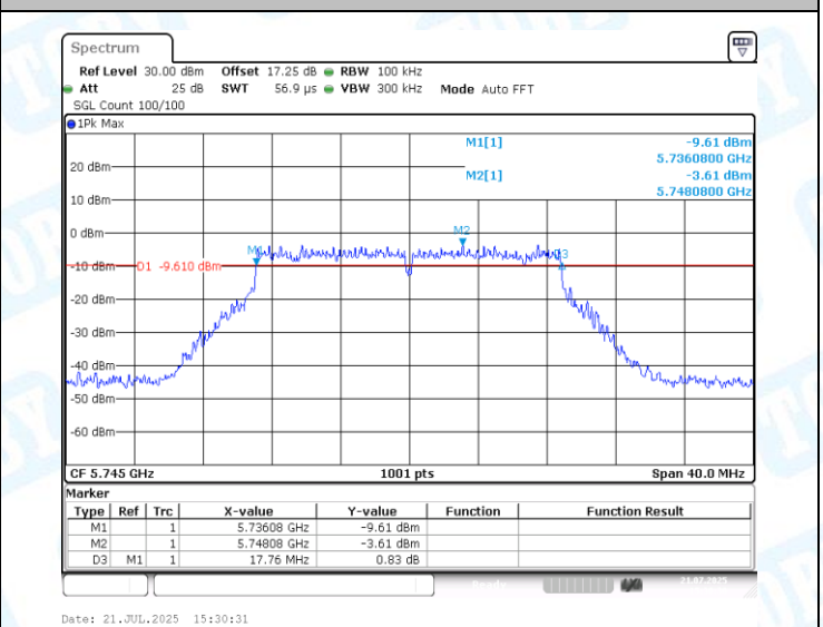
11AC20MIMO-Ant2-5745-PASS
