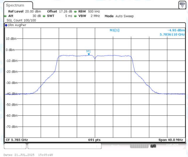
11A-CDD-Ant2-5785-PASS
