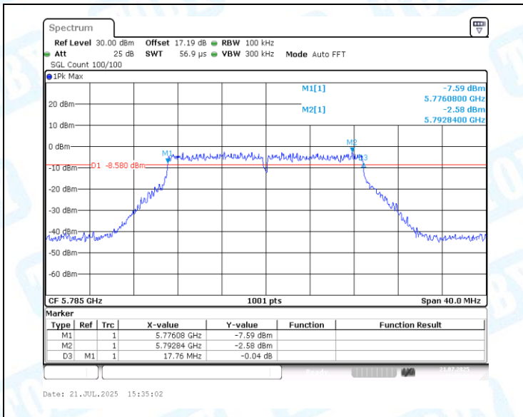
11AC20MIMO-Ant1-5785-PASS
