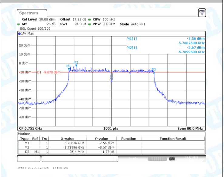
11AC40MIMO-Ant2-5755-PASS
