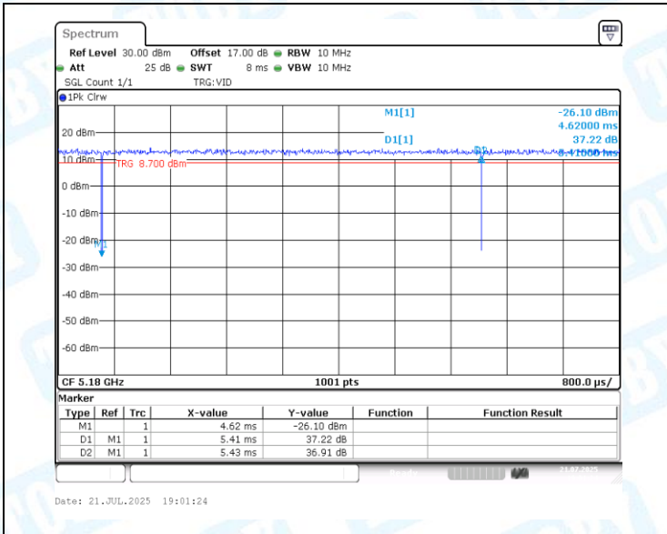
NTVN-11AX20MIMO-Ant2-5180
