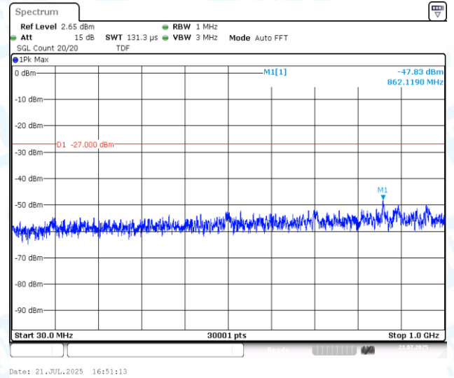
11AX20MIMO-Ant2-5825-30~1000-PASS
