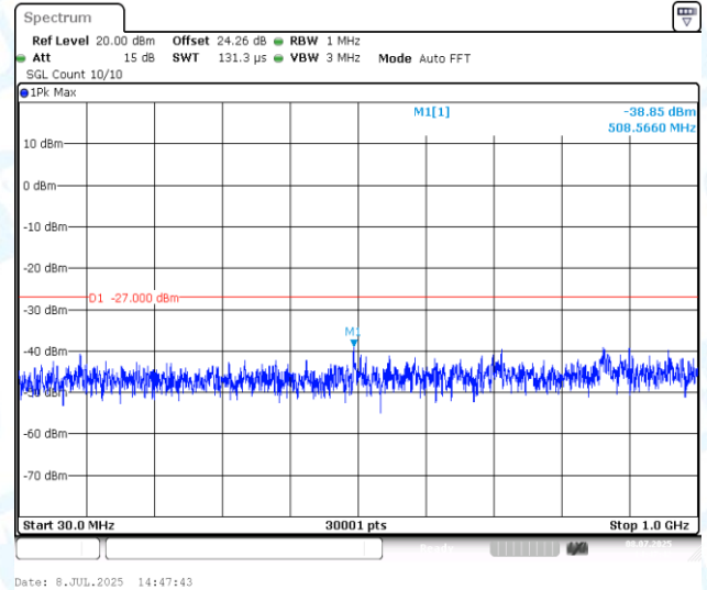
11AC40MIMO-Ant2-5230-30~1000-PASS
