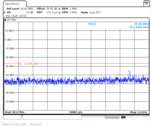
11AX20MIMO-Ant2-5200-30~1000-PASS
