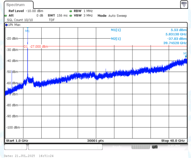
11AX20MIMO-Ant2-5825-1000~40000-PASS
