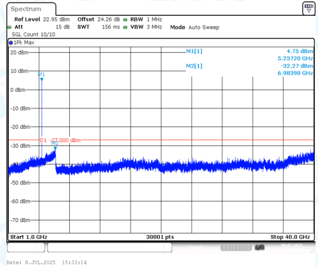
11AX20MIMO-Ant2-5240-1000~40000-PASS
