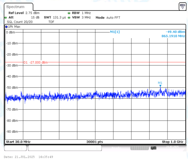
11AX20MIMO-Ant2-5745-30~1000-PASS
