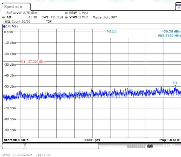
11AX20MIMO-Ant1-5745-30~1000-PASS
