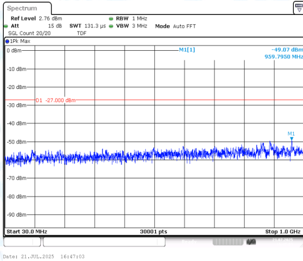
11AX20MIMO-Ant1-5825-30~1000-PASS
