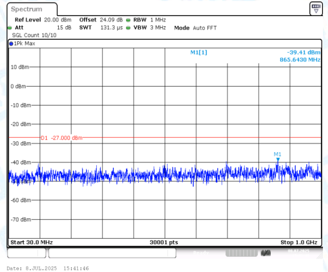
11AX40MIMO-Ant2-5190-30~1000-PASS
