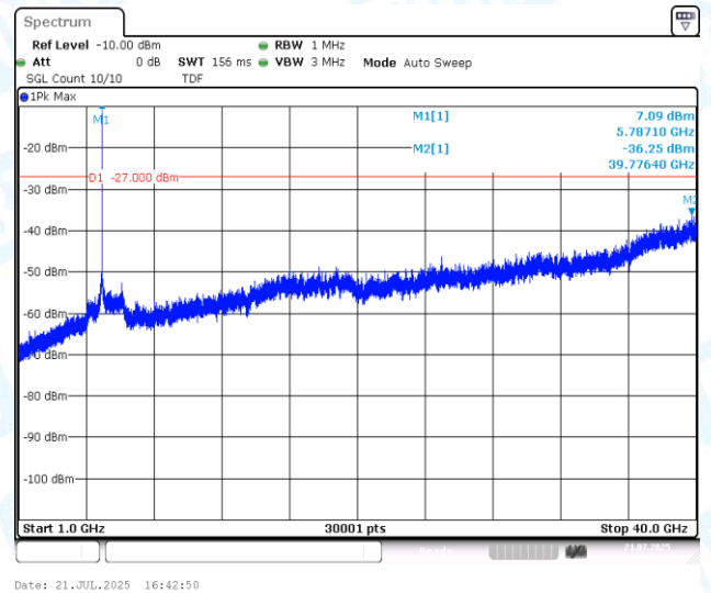
11AX20MIMO-Ant2-5785-1000~40000-PASS
