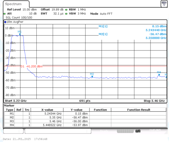
11N20MIMO-Ant2-5240-PASS
