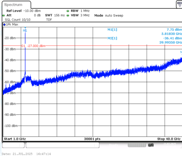
11AX20MIMO-Ant1-5825-1000~40000-PASS
