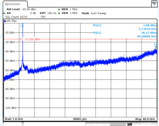
11AX80MIMO-Ant2-5775-1000~40000-PASS
