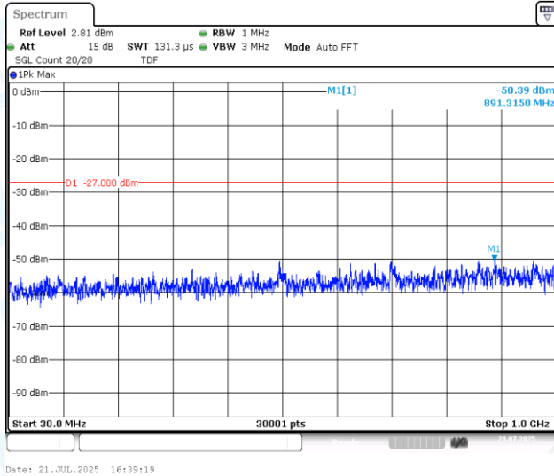
11AX20MIMO-Ant1-5785-30~1000-PASS
