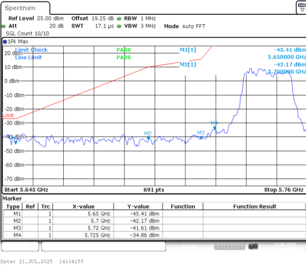
11N20MIMO-Ant1-5745-PASS
