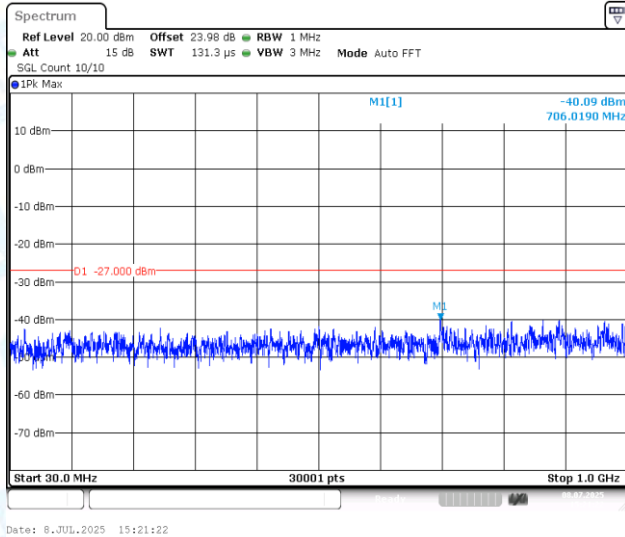
11AX20MIMO-Ant1-5200-30~1000-PASS
