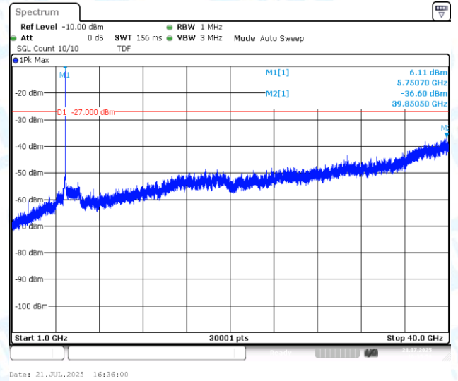
11AX20MIMO-Ant2-5745-1000~40000-PASS
